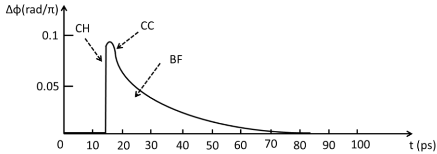
Fig. 2.2.9: Schematic diagram of phase evolution for a typical EAM following excitation by a single \sim 1 pJ pump pulse (pulsewidth \sim 100 fs).
