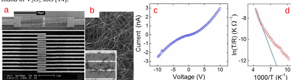
Fig. 1 (a) SEM images of IDEs fabricated by NIL with channel lengths of 100 nm. Scale bars = 10 \mu\text{m} (top) and 2 \mu\text{m} (bottom). (b) SEM image of the solution deposited VO x nanotube network (inset) the nanotubes spread across several metal fingers. (c) I-V curve of the VO x nanotube network on the interdigitated active area at room temperature. (d) Temperature dependence of the nanotube network resistance of the same sample area measured in (c).
