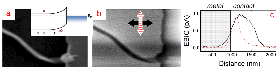
Fig. 3 (a) Secondary electron and (b) EBIC images of a single \text{VO}_x nanotube Schottky contact to a Au metal electrode. (Inset (a)) Band diagram where excess minority carriers diffuse to the space charge region and are swept to the contact by the internal electric field. (c) Line profiles of the data in (b) taken along (solid line/black arrow) and perpendicular (dashed line/dashed arrow) to the nanotube axis showing the signal decay.
