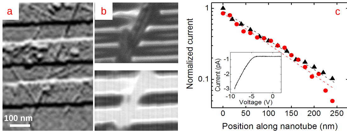
Fig. 2 (a) Non-contact AFM image of the solution-deposited VO x nanotubes on an IDE. (b) Secondary electron image (top) and corresponding EBIC image (bottom) of nanotube-channelled electrode fingers. The electrode spacing is 100 nm. (c) Semi-logarithmic EBIC line profiles from a Schottky contact at 5 kV for nanotube diameters of (●) 75 nm (▲) 200 nm. (Inset) I-V curve of the reverse bias nanotube-electrode contact.
