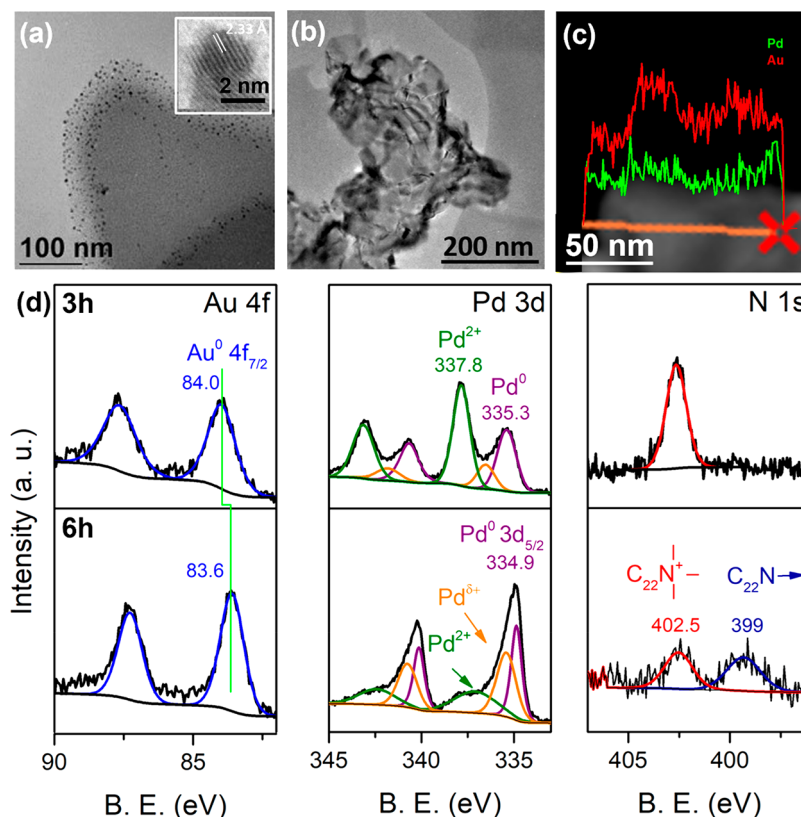
Figure 5. (a) TEM image 1 h after reaction showing NP formation. (b) TEM image from an incomplete reaction (3 h) showing formation of NSs. (c) EDX line map of NS after 3 h. (d) Au 4f, Pd 3d, and N 1s XPS core levels from incomplete and complete NS reactions.
