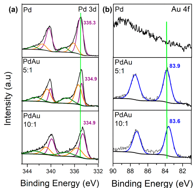
Figure 3. XPS analysis of (a) Pd 3d and (b) Au 4f core levels of Pd, PdAu 5:1 and 10:1 NS.
