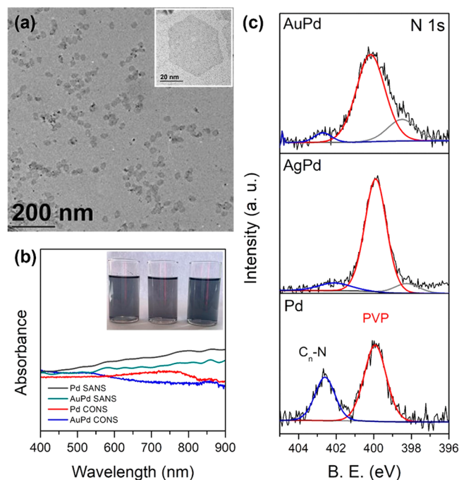
Figure 7. (a) Low-resolution TEM image. (b) UV-vis spectra of surfactant-assisted and CO-assisted NSs. (c) N 1s core level of Pd, PdAg and PdAu CO-assisted NSs.
