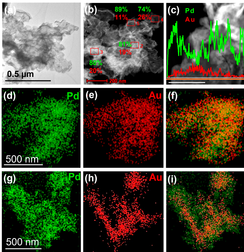
Figure 2. (a) TEM image of PdAu NSs 5:1. (b) STEM image and corresponding EDX quantification of atomic concentrations. (c) EDX line map of PdAu 5:1 NSs (scale bar is 100 nm). (d–f) Pd, Au, and overlaid EDX maps for PdAu 5:1. (g–i) Pd, Au, and overlaid EDX maps for PdAu 10:1 NSs.
