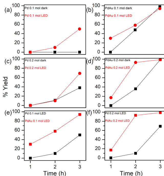
Figure 6. (a–f) Catalytic evaluation plots of the cross-coupling Suzuki reaction catalyzed using Pd and PdAu NSs at 0.1 and 0.2 mol % under visible light irradiation and in the dark.
