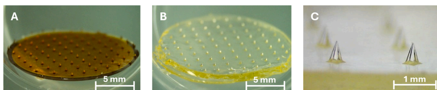
Fig. 13. Epoxy master (A) together with resulting PVP array (B), and a close up picture of two similarly prepared PVA microneedles (C).
