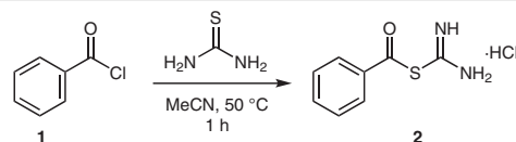
Scheme 1 Synthesis of S-benzoyl isothiurea hydrochloride ( 2 )
