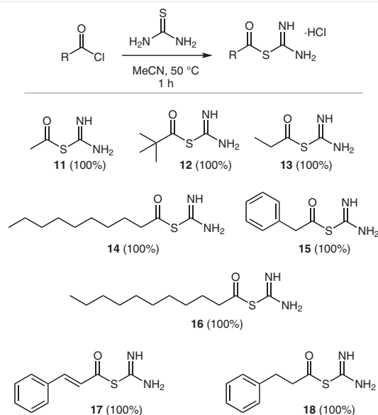
Scheme 3 Preparation of alkyl and aryl-alkyl derivatives 11–18 25
