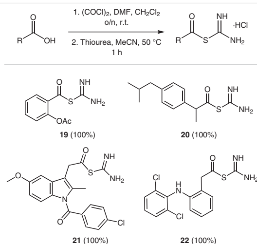
Scheme 4 Preparation of NSAID derivatives 19–22 25
