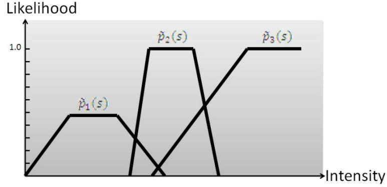
Figure 6.2: An explicitly probabilistic TF, where the material likelihood is defined using trapezoids in the familiar TF GUI interface.
