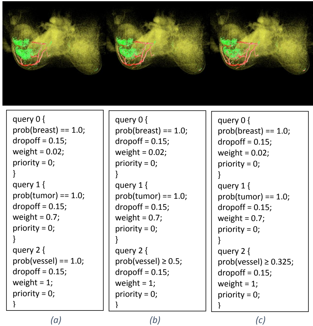
Figure 6.17: The Probabilistic Query uncertainty visualization applied to examine the correlations between the tumor and its surrounding vessels.
