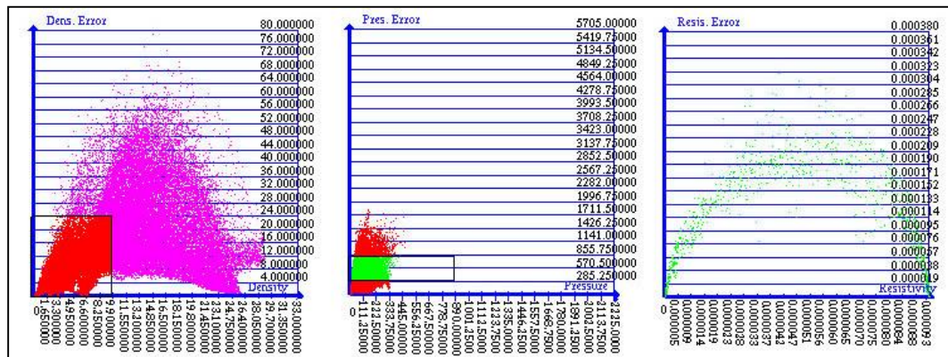
Figure 5.18: An example of a compound ROI specification.
