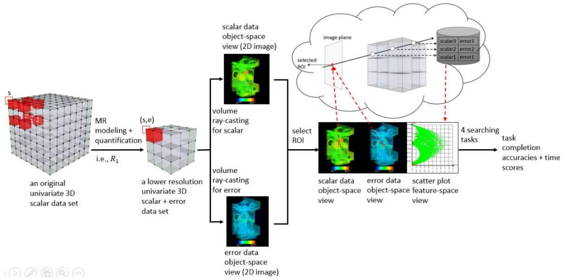
Figure 3.15: Workflow of LVIS uncertainty visualization technique.
