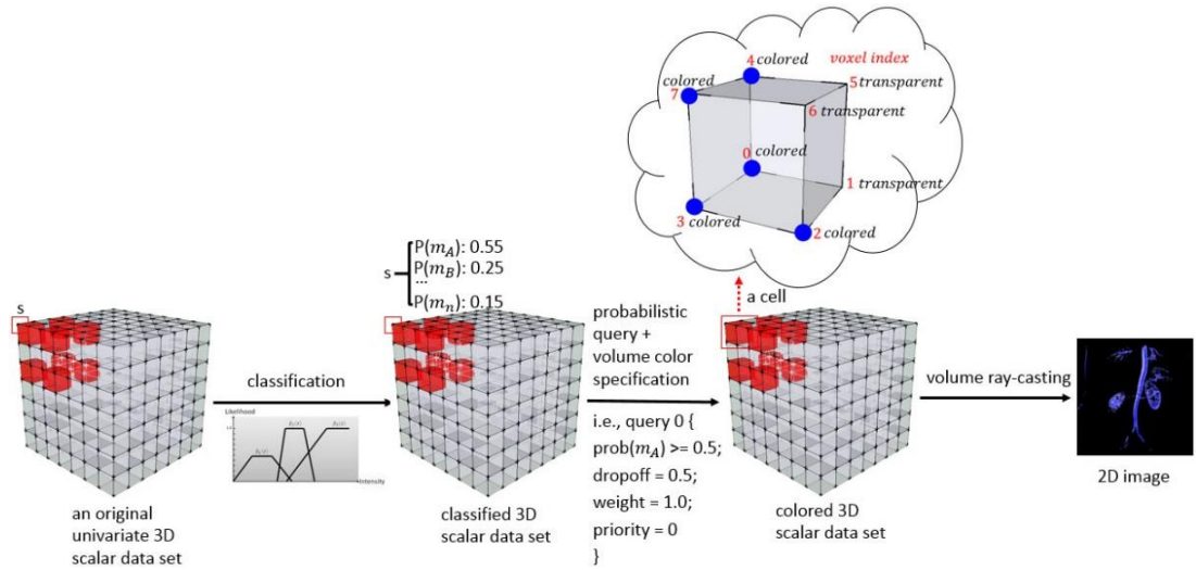
Figure 3.17: Workflow of Probabilistic Query uncertainty visualization technique.
