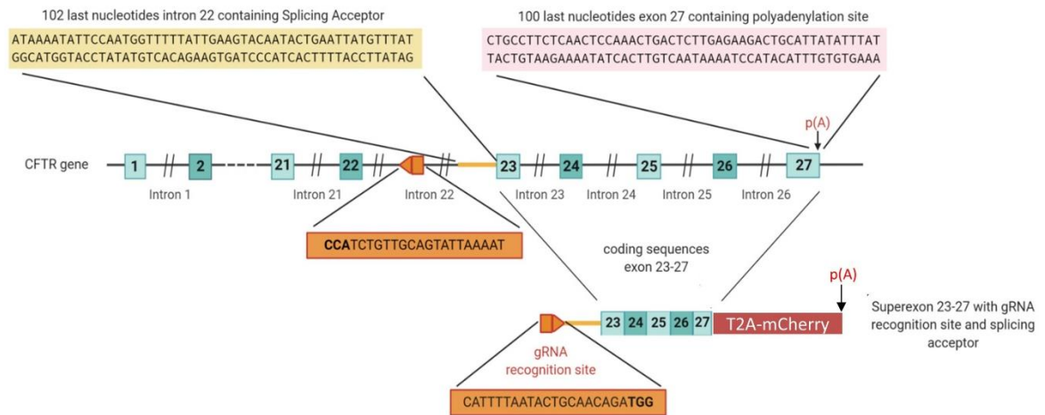
Figure 5.1: Graphical representation of the superexon version 1 design. The wild-type coding sequences of the exons 23 to 27 were fused together to form the superexon23-27. The 102 last nucleotides of the intron 22, containing the splicing acceptor, were added upstream of the superexon (in yellow). Before the splicing site, a gRNA recognition site was added, which was the same sequence as its homologous sequence in the genome, but in reverse-complementary orientation (in orange, with bold sequences being the PAM sites). The 100nt last nucleotides of the exon 27 were used as polyadenylation site (in pink).
