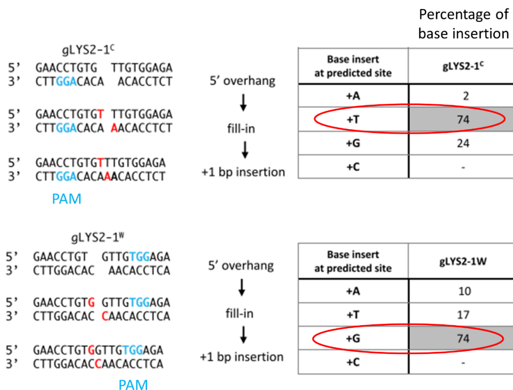
Figure 1.12: Pattern of insertion after Cas9 cutting and DSB repair. The left panel represents the expected insertion pattern if SpCas9 cut with one nucleotide 5' overhang, for two S. Cerevisiae genes. The right panel shows the percentage of base insertion observed after DSB repair. A correlation can be seen between the expected base insertion and the higher percentage of this expected base in the analyses (shown in the red circles). (Figure modified from Lemos et al. 2018; (96)).
