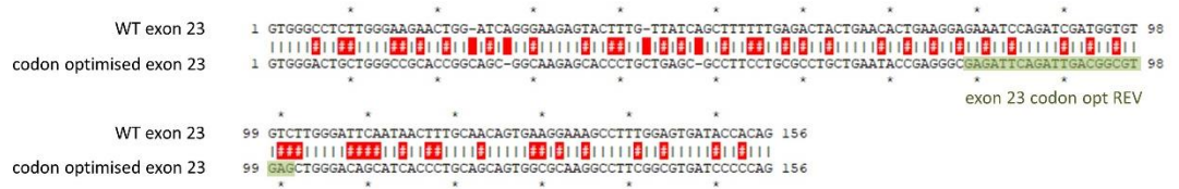
Figure 5.10: A) Graphic representation of SEv2, showing the CFTR cDNA sequence from exon 23 to exon 27, with a codon optimised exon 23 to differentiate from the endogenous CFTR before and after expression. Around the gRNA recognition site, a short, modified sequence of the intron 22 was added for NGS analysis (blue line). The DNA sequence on the top, represents the expected PCR amplicon sequence obtained after deep sequencing. Between the gRNA recognition site and the splicing acceptor, a 23nt reverse primer identical to a sequence in WT intron 22 was added (purple arrow and purple sequence). B) Graphic representation of the SEv2 integration into the CFTR gene at the 5' end, with the expected NGS PCR product sequence. C) Sequence alignment between the WT exon 23 and the codon optimised exon 23.
