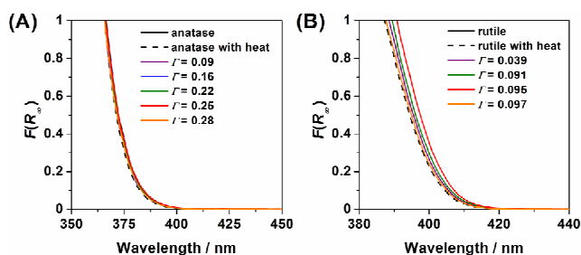
Figure 1. UV-Vis absorption spectra of (A) \text{SnO}_2/\text{anatase} and (B) \text{SnO}_2/\text{rutile} .
