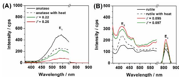
Figure 3. (A) PL spectra of \text{SnO}_2 /anatase at 77 K with an excitation wavelength of 320 nm. (B) PL spectra of \text{SnO}_2 /rutile measured under the same conditions.
