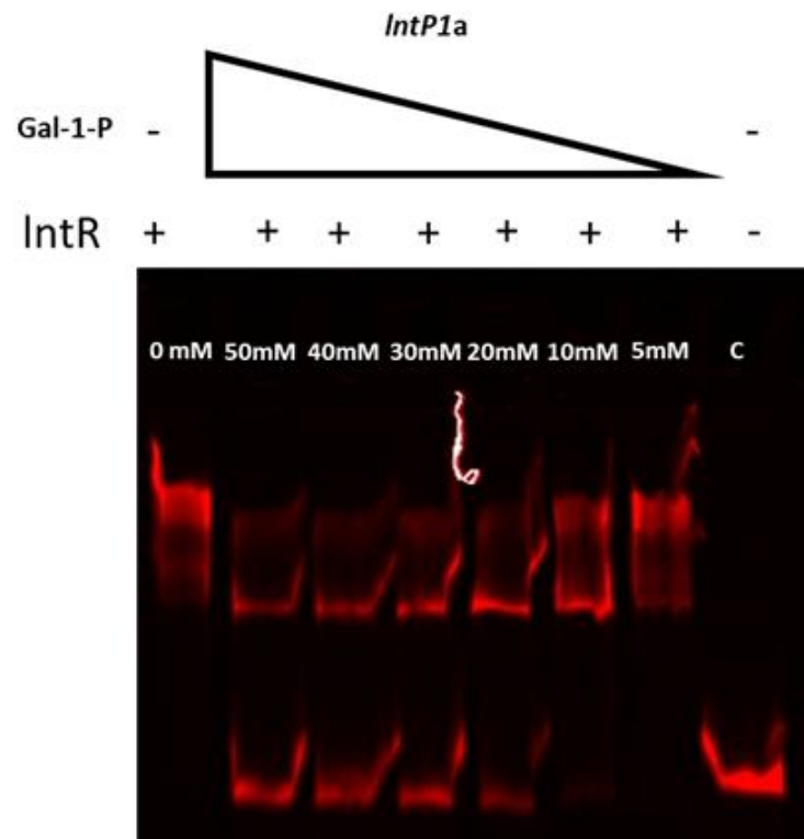
Supplemental Figure S3.3. EMSA images showing LntR interactions with promoter-containing DNA fragments, with the addition of a gradient (a) Gal-1-P and (b) Gal-6-P, ranging from 0mM-50mM. In each panel, ‘C’ indicates a negative control, where an equivalent amount crude cell extract from NZ9000 harbouring empty pNZ8150 was added instead of crude extract from the regulator-expressing NZ9000 strai
