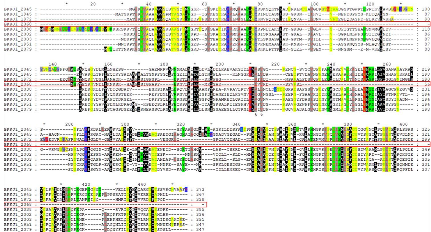
Supplemental Figure S5.1. Multiple sequence alignment of the amino acid sequences of the B. kashiwanohense APCKJ1 predicted truncated lacI-encoding gene galR (BKKJ1_2068; highlighted in red) and other predicted LacI-encoding genes in the APCKJ1 genome. A multiple sequence alignment was generated using the online resource Clustal Omega, with the default settings, and this alignment was visualised with Genedoc v 2.7.0, using physiochemical display mode (amino acids coloured based on shared physical and chemical properties). The alignment clearly shows a large proportion of the galR sequence missing when compared with the sequences of other LacI regulator-encoding genes.
