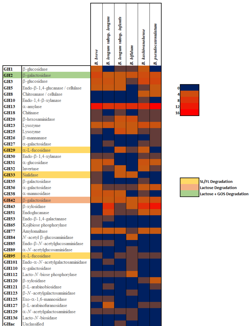
Figure 4.2. Heatmap representing the distribution of encoded glycosyl hydrolases, belonging to each GH family, across the genomes of B. breve UCC2003, B. longum subsp. longum NCC2705, B. longum subsp. infantis ATCC 15697, B. bifidum PRL2010, B. kashiwanohense JCM 15439 and B. pseudocatenulatum DSM 20438. A code colour grading is employed, which represents the number of glycosyl hydrolases of the same family encoded in each genome. Glycosyl hydrolase families which are known to function in the degradation of the HMO's 2-FL, 3-FL or 3-SL, lactose and/or GOS are indicated by shading.
