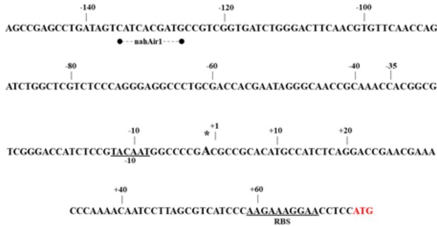
Supplemental Figure S3.1. Schematic representations (I) of the nahS (c) and nahA (d) promoter regions for the binding of NahR. Underlining indicates the 10 and 35 hexamers, and ribosome binding sites deduced from the primer extension results; experimentally determined transcriptional start sites (TSS) are indicated by asterisks. The dashed lines under sequences with names in boldface indicate the inverted-repeat nahSir1 and nahAir1 binding sequences displayed above the lollipops. The arrows in the right panels (II) indicate the primer extension products.
