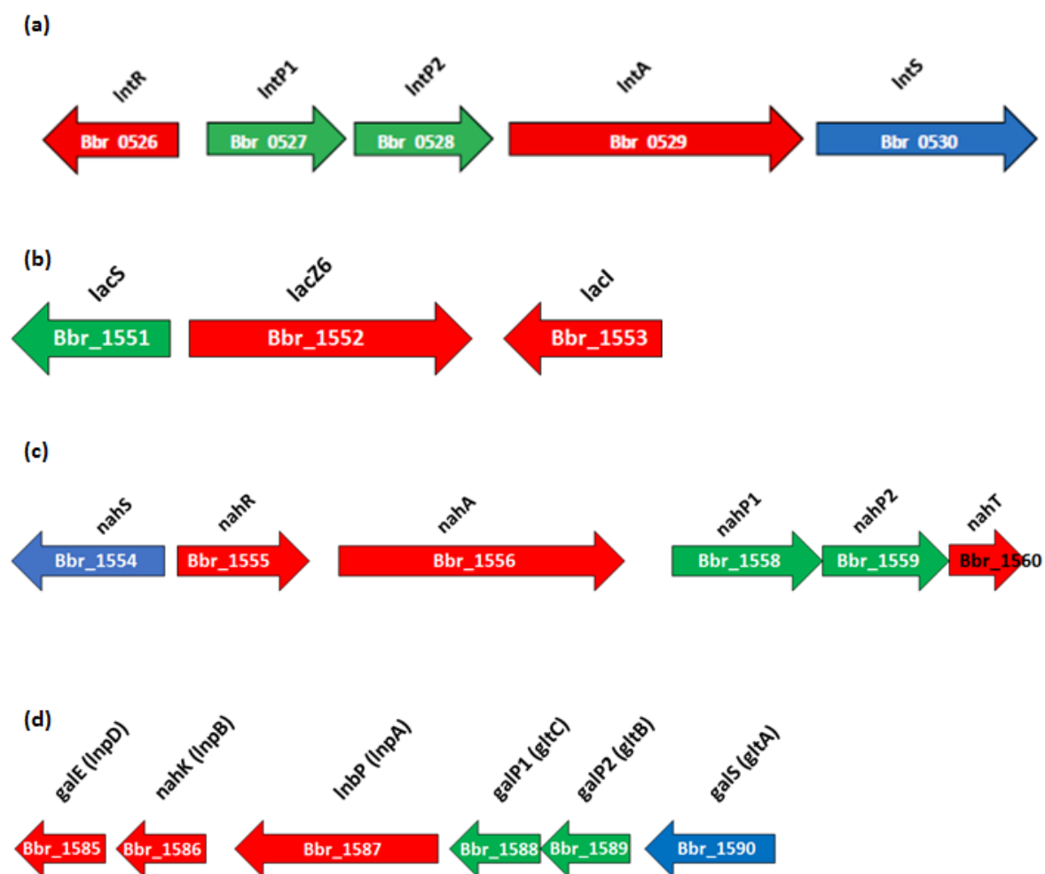
Figure 2.2. Schematic representation of the gene loci involved in the utilisation of LNT, LNnT and their substituents in B. breve UCC2003, as based on transcriptome analysis. The length of the arrows is proportional to the size of the open reading frame and the gene locus name, which is indicative of its putative function, is given at the top. Genes shown in red are predicted to encode proteins with an intracellular localisation, genes shown in green are predicted to encode proteins with a transmembrane localisation, and genes shown in blue are predicted to encode proteins with an extracellular localisation and a signal peptide sequence. The predicted function of each gene product is given in Table 2.1.
