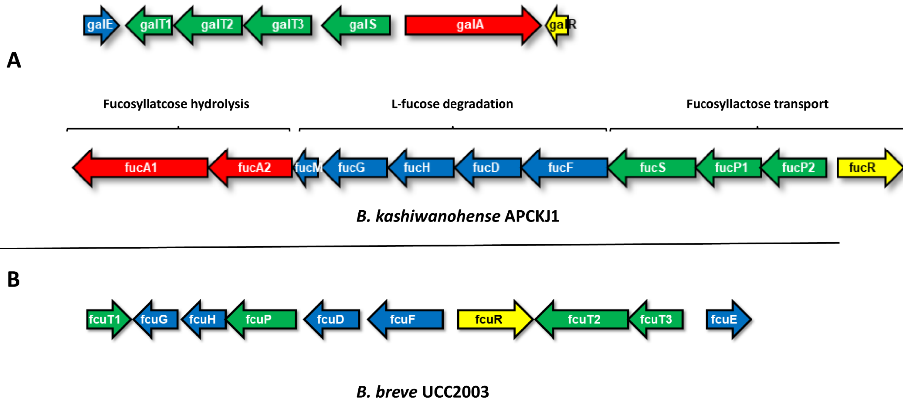
Figure 5.3. Schematic representation of the gene loci involved in the utilisation of: (A) 2-FL or 3-FL in B. kashiwanohense APCKJ1, and (B) L-fucose in B. breve UCC2003; as based on transcriptome analysis. The length of the arrows is proportional to the size of the open reading frame and the gene locus name, which is indicative of its putative function, is given inside the arrows. Genes shown in red are predicted to encode proteins with a hydrolytic function, genes shown in yellow are predicted to encode proteins with a regulatory function, genes shown in green are predicted to encode proteins with a transport function and genes shown in blue are predicted to encode proteins with another metabolic function.
