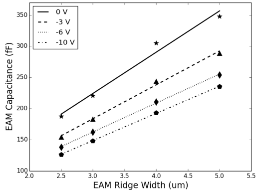
Fig. 4: EAM capacitance as a function of waveguide width for 200μm long EAMs.
