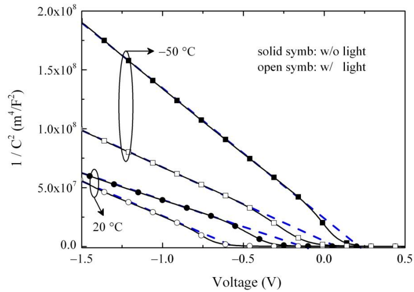
Fig. 5-9. 1/C^2 versus reverse bias voltage at 20 °C and -50 °C. Solid symbols: in dark; Open symbols: under illumination ( \lambda = 1.62 \mu\text{m} , P_{\text{opt}} = 10 \mu\text{W} ).
