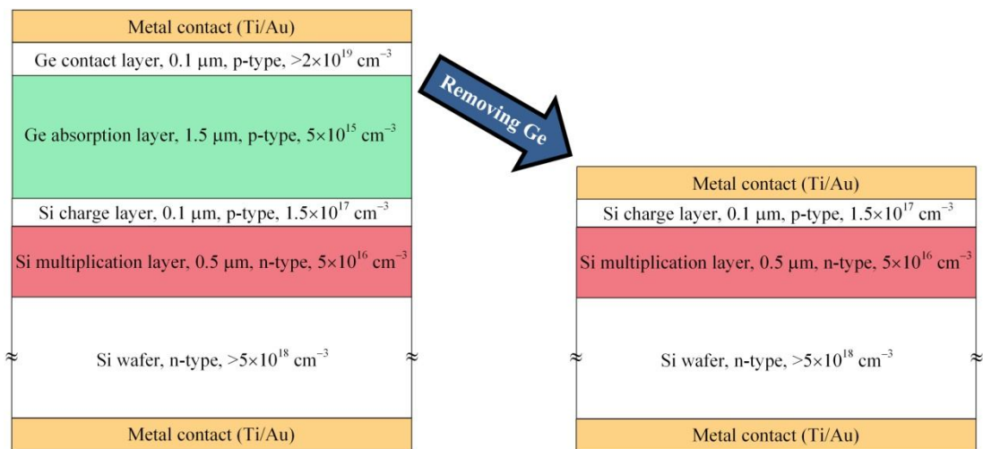
Fig. 3-19. Si devices were made from wafer number 8515 (Ge thickness: 1.5\text{ }\mu\text{m} ) by removing the germanium layer using wet etching.
