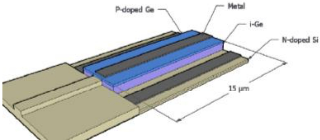
Fig. 1-17. Schematic view of pin germanium photodetector integrated in SOI waveguide. The photodetector length and width are 15 \mu\text{m} and 3 \mu\text{m} , respectively [45].
