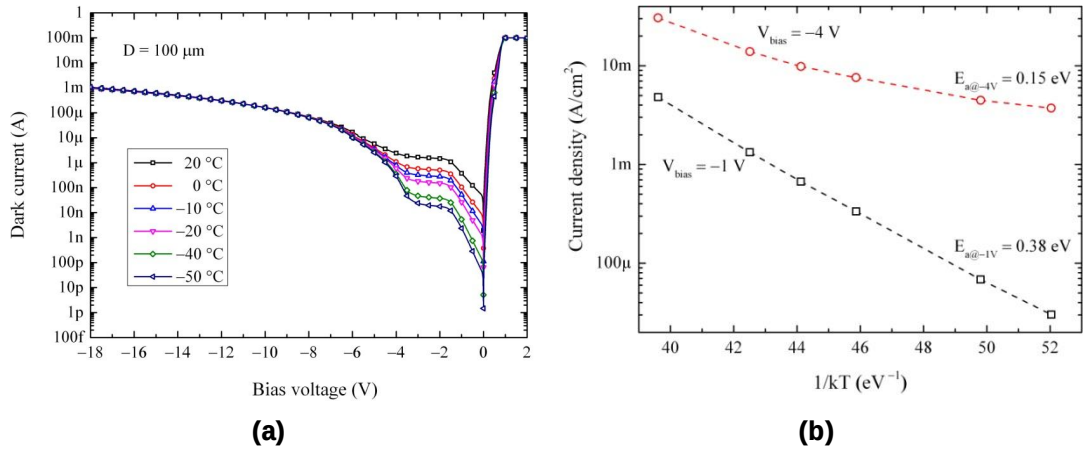
Fig. 3-14. (a) I - V characteristics of a 100 \mu\text{m} -diameter Ge/Si device from wafer number 8515 (Ge thickness: 1.5 \mu\text{m} ) at different temperatures in dark. (b) Current density versus 1/kT at -1 V and -4 V. The value of E_a at each bias voltage is also shown.
