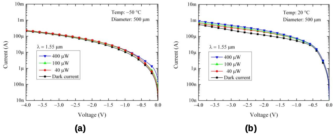
Fig. 5-12. I - V characteristics of the 500 \mu\text{m} -diameter Ge/Si photodetector in dark and under illumination ( \lambda = 1.55 \mu\text{m} ) at (a) -50^\circ\text{C} , and (b) 20^\circ\text{C} .
