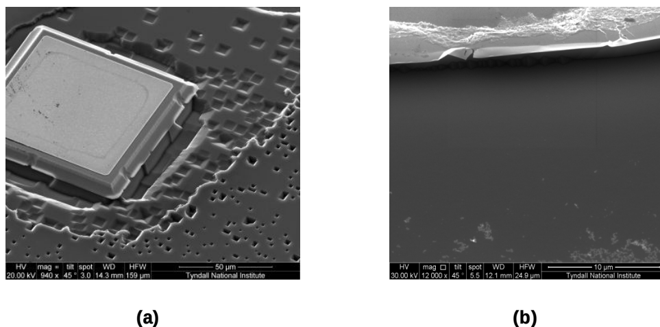
Fig. 3-21. SEM image of (a) Si sample designed for Ge/Si detector (wafer number 8515, Ge thickness: 1.5 \mu\text{m} ), and (b) Si sample (bulk, p-type), both after being etched using KOH.
