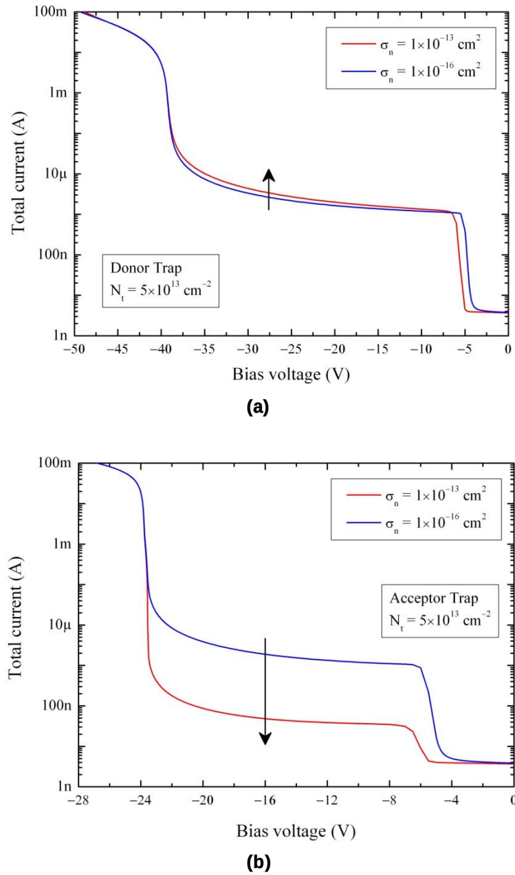
Fig. 2-15. Effects of electron capture cross sections on the total current for (a) donor type and (b) acceptor type traps. N_t = 5 \times 10^{13} \text{ cm}^{-2} for all cases.
