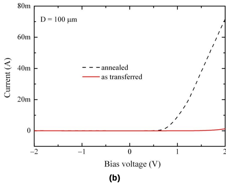
Fig. 4-2. (a) I – V characteristic of a 100 \mu\text{m} -diameter diode before and after annealing in log scale. (b) The I – V characteristic in linear scale. As shown in part (a), the ideality factor of the diode is 5.48 before an annealing and 2.28 after an annealing.
