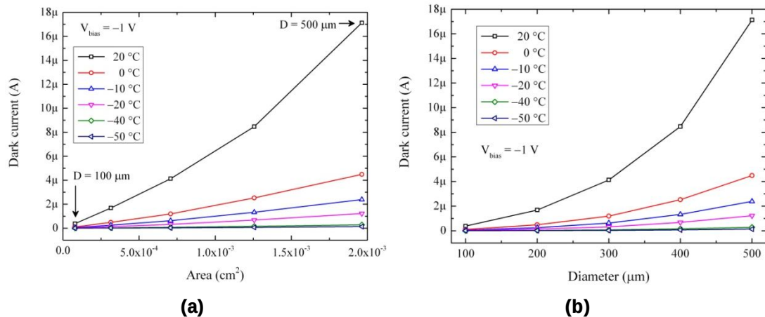
Fig. 3-15. Dark current of the Ge/Si devices versus (a) device area, and (b) device diameter at different temperatures. The Ge/Si devices were made using wafer number 8515 (Ge thickness: 1.5 \mu\text{m} ).
