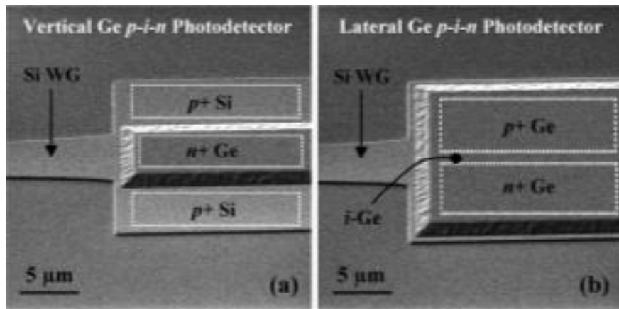
Fig. 1-4. (a) SEM micrograph showing an evanescent coupled Ge photodetector featuring vertical p-i-n configuration. The width W and length L of the detector is 8 and 100 \mu\text{m} , respectively. (b) Ge photodetector design with a lateral p-i-n configuration. The width W and length L of this detector is 20 and 100 \mu\text{m} , respectively [8].
