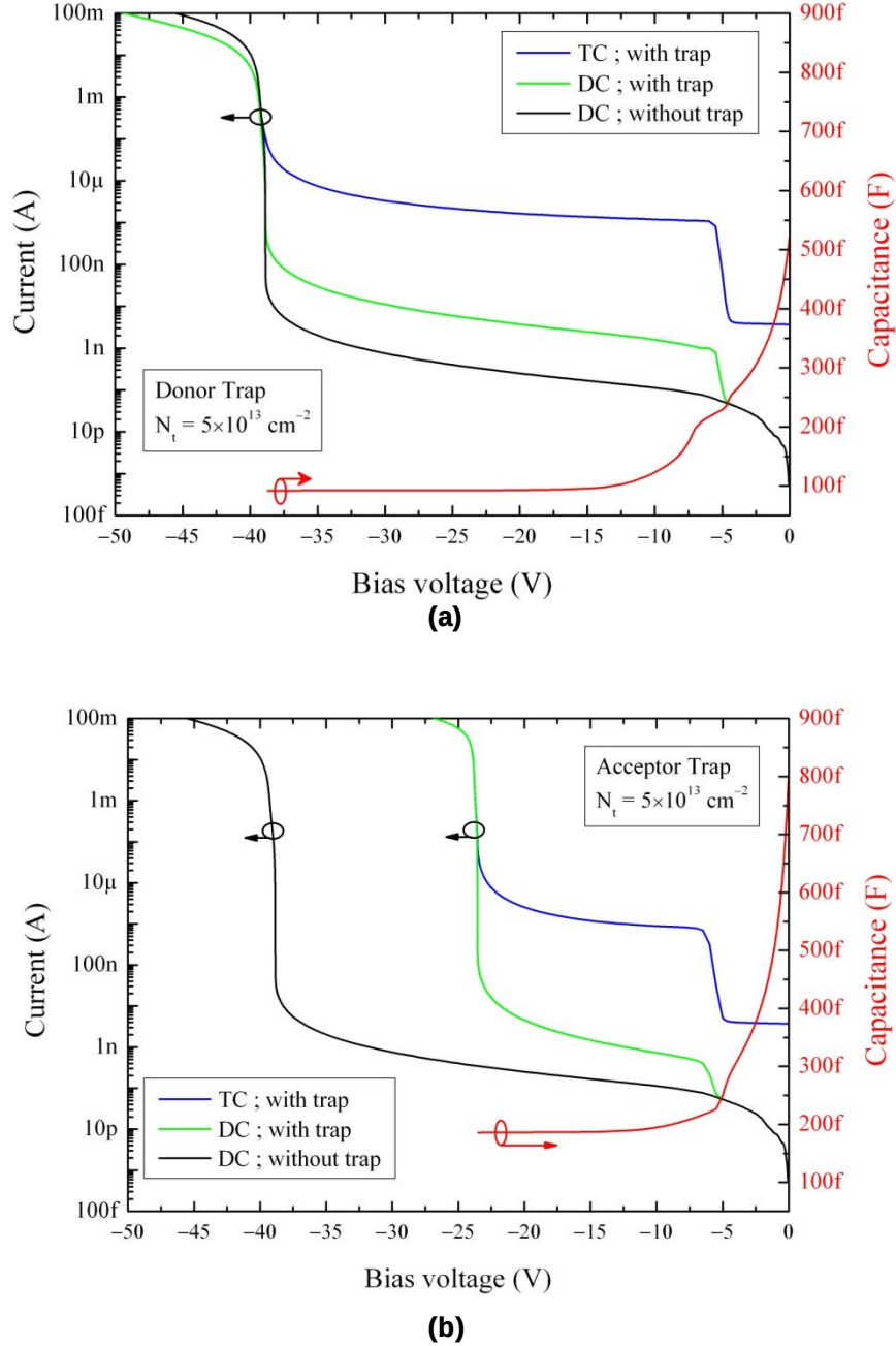
Fig. 2-12. I - V and C - V characteristics of Ge/Si APD with (a) donor traps ( N_t = 5 \times 10^{13} \text{ cm}^{-2} ), and (b) acceptor traps ( N_t = 5 \times 10^{13} \text{ cm}^{-2} ). Dark current of an ideal APD is also shown.
