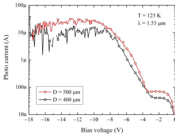
Fig. 3-18. Photo-current ( I_{TC} - I_{DC} ) of a 400 \mu\text{m} - and a 500 \mu\text{m} -diameter device at 125 K. The devices are made using wafer number 8515 (Ge thickness: 1.5 \mu\text{m} ).
