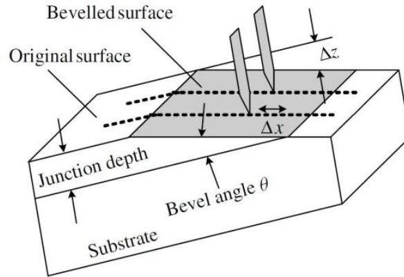
Fig. A2-1. Spreading resistance bevelled sample with probes - the probe path is shown by the dashed line.
