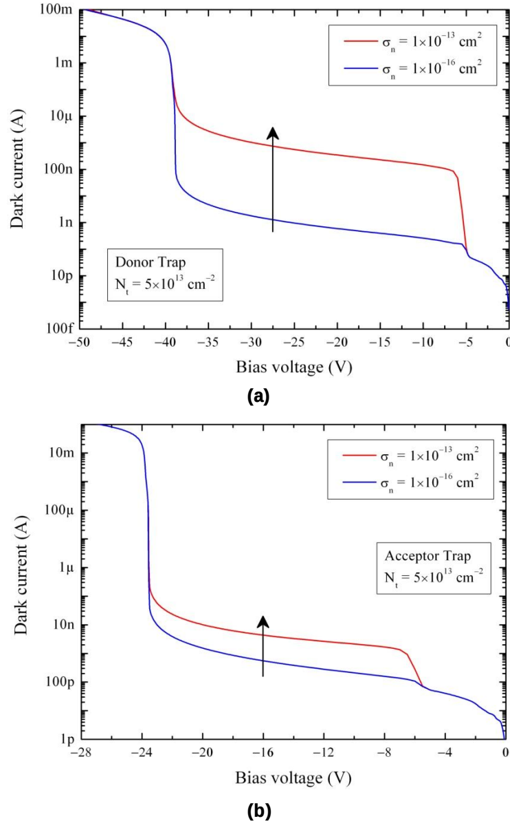
Fig. 2-14. Effects of electron capture cross sections on the dark current for (a) donor type and (b) acceptor type traps. N_t = 5 \times 10^{13} \text{ cm}^{-2} for all cases.
