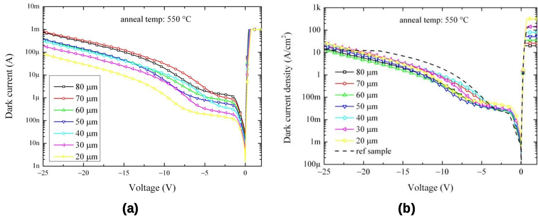
Fig. 3-22. (a) Dark current and (b) dark current density versus voltage of the annealed sample at 550 °C (wafer number: 8515, Ge thickness: 1.5 μm). In part (b), the dark current density of the reference sample (not annealed) is shown for comparison.
