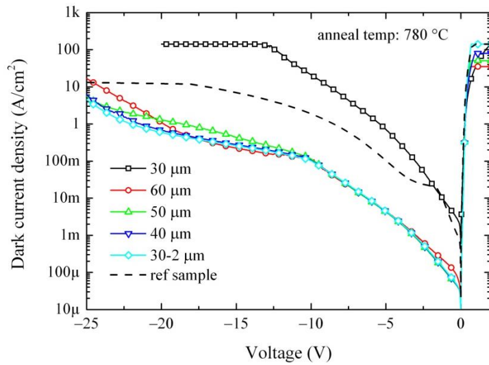
Fig. 3-23. Dark current density of the annealed sample at 780 °C for devices with different diameters (wafer number: 8515, Ge thickness: 1.5 μm). Comparing the results of the two 30 μm-diameter devices shows the non-uniform effect of the high temperature anneal. The characteristic of a reference sample (not annealed) is shown by dashed line.
