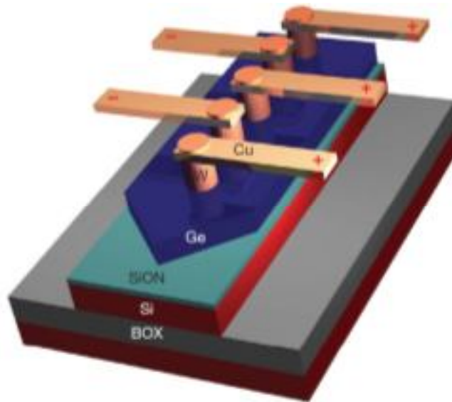
Fig. 1-20. Schematic of the nanophotonics Ge waveguide-integrated APD. The Ge layer is deposited on top of a SiON insulating layer which overlays a Si waveguide. The detector is biased through metallic interdigitated contacts consisting of W plugs and Cu wires [2].
