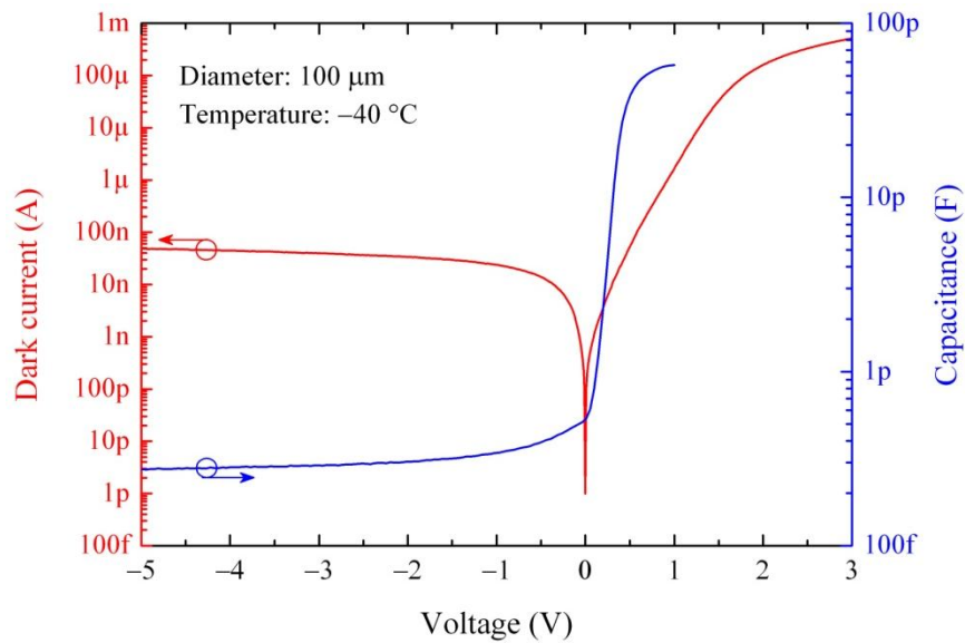
Fig. 5-18. I - V (left axis) and C - V (right axis) characteristics of a 100 μm-diameter device at -40 °C.
