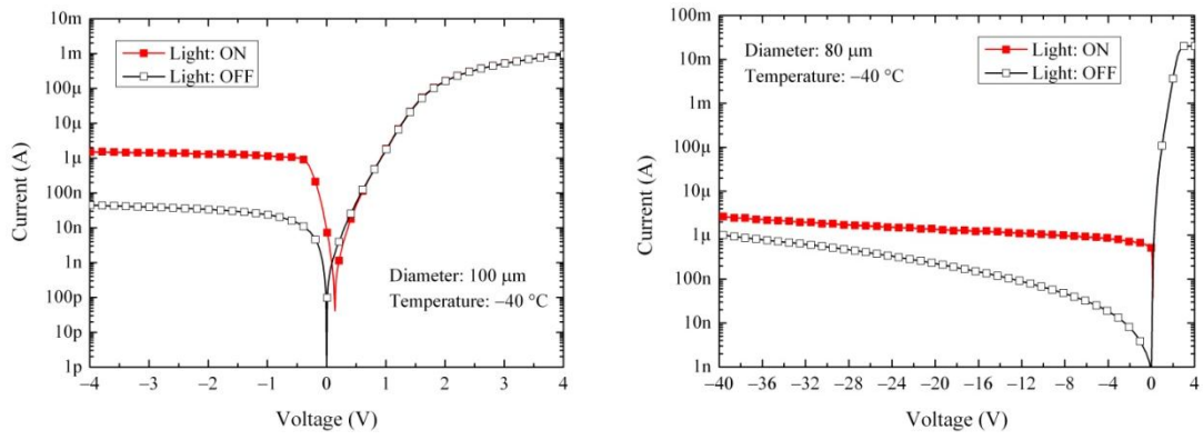
Fig. 5-17. Dark current and total current (under microscope white light illumination) of a 100 μm-diameter device (left) and an 80 μm-diameter device (right) for different bias voltage ranges.
