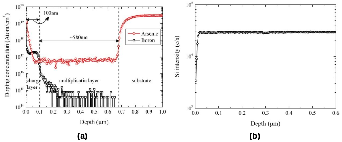
Fig. 3-8. (a) Arsenic and boron doping concentrations, and (b) Si intensity of different layers of UPSW. These results are obtained by SIMS measurement.
