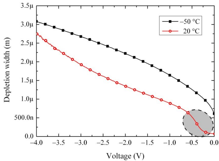
Fig. 5-10. Depletion width as a function of reverse bias voltage at 20 °C and -50 °C. The shaded region illustrates the effect of charges captured by the interface traps at 20 °C.
