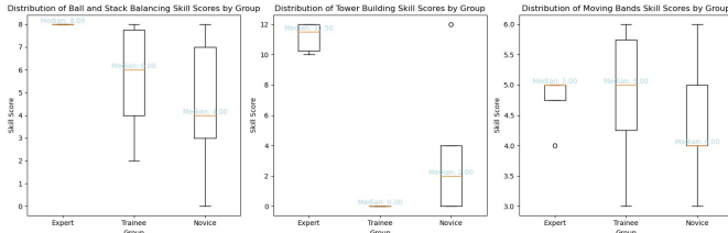
Fig. 2. Distribution of Performance for each skill
