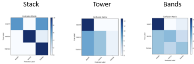
Fig. 5. Multi-class confusion matrices. Test accuracy of stack, tower, and bands is 79%, 49%, and 54%, respectively.
