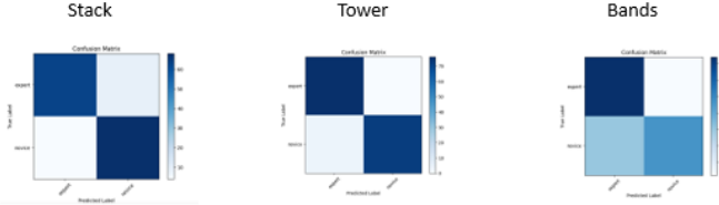
Fig. 6. Binary class confusion matrices. Test accuracy of stack, tower, and bands is 91%, 97%, and 79%, respectively.
