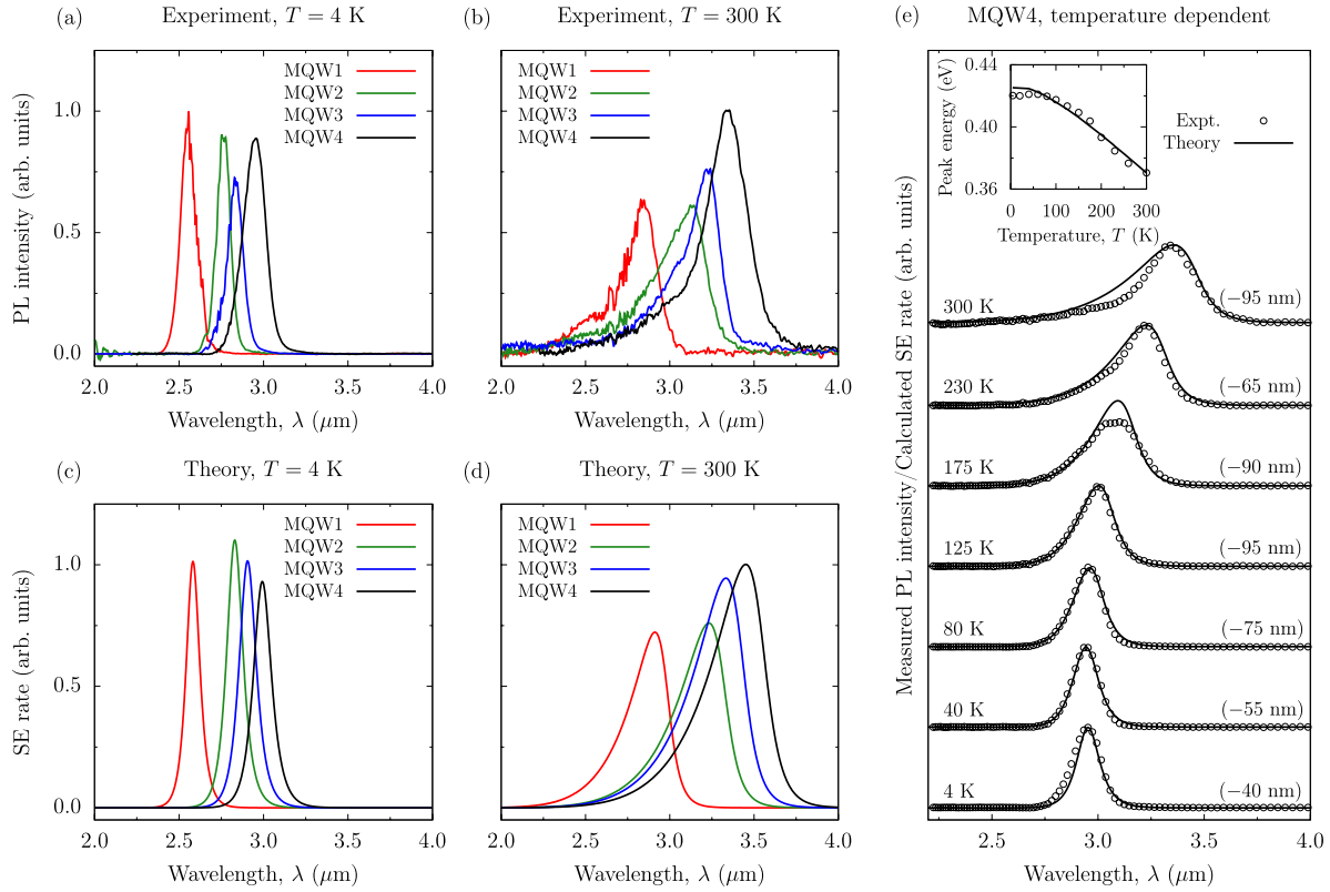
Figure 3. Measured PL spectra for structures MQW1–MQW4 (solid red, green, blue and black lines, respectively) at temperatures (a) T = 4 K, and (b) T = 300 K. The corresponding calculated SE spectra for structures MQW1–MQW4 at T = 4 and 300 K are shown respectively in (c) and (d). At each temperature the values of the measured PL and calculated SE have been normalised to that of the structure having the highest measured peak PL intensity (MQW1 at 4 K, and MQW4 at 300 K). The full temperature-dependent set of measured PL and calculated SE spectra for MQW4 are shown in (e) using, respectively, open circles and solid black lines. The calculated SE spectra in (e) have, at each temperature, been normalised in intensity (except at T = 175 K; see text) and shifted in wavelength (by the amount specified in parentheses) to match the experimental data at the PL peak. The open circles (solid black line) in the inset to (e) show the measured (calculated) variation of the PL (SE) peak energy with temperature in MQW4, where a rigid 11 meV redshift has been applied to the calculated SE peak energies to match the measured and calculated energy at T = 300 K.
