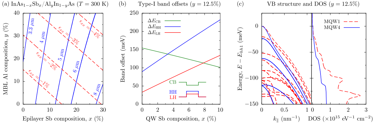
Figure 2. (a) Composition space map describing the ranges of in-plane strain ( \epsilon_{xx} ) and room temperature band gap (emission wavelength) accessible using bulk-like \text{InAs}_{1-x}\text{Sb}_x epitaxial layers grown on an \text{Al}_y\text{In}_{1-y}\text{As} MBL. Dashed red and solid blue lines respectively denote paths in the composition space along which \epsilon_{xx} and the band gap are constant. (b) Calculated variation of the CB, HH and LH type-I band offsets (solid green, blue and red lines, respectively) with Sb composition x , for compressively strained \text{InAs}_{1-x}\text{Sb}_x QWs grown on an \text{Al}_{0.125}\text{In}_{0.875}\text{As} MBL. (c) Calculated VB structure (left panel) and DOS (right panel) for structures MQW1 (dashed red lines) and MQW4 (solid blue lines) of table 1. For each structure the zero of energy has been set at the QW VB edge—i.e. at the energy of the highest energy valence subband hh1 , which is purely HH-like at k_{||} = 0 .
