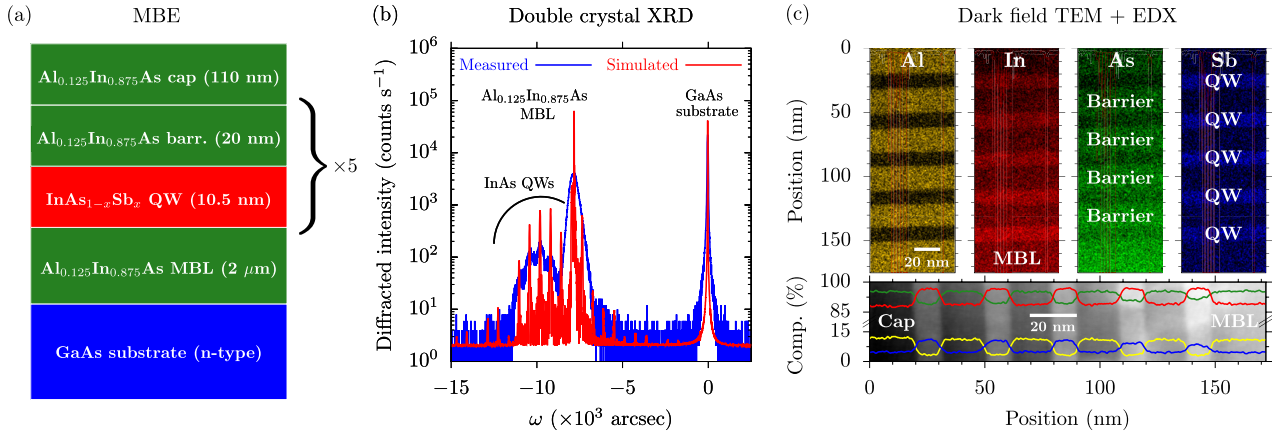
Figure 1. (a) Schematic illustration of the metamorphic multi-QW structures investigated in this work: the structures consist of compressively strained \text{InAs}_{1-x}\text{Sb}_x QWs grown between unstrained \text{Al}_{0.125}\text{In}_{0.875}\text{As} barriers, with growth on GaAs facilitated via the use of an \text{Al}_{0.125}\text{In}_{0.875}\text{As} MBL. (b) DC-XRD spectrum for MQW1, measured (solid blue line) and simulated (solid red line) about the GaAs (004) reflection. (c) Upper panels: false-colour dark-field TEM images for MQW4, where the intensity of the yellow, red, green and blue colouration respectively describes the Al, In, As and Sb compositions in the QW and barrier layers. Lower panel: solid yellow, red, green and blue lines respectively denote the variation of the Al, In, As and Sb compositions along the (001) growth direction for MQW4, as inferred from EDX measurements. For illustrative purposes, the EDX data have been superimposed onto a dark-field TEM image of the structure.
