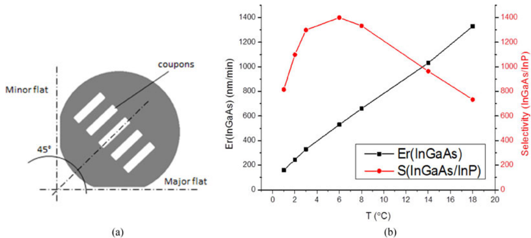
Fig. 5. Coupon arrangement with respect to the crystal planes of the wafer (a); the \langle 010 \rangle and \langle 001 \rangle crystal planes are at 45^{\circ} to the major axis. Etch-rate of \text{FeCl}_3:\text{H}_2\text{O} (1:2) for InGaAs along \langle 010 \rangle and \langle 001 \rangle planes and the related selectivity to InP for bath temperatures in the range 1–18 ^{\circ}\text{C} (b).
