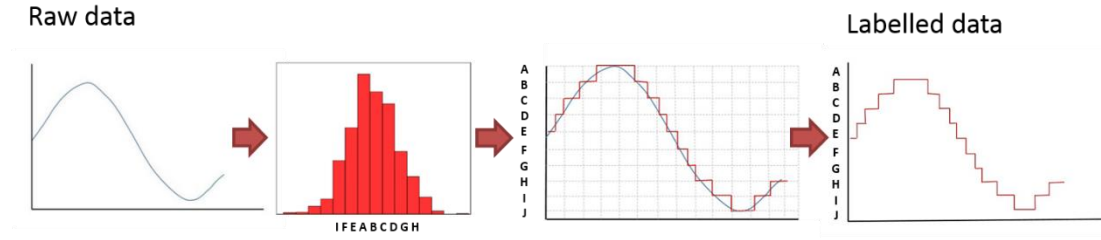
Figure 3.6: Schematic representation of the signal labelling using histogram binning.
