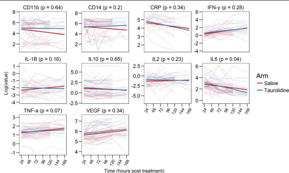
Fig. 2 Seven-day linear trends in laboratory endpoints. Differences in the 7-day linear trend between treatment arms were tested using linear mixed effects models and treatment X time interaction term. The p -values in the plot are from the likelihood ratio test for a model including that interaction term vs. a model without it
