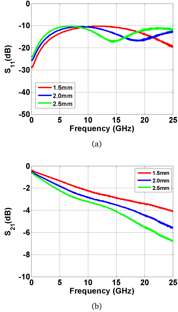
Figure 5.8: Measured Electrical S-parameters for devices with different electrode length: (a) S_{11} . (b) S_{21} .
