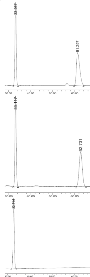
Figure 5. Chiral HPLC trace for ( \pm )-1b, top; ( \pm )-2b, middle; and ( S )-2b, bottom. For ( \pm )-2b and ( S )-2b, the data is obtained using the individual crystal from the single crystal analysis.
