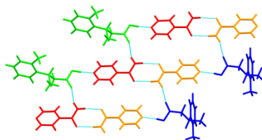
Figure 4. Hydrogen bond motif in ( S )-2b. The same color scheme is applied as for Figure 1.
