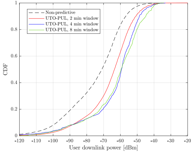
Fig. 4: CDF of user receive power for different prediction windows
