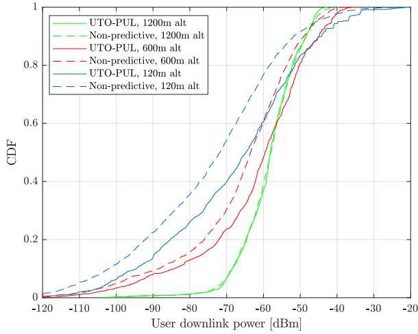
Fig. 5: CDF of user receive power for different UAV altitudes
