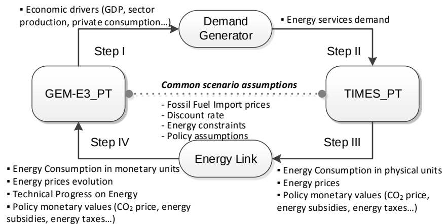
Figure 5.2 HYBTEP soft-linking methodology (Fortes et al., 2014)
