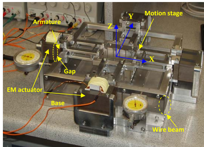
Figure 1. A desktop-size XY compliant parallel manipulator actuated by two EM actuators (where the twisting rotation about the Z-axis is well constrained by appropriately setting up the ratio of the motion stage size to the wire beam length and making beams distribute around multiple circles).
