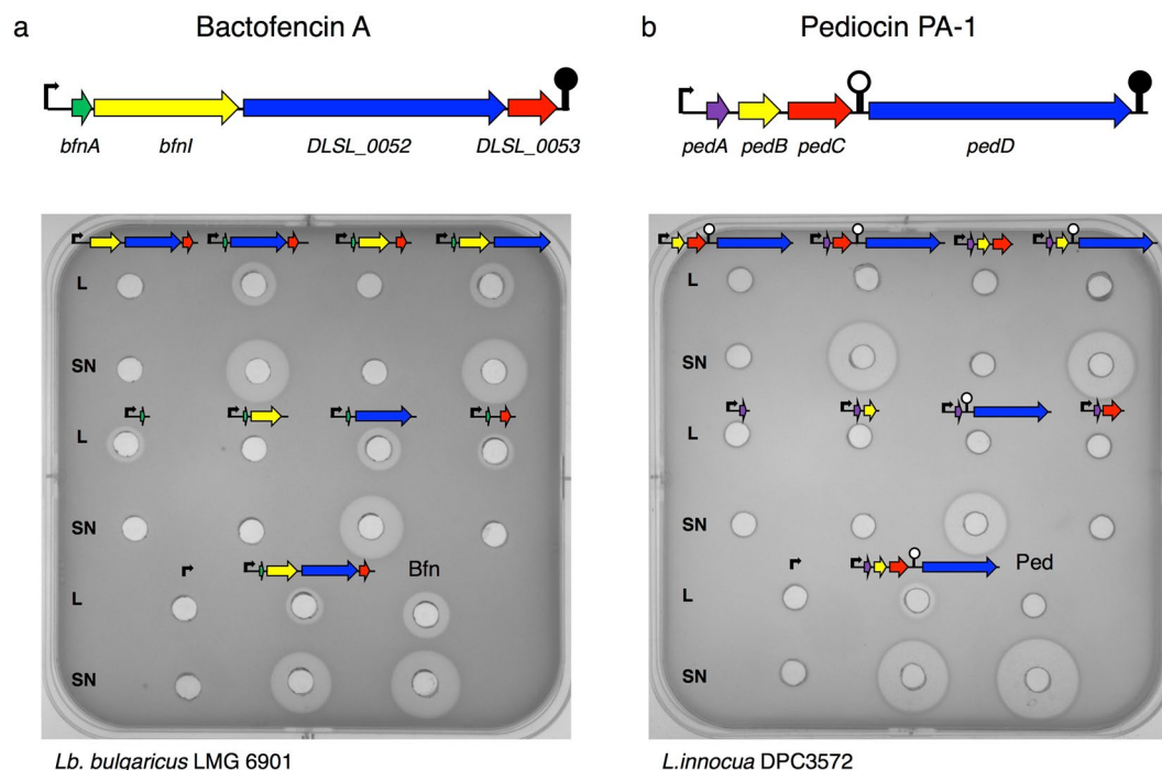
Figure 3. Antimicrobial activity of cell-free supernatants (SN) and lysates (L) of E. coli Tuner™ (DE3) after 3 hours of 25 \mu M IPTG induction. (a) Analysis of bactofencin A activity against Lb. bulgaricus and (b) pediocin PA-1 activity against L. innocua . The genes that encode the structural peptide of bactofencin and pediocin are indicated in green and purple arrows, respectively. The immunity, the transporter and the accessory protein encoded genes are shown in yellow, blue and red arrows. The black arrow indicates the T7lac promoter. Samples from the natural producers Lb. salivarius DPC6502 and P. acidilactici LMG2351 are indicated as Bfn and Ped.
