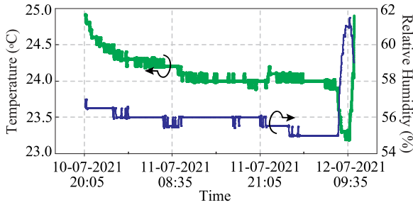
Fig. 5. Measured temperature and humidity results.
