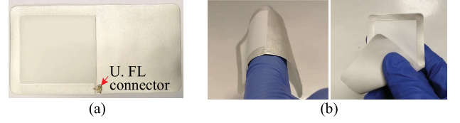
Fig. 2. (a) Screen-printed antenna prototype upon U. FL connector assembly. (b) Antenna under deformation demonstrating its flexibility.
