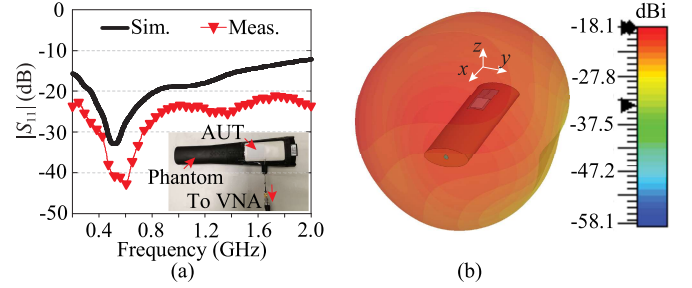
Fig. 3. (a) Measured and simulated |S_{11}| when the antenna attached on the phantom as illustrated in the inset. (b) Simulated 3D radiation pattern of the antenna at 868 MHz.
