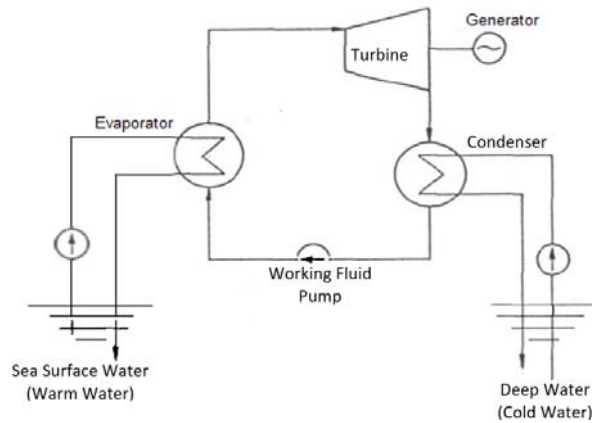
Figure 2. OTEC Closed Cycle schematic [7]
