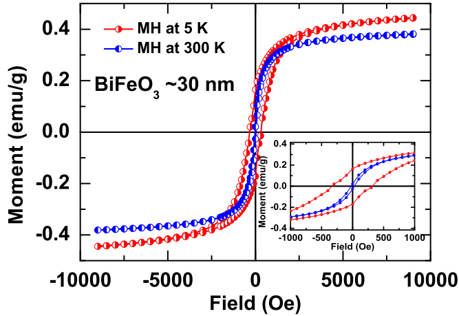
FIG. 4. (Color online) Magnetic hysteresis loop showing the soft ferromagnetic behavior of nanoscale \text{BiFeO}_3 ; the portion of the loop near origin is blown up in the inset to demonstrate absence of any exchange bias whatsoever, thus proving the sample to be free from any magnetic impurity.
