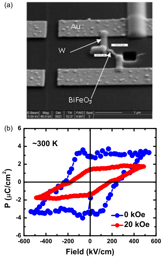
FIG. 5. (Color online) (a) Scanning electron microscopy image of the patterned nanochain of \text{BiFeO}_3 and (b) the remanent hysteresis loop measured at room temperature under zero and \sim 20 kOe magnetic field.
