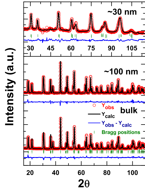
FIG. 1. (Color online) Powder neutron diffraction data and their refinement by FullProf for samples of different particle sizes; while the wavelength corresponding to the topmost pattern is 2.417 Å, it is 1.480 Å for the other patterns.
