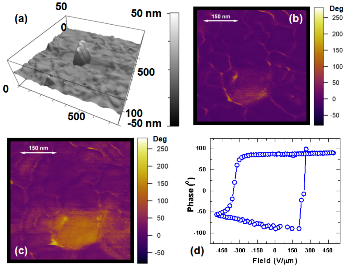
FIG. 3. (Color online) (a) AFM and phase contrast PFM images under (b) zero field and (c) poling under 10 V of an isolated nanoparticle of BiFeO 3 in vertical scan; poling leads to a change in color from purple to yellow because of \sim 90^\circ switching of polar domain; the polarization is oriented vertically after poling; (d) the complete phase evolution hysteresis loops from switching spectroscopy PFM measurement.
