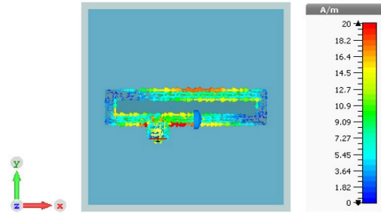
FIGURE 3. Surface current distribution at 2.38 GHz.
