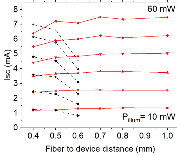
FIGURE 3.15: Variation of I_{sc} of Chip 2 as a function of fiber-to-device distance for incident optical powers ranging from 10 mW to 60 mW. The I_{sc} values under annular beam illumination are shown in black (dashed trace), while those under quasi-Gaussian illumination are shown in red (solid trace).
