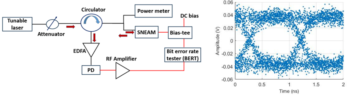
FIGURE 4.15: (a) Schematic of Eye diagram measurement and (b) The SNEAM device modulated with NRZ-OOK signal at 1 Gbps.
