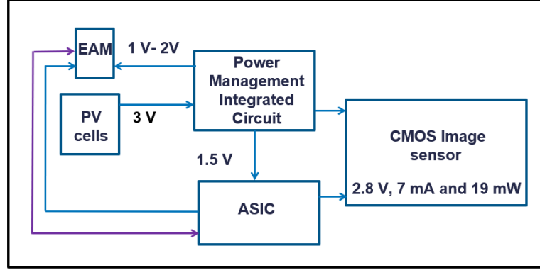
FIGURE 5.4: Block diagram illustrating the voltage distribution through the power management integrated circuit (PMIC) to the various system components, highlighting the supply requirements of the customized CMOS image sensor.
