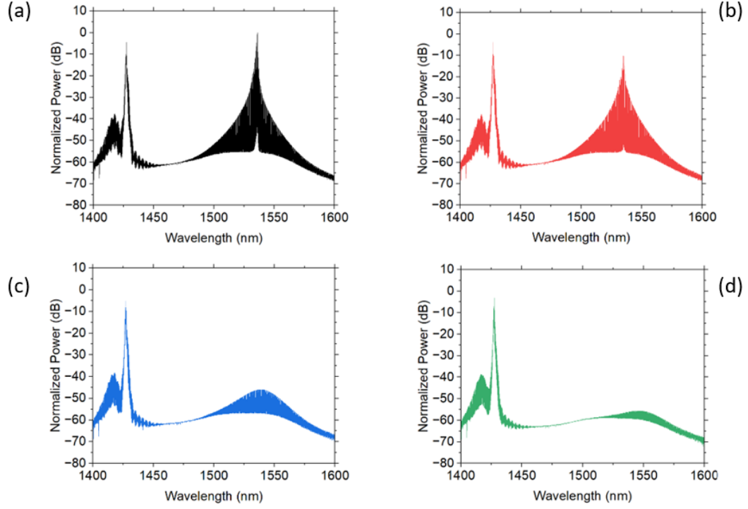
FIGURE 2.7: Emission spectrum of receiver laser near 1540 nm under zero bias and reverse bias condition with optically pumped by 1427 nm (a) 0 mA (b) -10 mA (c) -20 mA and (d) -30 mA.
