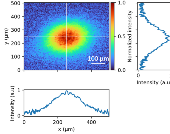
FIGURE 3.5: One-dimensional line scans along the x and y direction through the center of the quasi-Gaussian beam recorded on a diffusive imaging surface at a fiber to imaging plane distance of 600 \mu\text{m} . The profiles show a centrally peaked, Gaussian-like intensity distribution with superimposed fluctuations arising from multimode speckle.
