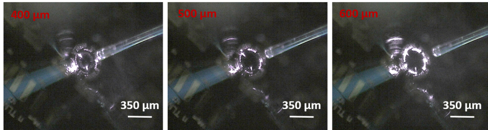
FIGURE 3.14: Annular beam illumination on the four segment GaAs PPC device captured at a 45 degrees angle for fiber to device distances of 0.4 mm, 0.5 mm, and 0.6 mm (images shown from left to right).
