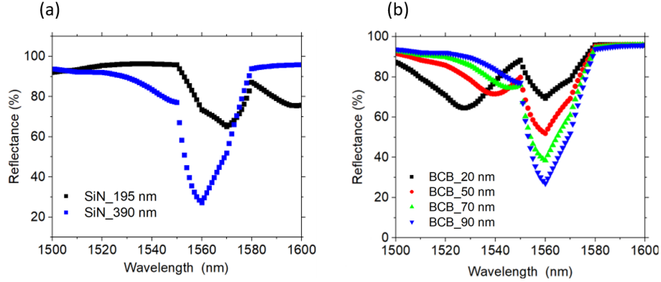
FIGURE 4.4: Thin-film simulation results of the multilayer PIN-BCB-SiN-Au structure obtained using Essential Macleod. (a) Reflectance spectra showing the variation in reflectance minimum for quarter-wavelength (195 nm) and half-wavelength (390 nm) SiN thicknesses at a fixed BCB thickness of 90 nm, highlighting the resonance near 1560 nm. (b) Spectral reflectance as a function of wavelength for different BCB thicknesses with the SiN thickness fixed at 390 nm.
