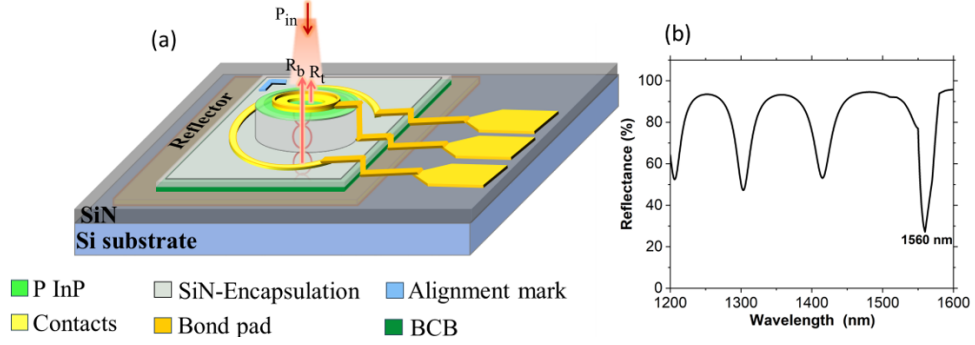
FIGURE 4.3: (a) Schematic of asymmetric FP resonance in the SNEAM device, (b) The simulated cavity response plotted for comparing reflection intensity with increase in reverse bias.
