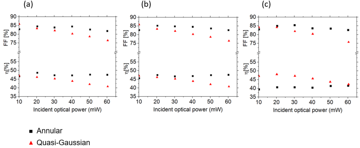
FIGURE 3.10: Variation of power conversion efficiency \eta and FF with incident optical power for the four segment PPC under annular and quasi-Gaussian illumination at fiber to device separations of (a) 400 \mu\text{m} , (b) 500 \mu\text{m} and (c) 600 \mu\text{m} .
