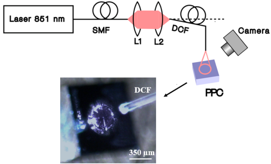
FIGURE 3.4: Experimental setup for annular beam illumination on the PPC. SMF; Single mode fiber coupled laser, L1 collimator focal length= 18.4 mm, L2 Biconvex lens focal length= 25 mm, DCF; double clad fiber (DCF-13 Thorlabs). The inserted picture shows diced chip under annular illumination at a fiber to device distance of 600 \mu\text{m} , recorded using a Dino-Eye Edge digital microscope (AM4025X model).
