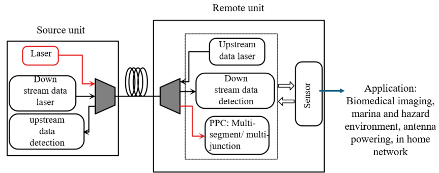
FIGURE 1.2: Schematic illustration of the POF system.
