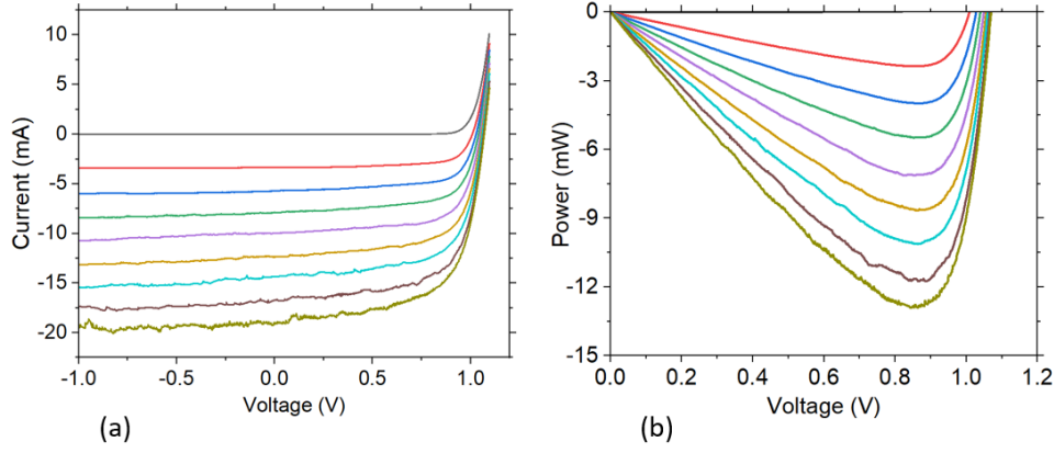
FIGURE 2.12: (a) I–V and (b) P–V characteristics of the 1060 nm waveguide laser operating as a PPC under different levels of incident optical power. The curves show the transition from dark to illuminated conditions, with photocurrent and output electrical power increasing proportionally with optical intensity. The curves are colour-coded from black (top) to olive-green (bottom), corresponding to incident optical powers ranging from 0 to 74 mW, obtained from pump power steps of 10 mW after normalization.
