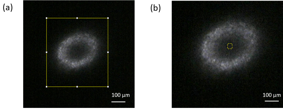
FIGURE 5.3: Power ratios calculated from raw annular beam images using background corrected integrated intensities extracted in ImageJ for a 350 \mu\text{m} diameter annular beam on a diffuse target. The highlighted rectangle indicates (a) the annular beam and background region and (b) 30 \mu\text{m} wide region used to estimate the fraction of optical power present at the beam center.
