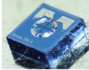
FIGURE 3.2: (a) Picture of 1 mm \times 1 mm chip with four segments laterally interconnected PPC with active diameter of 350 \mu\text{m} .
