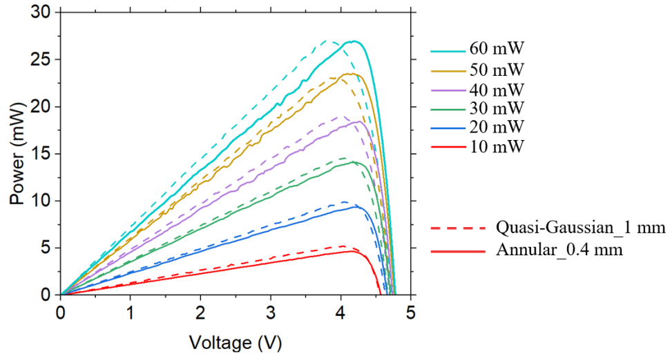
FIGURE 3.17: PV characteristics of the four-segment, 350 \mu\text{m} active diameter PPC, measured at the fiber-to-device separations corresponding to maximum power extraction for each illumination profile. Solid lines correspond to annular illumination at a distance of 0.4 mm, while dashed lines represent quasi-Gaussian illumination at a distance of 1 mm. Curve colour denotes the incident optical power, varied from 10 to 60 mW (bottom to top curve).
