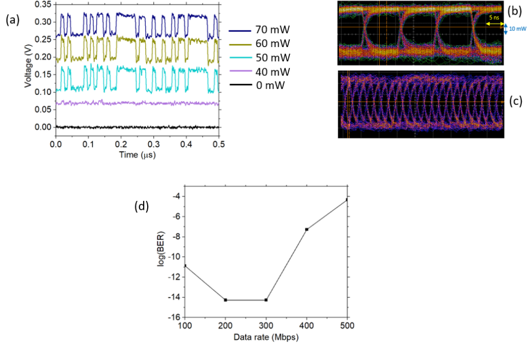
FIGURE 2.10: Data transmission from the receiver laser. (a) Detected 100 Mbps modulated signals from the receiver laser under varying absorbed optical powers, showing modulation onset above 40 mW. Eye diagrams of the received signal at varying data rates, illustrating the transition from a wide-open eye at lower bit rates (b) 100 Mbps and partially closed eye at higher bit rates (c) 500 Mbps. (d) Bit error rate (BER) plotted as a function of data rate, showing stable data transmission 200 Mbps to 300 Mbps.
