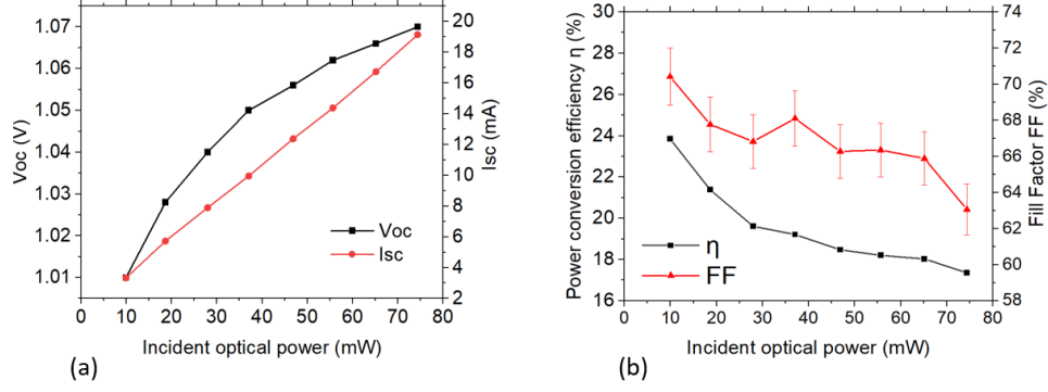
FIGURE 2.13: (a) Variation of of the 1060 nm single-junction PPC with incident optical power. (a) V_{oc} and I_{sc} showing a steady increase with illumination. (b) \eta and FF, with peak values of 23% and 70% at 10 mW, respectively. FF error bars denote the propagated I–V uncertainty used in the FF extraction, assuming 1.5% current and 0.5% voltage uncertainty, corresponding to a relative FF uncertainty of 2.24%. The slight FF increase near 40 mW lies within this uncertainty and is attributed to coupling fluctuations.
