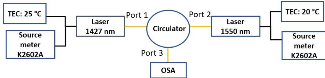
FIGURE 2.6: Schematic of the receiver laser PPC setup used to characterize lasing behavior under optical pumping through an optical circulator. Black lines indicate electrical connections, and yellow lines represent SM optical fibers.
