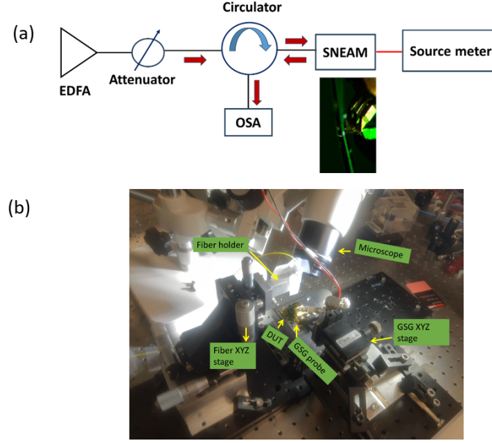
FIGURE 4.9: (a) Schematic of reflection experimental setup for the SNEAM device. The inset shows the fibre aligned device during testing. (b) Experimental setup showing a single-mode fiber aligned surface normal to the top surface of the device under test (DUT), which is probed using a GSG probe.
