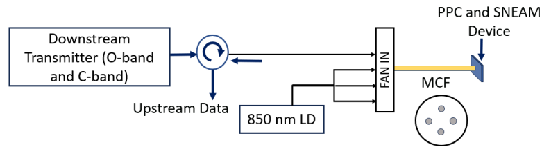
FIGURE 5.6: Schematic of experimental design on MCF as single fiber solution on illumination of PPC and bidirectional single transmission.
