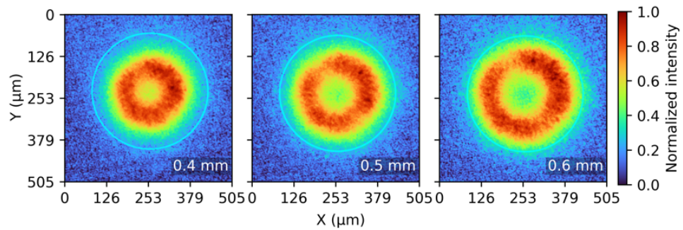
FIGURE 3.12: Annular beam intensity distributions overlapped with a 350 \mu\text{m} circular disk representing the PPC active region, plotted for fiber-to-device distances ranging from 0.4 mm, 0.5 mm and 0.6 mm.
