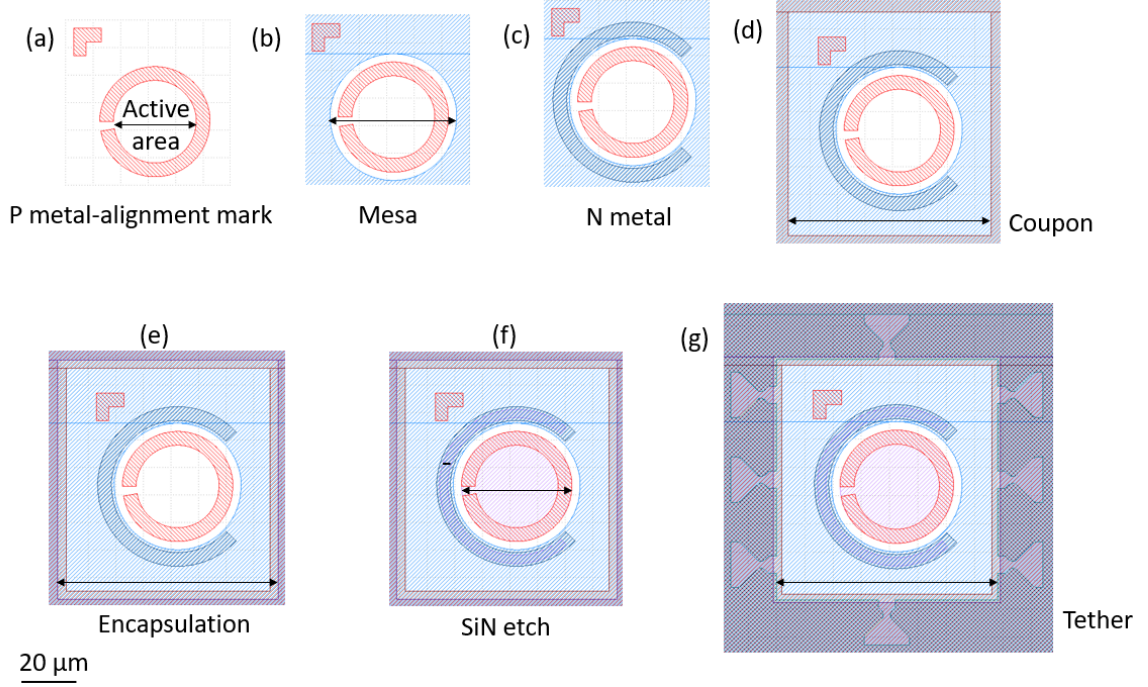
FIGURE B.1.1: Seven-layer lithography mask layout used for source wafer fabrication of the SNEAM device, with panels (a)–(g) showing the sequential mask layers. Coloured regions indicate areas exposed during the corresponding lithography step, while features from previous steps are retained for reference to illustrate layer alignment. Black arrow markers denote the lateral dimensions of the mesa and coupon features. The layouts correspond to a device aperture of 30\ \mu\text{m} .
