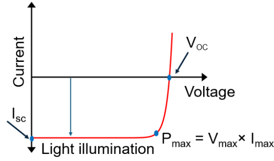
FIGURE 2.2: Schematic I-V characteristic of a PV device under illumination, shown by the red curve. The maximum power point, indicated by P_{max} , is used to calculate \eta and FF.
