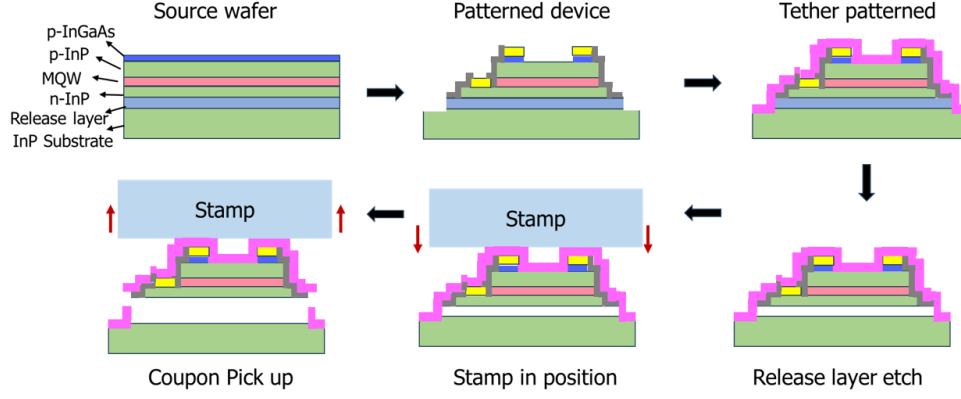
FIGURE 4.5: Overview of the fabrication process flow for the source wafer.
