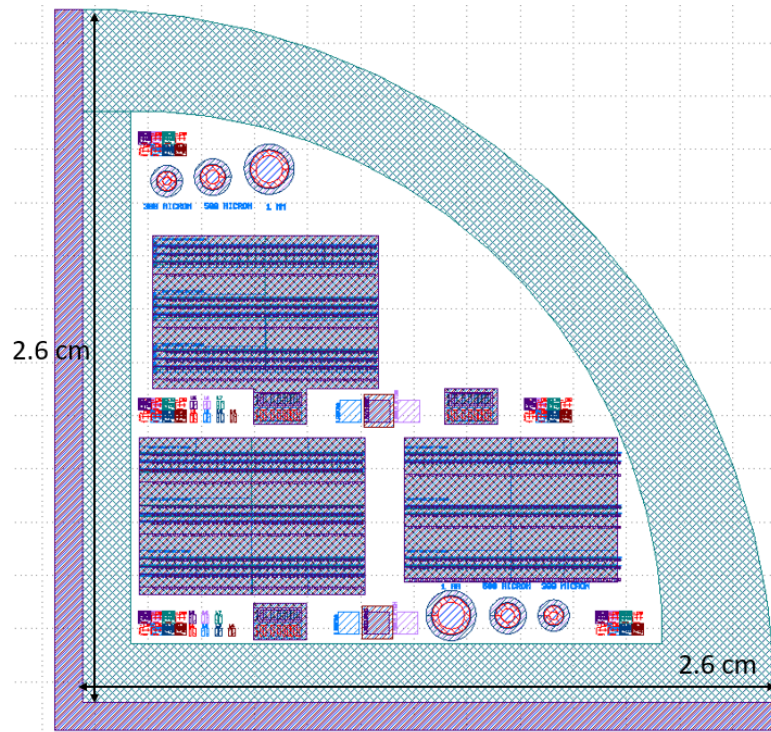
FIGURE B.3.1: Complete GDS mask layout for the SNEAM source wafer, showing the arrangement of multiple device geometry. The layout incorporates devices with different active diameters, n-metal-to-mesa gaps, and tether configurations. The designed mask occupies one quarter of the source wafer.
