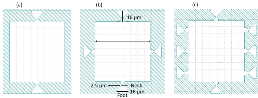
FIGURE B.2.1: GDS mask layouts showing coupon designs with different tether configurations used for source wafer fabrication. From (a)–(c) illustrate coupons incorporating two, four, and eight tethers, respectively. Shaded regions indicate areas exposed during lithography, while unshaded regions represent protected regions.
