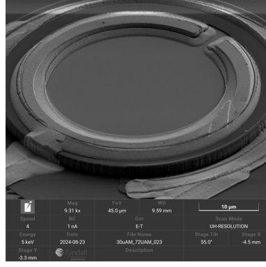
FIGURE 4.10: SEM image of the 30 \mu\text{m} SNEAM device. The active area is surrounded by a circular P-metal ring, which defines the optical access aperture relevant to fibre alignment during measurement.
