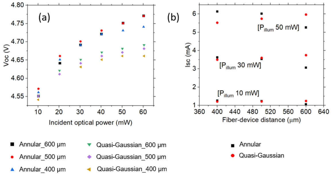
FIGURE 3.8: Comparison of quasi-Gaussian and annular beam illumination on the four segment PPC at fiber to device separations of 400 \mu\text{m} , 500 \mu\text{m} , and 600 \mu\text{m} for varying incident optical powers: (a) V_{oc} and (b) I_{sc} .
