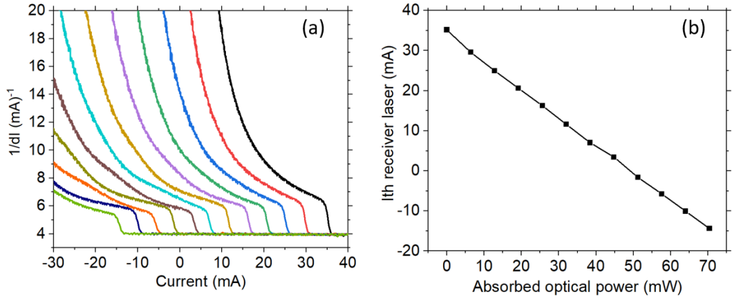
FIGURE 2.8: (a) Plot of the inverse differential current \frac{1}{dI} versus current for absorbed optical powers ranging from 0 mW (no pumping) to 70 mW. The curves are colour-coded from black (right) to light green (left), indicating increasing absorbed optical power. (b) Threshold current ( I_{th} ) as a function of absorbed optical power.
