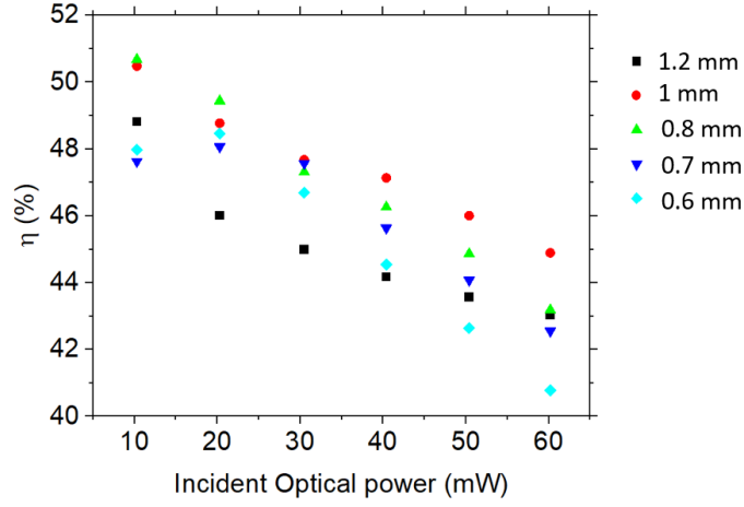
FIGURE 3.19: \eta plotted as a function of incident optical power for fiber to device distance of 0.6 mm to 1.2 mm under quasi-Gaussian illumination on Chip 2.
