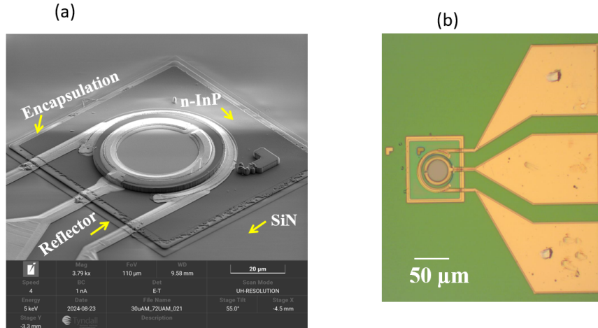
FIGURE 4.7: EAM device with an active diameter of 30 μm printed onto the target wafer: (a) Scanning electron microscope (SEM) image of the device following bondpad metallization on the transferred coupon. (b) Microscope image of the completed device showing the GSG pad configuration.
