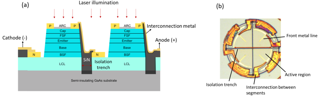
FIGURE 3.1: (a) Cross-sectional schematic of a laterally segmented, surface-normal GaAs PPC, showing the vertical layer structure, isolation trench with SiN for encapsulation, series interconnection metal, and anode and cathode contacts under surface-normal laser illumination. (b) Front view of the circular four-segment laterally connected PPC showing the device layout with isolation trenches (black cross lines) and metal connections; the red arrow indicates the device active diameter.
