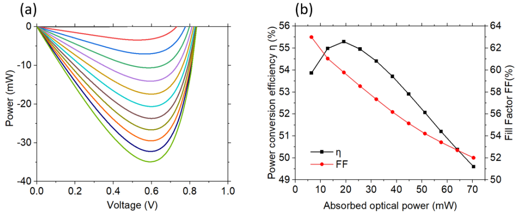
FIGURE 2.5: (a) Output P-V characteristics of the receiver laser PPC under different absorbed optical powers from 6.4 mW (red-top) to 70 mW (bright-green-bottom). (b) Variation of \eta and FF as a function of absorbed optical power, showing a gradual decrease at higher optical injection due to carrier density dependent effects.
