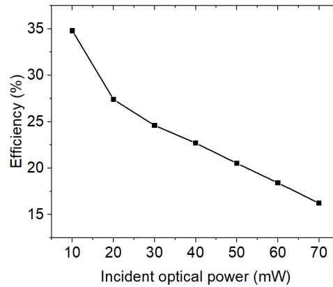
FIGURE 2.16: Efficiency of the triple-junction waveguide receiver plotted as a function of incident optical power.
