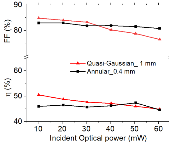
FIGURE 3.18: \eta and FF of chip 2 as a function of incident optical power under quasi-Gaussian and annular illumination for fiber to device distances of 1 mm and 0.4 mm, respectively. The results highlight that the device exhibits peak performance at these distances for each illumination condition.
