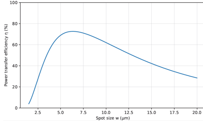
FIGURE 2.18: Calculated power transfer efficiency as a function of Gaussian beam waist, showing an optimum efficiency of approximately 72% at w \approx 6 \mu\text{m} due to the balance between junction current matching and optical spillover losses.
