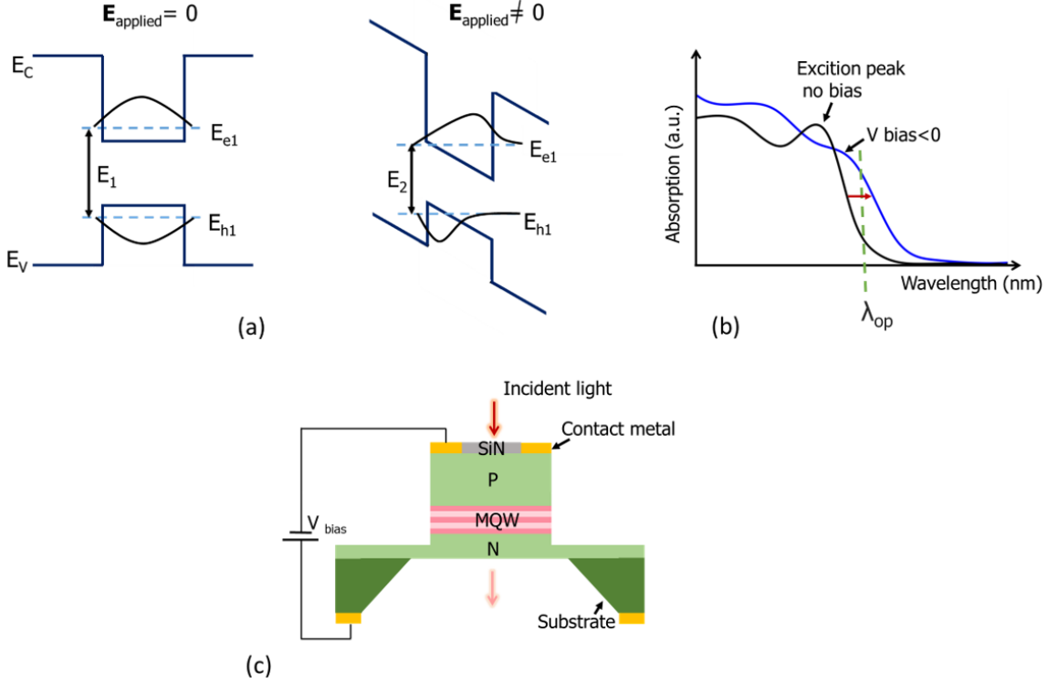
FIGURE 4.1: (a) Band diagrams illustrating the electron and hole wavefunction in a single QW, under no bias and reverse condition. (b) Schematic absorption spectra showing the QCSE-induced redshift and reduction of the excitonic peak under reverse bias, with \lambda_{op} indicating the wavelength of maximum modulation. (c) Schematic of surface normal EAM under transmission design.
