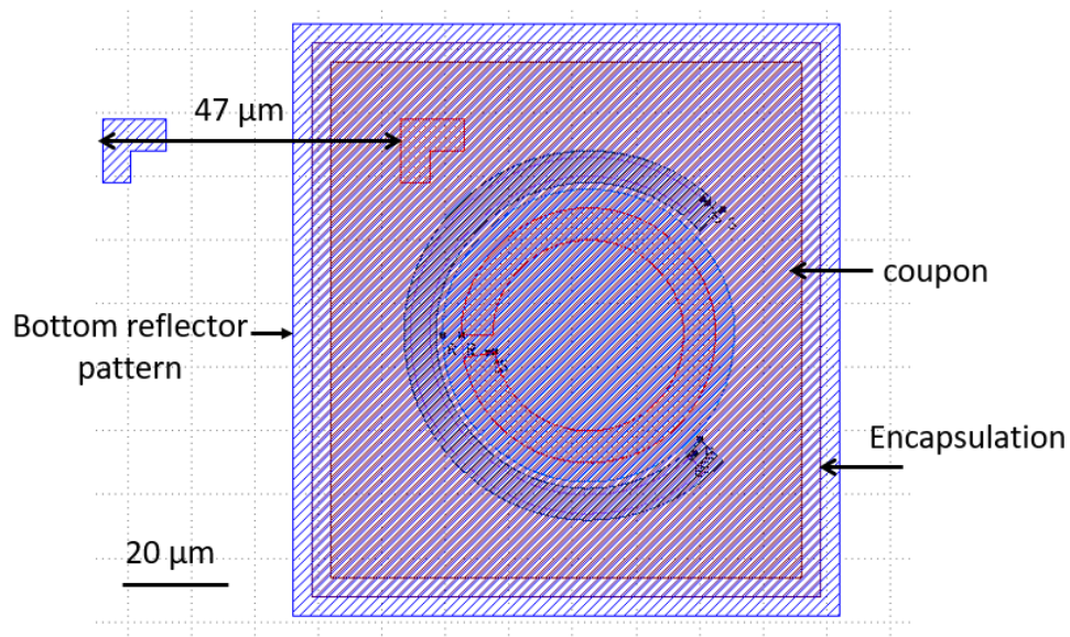
FIGURE B.5.1: Alignment of a source coupon, including the PIN device layout extracted from the GDS mask, with the patterned target location, as targeted during the transfer-printing process and observed after transfer printing.
