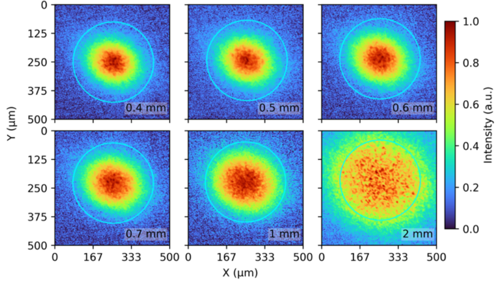
FIGURE 3.11: Quasi-Gaussian beam intensity distributions overlapped with a 350 \mu\text{m} circular disk representing the PPC active region, plotted for fiber-to-device distances ranging from 0.4 mm to 2 mm.
