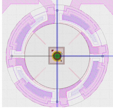
FIGURE 5.1: Layout showing the centrally positioned SNEAM with 30\ \mu\text{m} on four segmented PPC with 350\ \mu\text{m} .
