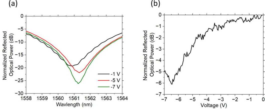
FIGURE 4.11: ((a) Normalized reflection spectra of the 30 \mu\text{m} active diameter device SNEAM device measured at reverse biases of -1 V, -5 V and -7 V, (b) Transfer characteristic showing the normalized reflected power as a function of applied reverse bias for the same device.
