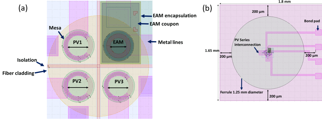
FIGURE 5.5: Suggested integrated layout of three single-junction PPCs (26 \mu\text{m} active diameter) connected in series and a central EAM (20 \mu\text{m} active area). (a) Detailed device-level layout adapted for MCF illumination. (b) Chip-level overview showing the overall chip dimensions 1.65 mm \times 1.8 mm, including fiber ferrule and wire bonding for packaging.
