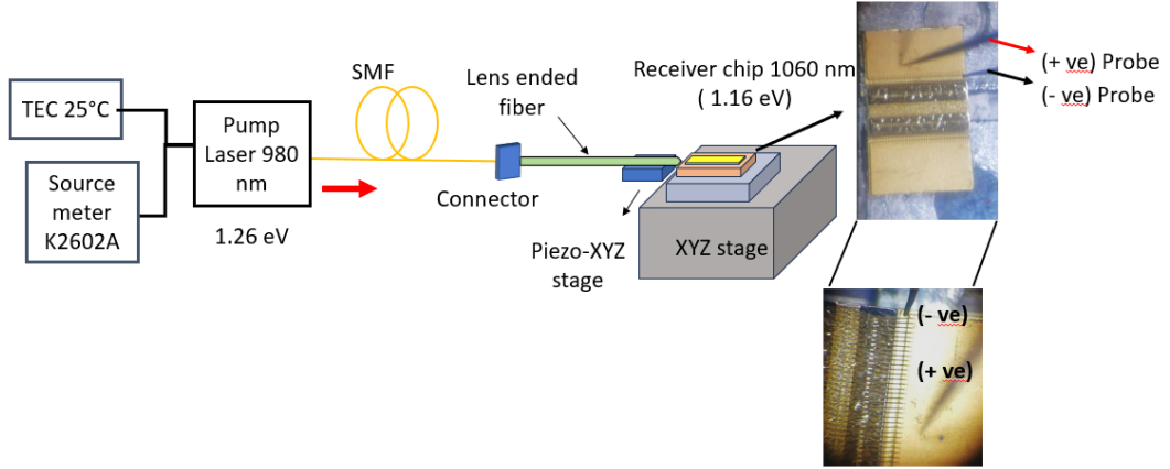
FIGURE 2.11: Experimental setup for optical power transfer using an edge-coupled waveguide laser receiver. A SMF-coupled pump laser is focused onto the receiver facet through a tapered lensed fiber mounted on an XYZ stage. The absorbed optical power generates photocurrent across the device terminals. Insets show the bare chip (top right) and needle probe placed on the chip indicating polarity (bottom right).
