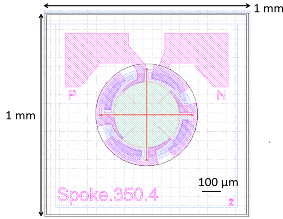
FIGURE A.3.1: Layout design of 350 \mu\text{m} active diameter PPC in 1 mm \times 1 mm chip.
