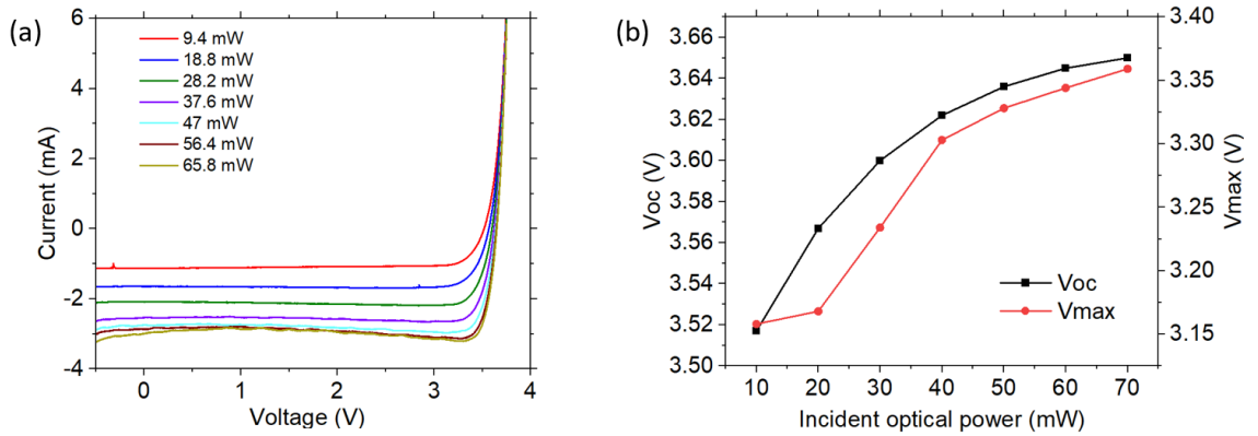
FIGURE 2.15: (a) I–V characteristics of the 905 nm triple-junction waveguide PPC under varying incident optical power from 9.4 mW (top curve) to 65.8 mW (bottom curve), showing increased photocurrent with illumination. Variations in the curves arise from optical coupling instability during measurement. (b) Variation of V_{oc} V_{mpp} with incident optical power, demonstrating voltage multiplication from the three series-connected p–n junctions and a maximum output of 3.1 V at 9.4 mW.
