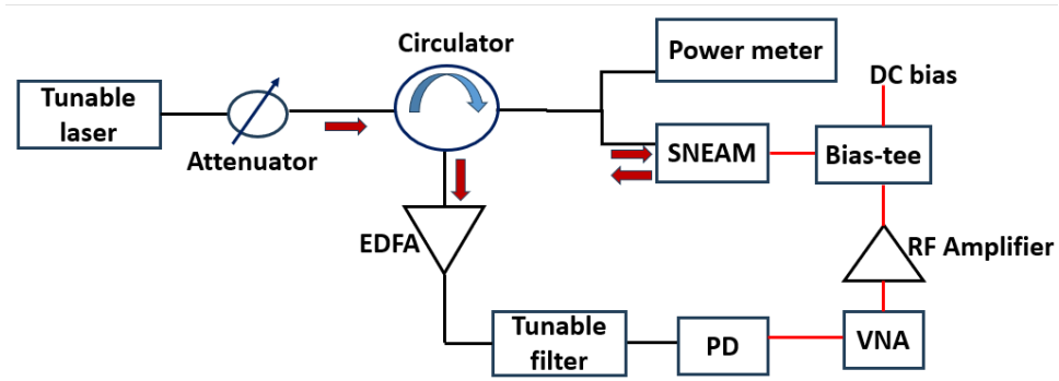
FIGURE 4.13: Schematic of experimental setup for electro-optic measurement.
