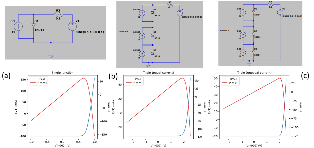
FIGURE A.2.1: SPICE-based circuit models and simulated I-V and P-V characteristics illustrating current limitation in series connected diode circuits. (a) single junction circuit driven by a current source with I_{\text{ext}}=100 mA, delivering of 60 mW; (b) three series connected diode circuits driven by equal current sources, resulting in voltage addition with I_{\text{ext}}=33.3 mA and unchanged output power of 60 mW; (c) three series connected diode circuits driven by unequal current sources, where I_{\text{ext}}=20 mA, leading to reduced output power of 40 mW.
