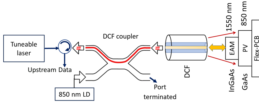
FIGURE 5.2: Schematic of single fiber solution using a DCF and a DC1300LQ2FA 2 \times 1 DCF coupler to simultaneously launch 850 nm annular illumination into the inner cladding and support bidirectional 1550 nm signal transmission through the single mode core of DCF-13.
