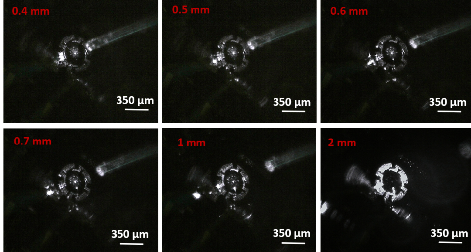
FIGURE 3.13: Illumination on the four segment GaAs PPC captured at a 45 degrees angle under quasi-Gaussian illumination for varying fiber-to-device distances.
