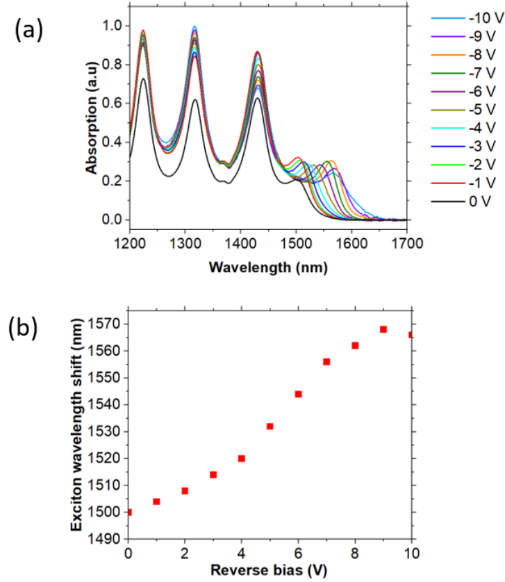
FIGURE 4.8: (a) The QCSE effect of SNEAM with presence of asymmetric FP condition. Voltage induced exciton shift tested for 30 \mu\text{m} diameter device and (b) Exciton wavelength shift versus reverse bias applied to the device.
