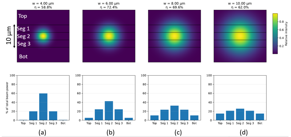
FIGURE 2.17: Numerical analysis of Gaussian beam coupling to a triple p–n junction waveguide receiver. (a–d) Simulated spatial intensity distributions at the receiver facet for increasing Gaussian beam waist values ( w = 4, 6, 8 , and 10 \mu\text{m} ), together with the corresponding fraction of optical power incident on each segment of the p–n junction stack within the 10 \mu\text{m} -high waveguide.
