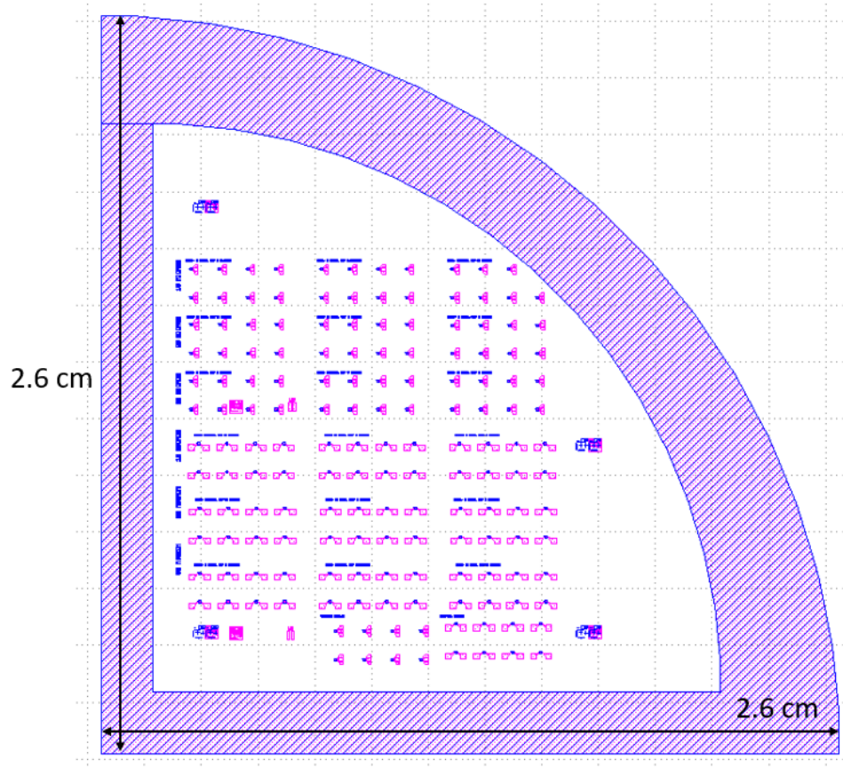
FIGURE B.4.1: Overview of the GDS mask layout for target-wafer fabrication. The mask includes definitions for the bottom reflector as well as GSG and GS bond pads to support multiple device testing and characterization. The designed mask occupies one quarter of the target wafer.
