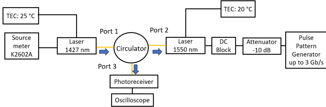
FIGURE 2.9: Schematic of the experimental setup for optical pumping and data modulation of the receiver laser using a pulse pattern generator through an optical circulator, demonstrating upstream data transmission operation. Black lines indicate electrical connections, and yellow lines represent SM optical fibers.
