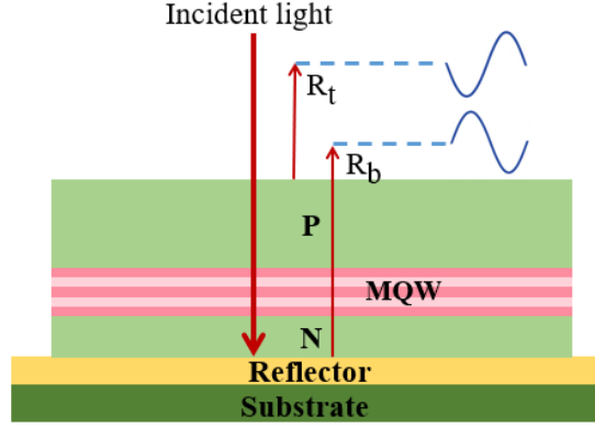
FIGURE 4.2: Schematic illustration of light reflection in the asymmetric Fabry–Perot operation of SNEAM. The top reflection R_t exhibits a 180-degree phase shift, and the bottom reflection R_b , after passing through the cavity, ideally returns with an opposite phase and an amplitude comparable to R_b , enabling destructive interference in the reflected signal.
