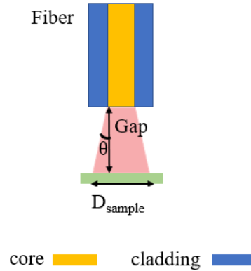
FIGURE 3.3: Schematic of the surface-normal illumination geometry showing the fiber-to-device distance ( G ). The emitted beam diverges from the fiber core at an angle \theta , expanding to a diameter D_{\text{sample}} that defines the illuminated area on the PPC surface.
