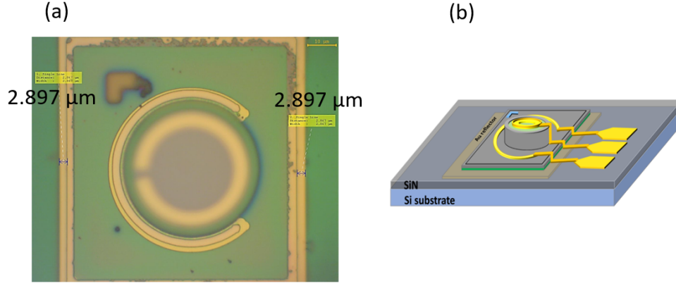
FIGURE 4.6: (a) Microscope image of the transferred coupon on the target wafer prior to GSG pad metallization, showing the alignment accuracy. (b) Schematic illustration of the printed device on the target wafer following completion of the GSG pad metallization.
