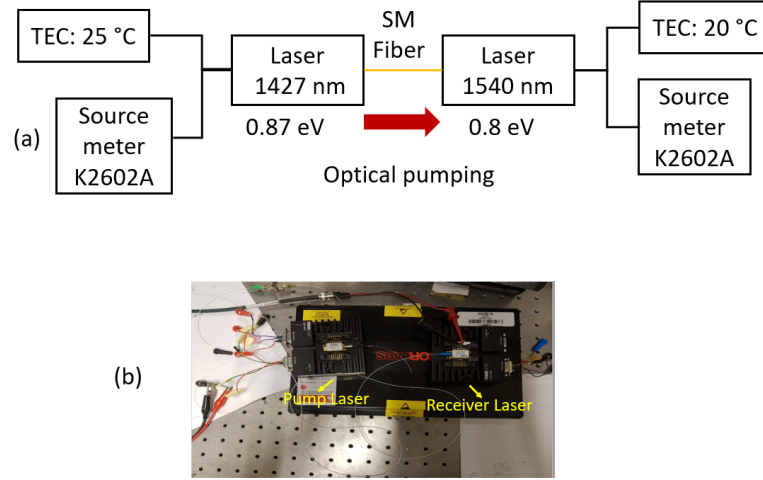
FIGURE 2.3: (a) Schematic of laser-to-laser power conversion through edge coupling using a SMF. (b) Experimental setup showing both lasers in packaged form, where the pump laser optically pumps the receiver laser and the resulting electrical current is measured using mini hook test leads connected to the receiver laser anode and cathode.
