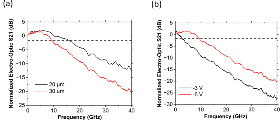
FIGURE 4.14: Normalized electro-optic bandwidth S_{21} of SNEAM devices measured for (a) 20 \mu\text{m} and 30 \mu\text{m} active diameters at -5 V bias, and (b) a 30 \mu\text{m} active diameter at -3 V and -5 V bias.
