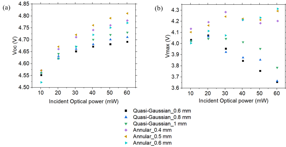
FIGURE 3.16: (a) V_{oc} and (b) V_{max} as functions of incident optical power for different fiber-to-device distances under quasi-Gaussian and annular illumination.
