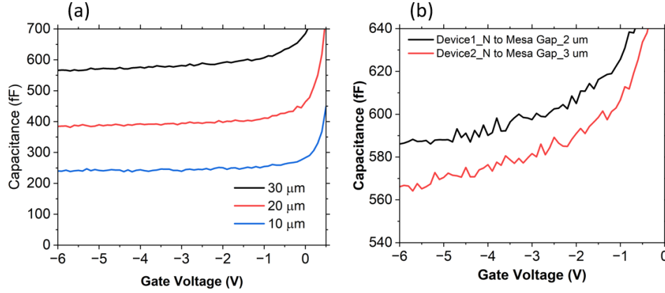
FIGURE 4.12: (a) C-V measurement for a variation of active diameter and (b) Effect of mesa-to-n-contact spacing on the capacitance of a 30 \mu\text{m} active diameter device, comparing spacings of 2 \mu\text{m} and 3 \mu\text{m} .
