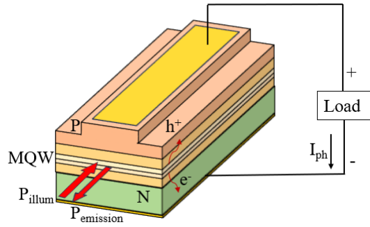
FIGURE 2.1: Schematic of the waveguide receiver laser operating as a photovoltaic (PV) converter, where incident optical power P_{illum} is absorbed in the MQW region generates carriers that produce a photocurrent I_{ph} driving an external load.
