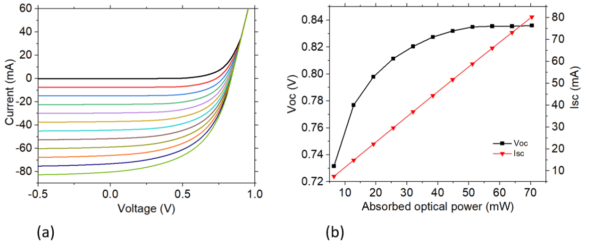
FIGURE 2.4: (a) I-V characterization of edge coupled waveguide PPC under no optical incident illumination (black curve-top) and with variation of absorbed optical power from 6.4 mW (red-top second curve) to 70 mW (bright-green-bottom). (b) Variation of V_{oc} and I_{sc} as a function of absorbed optical power, showing the logarithmic increase of V_{oc} and the linear dependence of I_{sc} with optical power.
