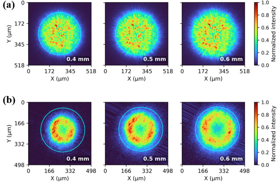
FIGURE 3.6: Normalized two-dimensional intensity distributions of the beams recorded at fiber-to-device distances of 400 \mu\text{m} , 500 \mu\text{m} , and 600 \mu\text{m} (left to right), with a 350 \mu\text{m} circular disk overlaid to represent the PPC active area. Each panel corresponds to an independently acquired beam image at the indicated fiber-to-device distance. (a) Quasi-Gaussian beam. (b) Annular beam.
