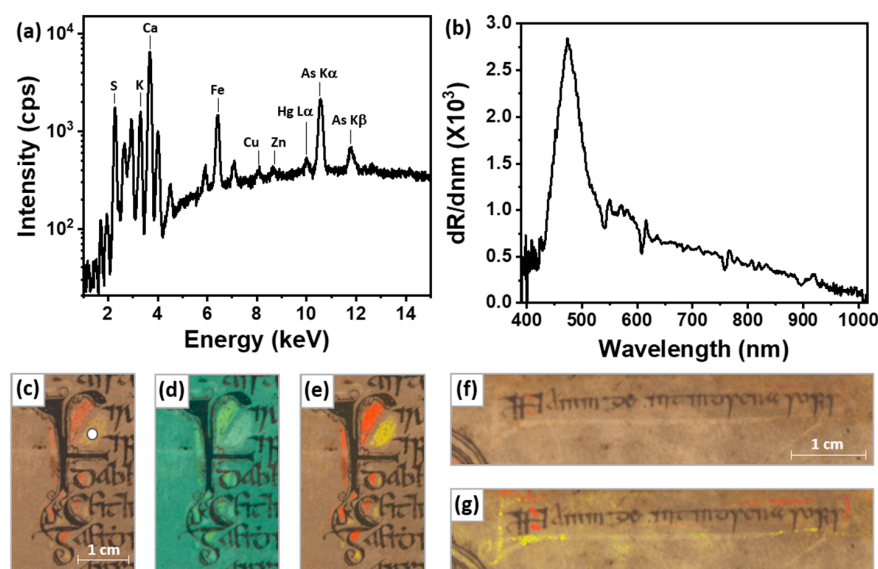
Figure 7. (a) XRF spectrum of a yellow pigment, folio 48 r; (b) Representative FORS spectrum of a yellow pigment, folio 54 v; (c–e) Visible image, IRFC, and PCA-based color reconstruction of the decoration of initial letter F (folio 48 r). White dot in visible image indicating the location where XRF spectrum was recorded; (f,g) Visible image and PCA-based color reconstruction of orpiment in probatio pennae , folio 48 r upper margin.
