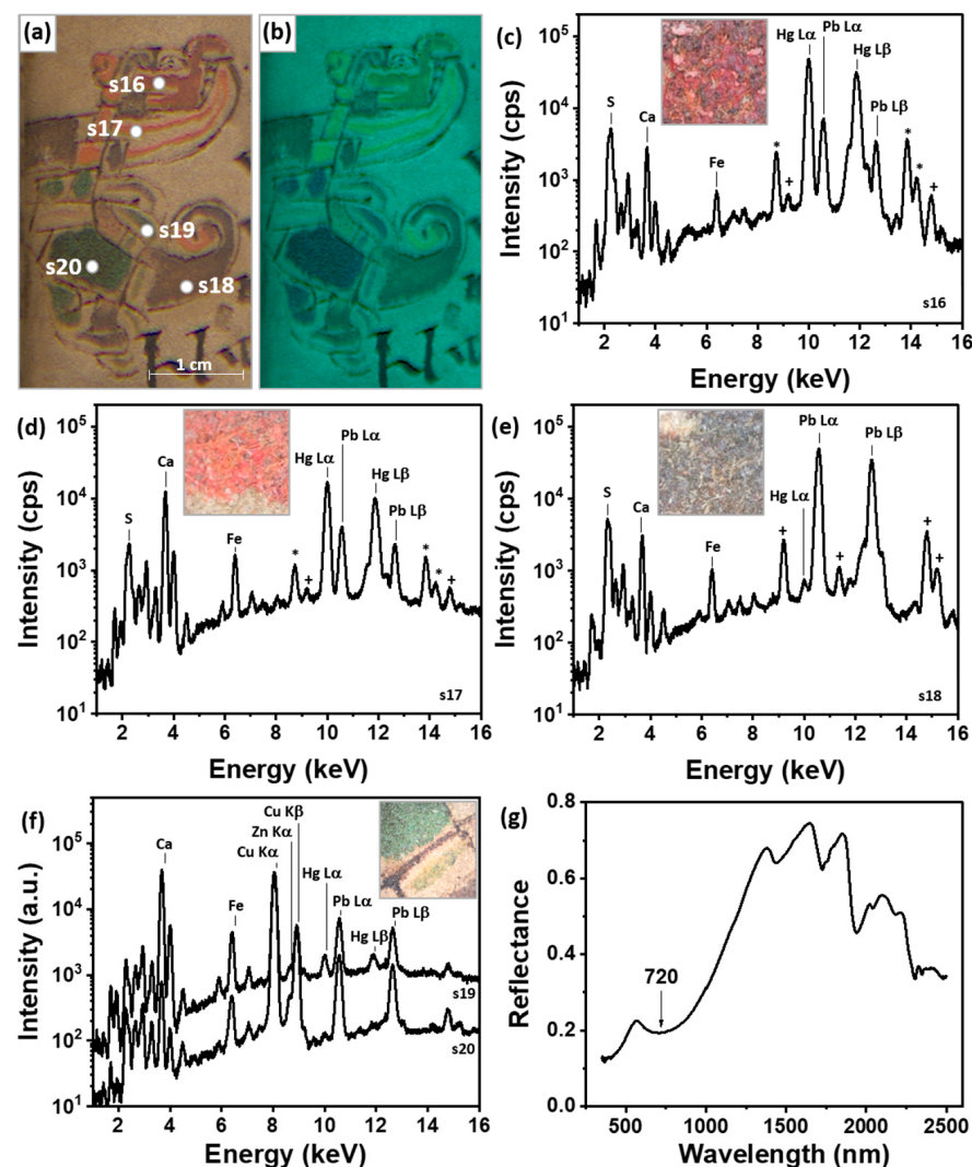
Figure 8. (a) Visible image and (b) IRFC of zoomorphic initial letter, folio 111r. White spots and numbering represent areas where XRF spectra were taken; (c–e) XRF spectra of spots 16, 17 and 18, respectively. Insets show microscopic optical images of the areas of analysis. * represents other peaks of Hg; + indicates other peaks for Pb; (f) XRF spectra of light green pigment (top spectrum, s19) and dark green pigment (bottom spectrum, s20); (g) FORS spectra of the dark green area (s20).
