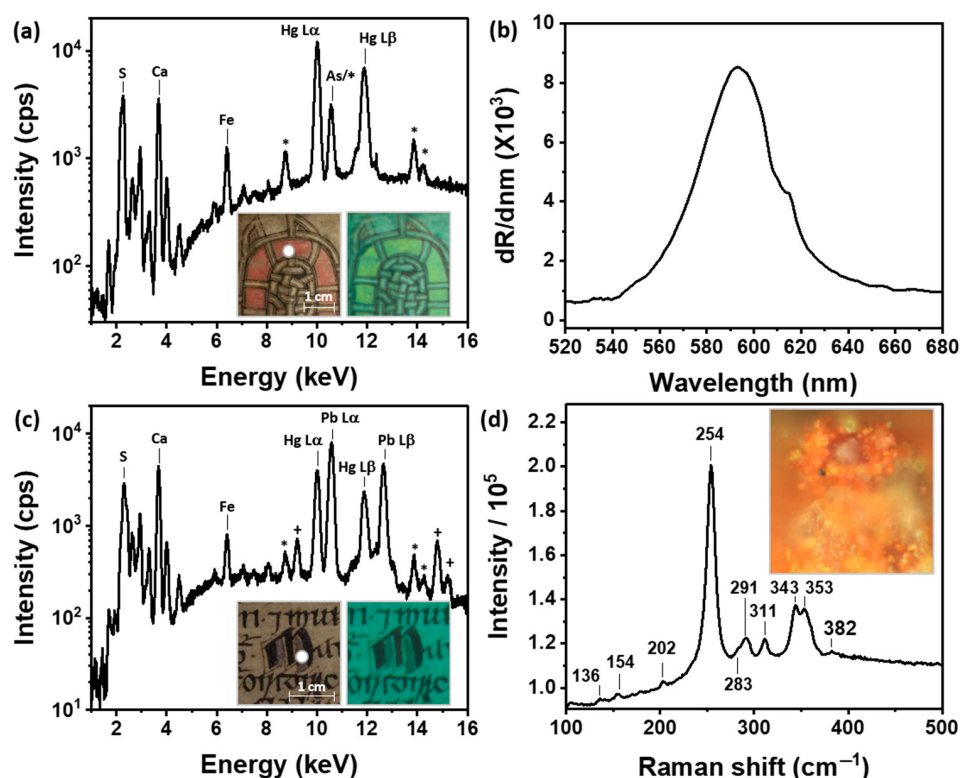
Figure 5. (a) XRF spectra of the red pigment cinnabar or vermilion. * represents other peaks for Hg. Insets show visible (left) and IRFC image (right) of the decorated initial letter in folio 48 r (quire 10). White dot in the visible image indicates where XRF analysis was performed; (b) FORS spectra confirming vermilion, folio 48 r; (c) XRF spectra of the red mixture of cinnabar/vermilion with Pb-based pigment/s. + indicates other peaks for Pb. Insets show visible (left) and IRFC image (right) of the decorated initial letter in folio 9 r. White dot in the visible image represents where XRF analysis was performed; (d) Raman spectrum, recorded using a 785 nm laser, confirms that cinnabar/vermilion and orpiment were used in mixture. Folio 50 r.
