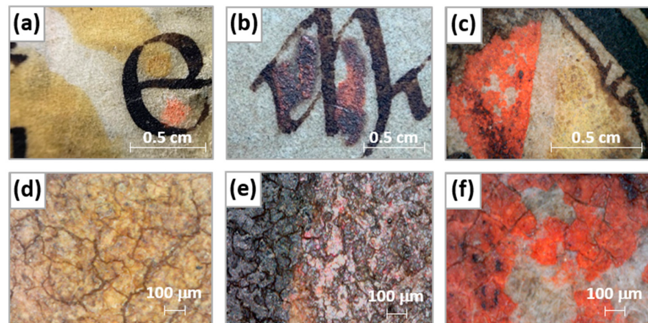
Figure 9. Optical microscopy images of pigment details across the book showing details of: (a,d) pigment migration and smudging; (b,e) pigment color change; (c,f) pigment detachment.
