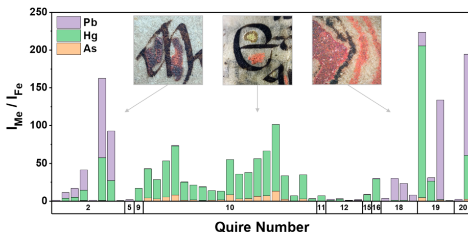
Figure 6. Histogram plotting the content of Pb, Hg, and As, ascribable to the presence of red cinnabar/vermillion, lead-based pigment(s), and orpiment (elements normalized to Fe). Insets: representative photographs of pigment applications in different red shades and yellow colorations.
