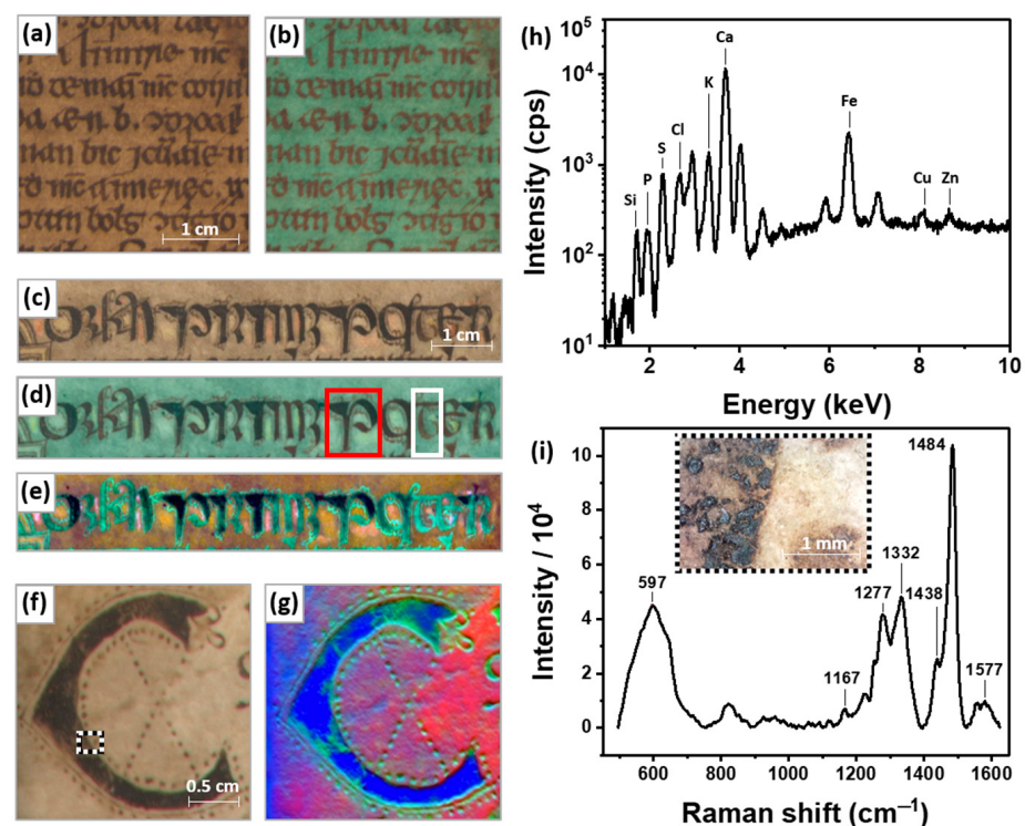
Figure 4. (a) Visible image and (b) IRFC image of a detail of folio 2 r showing body text; (c) Visible image, (d) IRFC image, and (e) Color composite image, based on PCA projections, of a detail of folio 48 r showing display text. Red box highlights a thick application of ink, while the white box highlights a thin application of ink; (f) Visible image; and (g) PCA image of a detail of folio 35 r showing the initial letter C. Dashed box highlights location of inset of (i); (h) Representative XRF spectrum of text ink, folio 2 r; (i) Raman spectrum of the letter body fragment taken at 785 nm. Inset shows an optical microscopy image of the area where the fragment dislodged.
