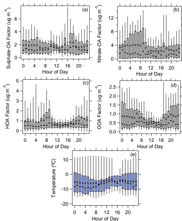
Fig. 11. Boxplots of diurnal trends for the Sulphate-OA (a) , Nitrate-OA (b) , HOA (c) , and OOA factors (d) , from the PMF Full MS analysis, along with temperature (e) . Boxes indicate interquartile ranges, horizontal lines indicate median hourly values, cross markers indicate hourly means, and whiskers represent the 5th and 95th percentiles. The HOA factor demonstrated a strong diurnal trend consistent with traffic patterns, while the OOA factor demonstrated a trend more consistent with daytime lows and overnight highs. The Nitrate-OA factor showed a minor diurnal trend indicative of more regional contributions as compared to OOA, while the Sulphate-OA factor showed minimal diurnal trend.
