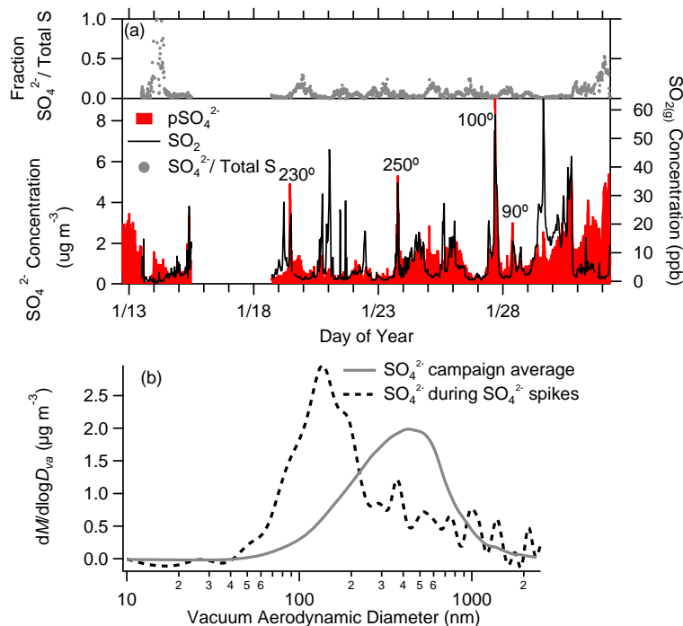
Fig. 10. Particulate sulphate concentration ( \text{SO}_4^{2-} ) vs. \text{SO}_{2(g)} concentration, and fraction of \text{SO}_4^{2-}/\text{Total } S ( \text{Total } S = \text{SO}_4^{2-} + \text{SO}_2 ) (a) . Due to the winter conditions, the fractional contribution of p\text{SO}_4^{2-} to total S was typically very low. Shown in (b) are the averaged particle size distributions of AMS \text{SO}_4^{2-} over the entire campaign, as well as during the extreme \text{SO}_4^{2-} spikes. Particulate \text{SO}_4^{2-} measured during the spikes appeared highly local due to their significantly smaller modal diameter.
