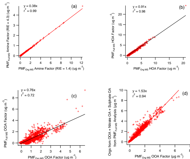
Fig. 13. Scatter plots Amine (a) , HOA (b) , and OOA (c and d) factors comparing their mass derived from PMF Full MS vs. PMF Org MS analyses. One observation (31 January 2005 21:00 LT) was removed from the HOA comparison to enhance the fit of the trendline.
