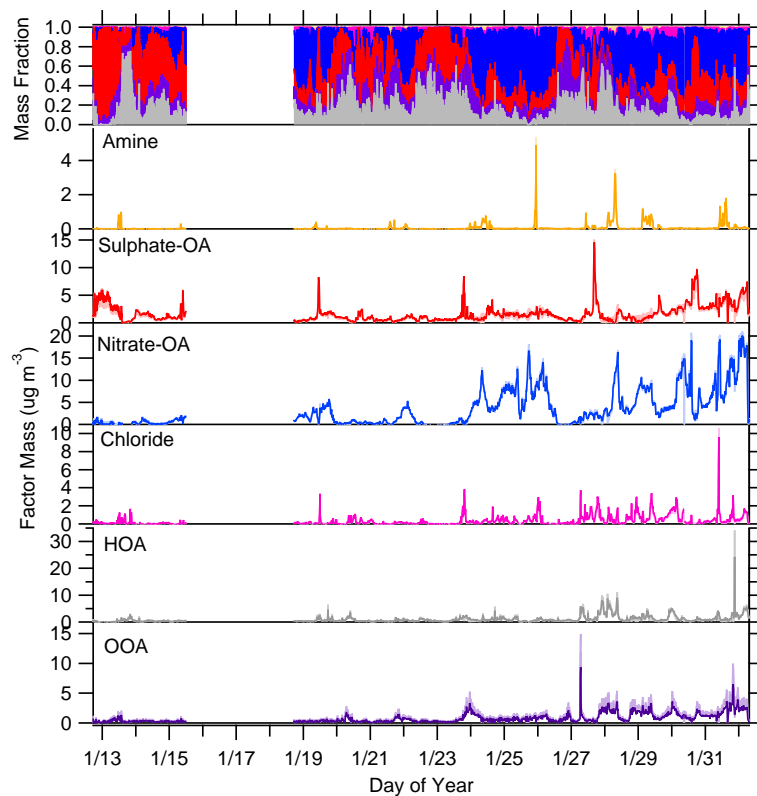
Fig. 4. Time series of the factors from the six factor solution from \text{PMF}_{\text{Full MS}} analysis. The solid line represents \text{FPeak} = 0 , and the range of uncertainties through \text{FPeak} analysis ( -10 and +10 ) is shown in the shaded regions.
