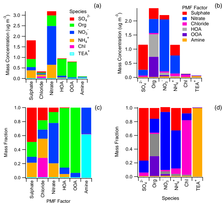
Fig. 7. Chemical composition by factor and species components of the six PMF factors from the \text{PMF}_{\text{Full MS}} analysis.
