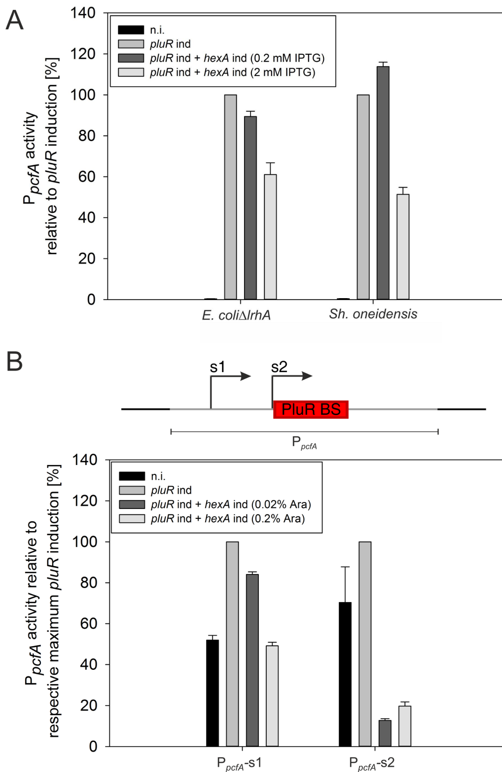
Fig 5. Effect of HexA on the P_{pcfA} activity in the heterologous systems of E. coli \Delta lrhA and Sh. oneidensis . E. coli \Delta lrhA and Sh. oneidensis were transformed with plasmids pBAD24- P_{ara} - pluR - P_{lac} - hexA and pACYC- P_{lac} - hexA - P_{ara} - pluR , respectively, in combination with plasmid pBBR- P_{pcfA} - lux . In E. coli \Delta lrhA the pluR expression was achieved via the addition of 0.1% (w/v) arabinose and in Sh. oneidensis 0.02% (w/v)
