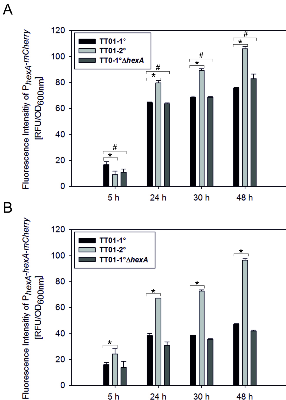
Fig 1. Transcriptional and translational levels of hexA expression. The transcriptional level, by fusing the promoter of hexA to mCherry (A), as well as the translational level, by generating protein hybrids of HexA with mCherry under the control of the hexA promoter (B), were investigated. The reporter constructs P_{hexA}\text{-}mCherry and P_{hexA}\text{-}hexA\text{-}mCherry , respectively, were integrated into the chromosome and fluorescence intensities were measured after 5 h (early exponential phase), 24 h (mid-exponential phase), 30 h (stationary phase), and 48 h (late stationary phase) in the P. luminescens
