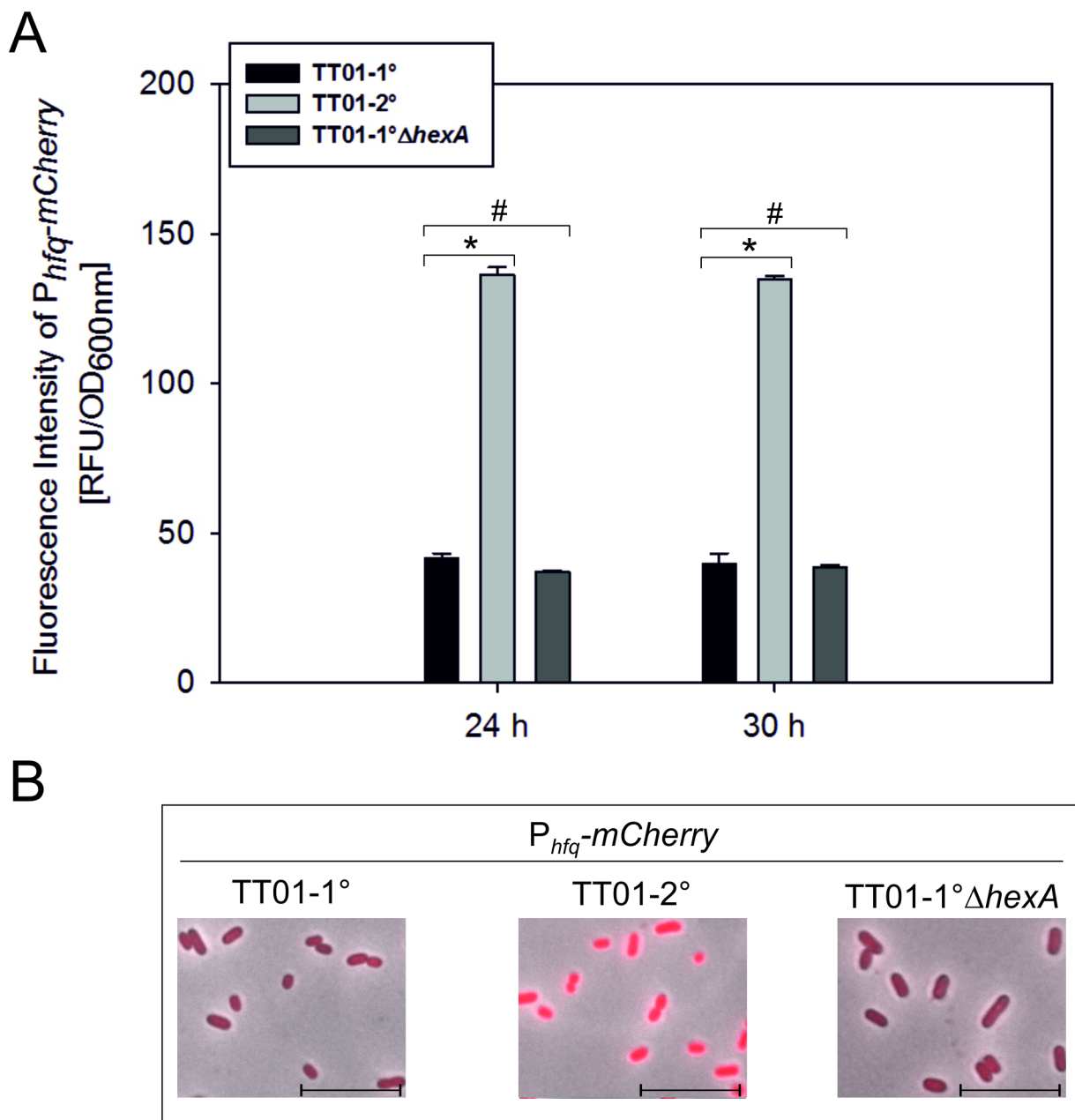
Fig 3. Transcriptional levels of hfq in P. luminescens TT01-1°, TT01-2° and TT01-1° \Delta hexA. Promoter activity of hfq at the population level. The respective reporter construct P hfq -mCherry was integrated into the chromosome and fluorescence intensities were measured after 24 h (mid-exponential phase) and 30 h (stationary phase) in the strains TT01-1°, TT01-2°, TT01-1° \Delta hexA. The asterisk (*) indicates statistically significant differences with a p-value smaller than 0.05. The hash (#) indicates no statistically significant differences with a p-value bigger than 0.05. Error bars represent standard deviation of three independently performed experiments (A). P hfq activity in TT01-1°, TT01-2° and TT01-1° \Delta hexA at the single cell level. The scale depicts 10 \mu m. Representative images from one of three independently performed experiments at time point 48 h are shown (B).
