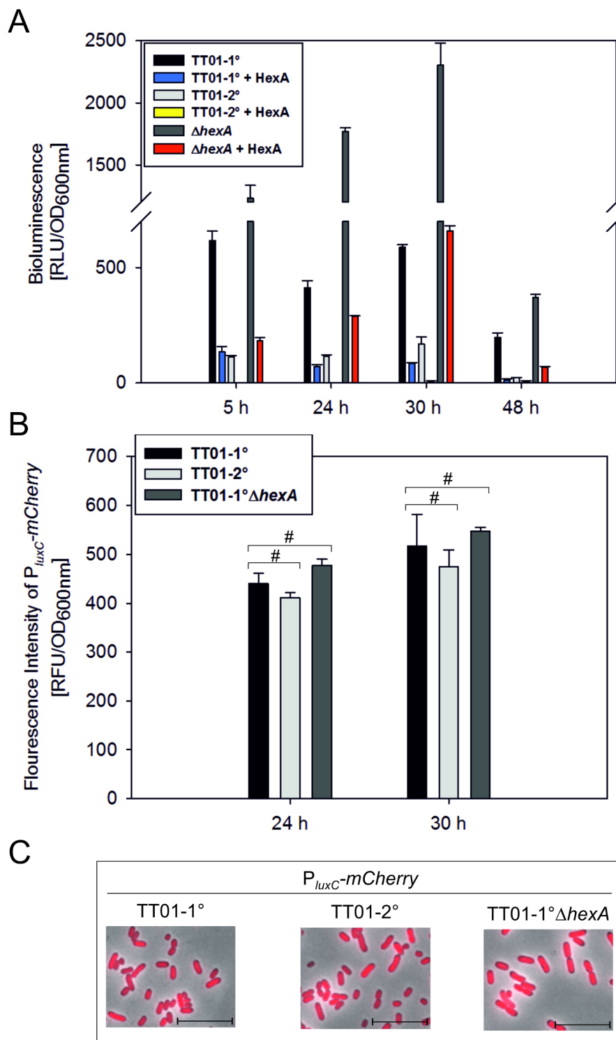
Fig 2. Effect of HexA on the bioluminescence of P. luminescens . Bioluminescence in P. luminescens TT01-1°, TT01-2° and TT01-1° \Delta hexA under native conditions and with enhanced levels of HexA. Error bars represent standard deviation of three independently performed experiments (A). Promoter activity of luxCDABE at the population level. The respective reporter construct P_{luxC} -mCherry was integrated into the chromosome and fluorescence intensities were measured after 24 h (mid-exponential growth phase) and 30 h (stationary growth phase) in the strains TT01-1°, TT01-2°, TT01-1° \Delta hexA . The hash (#) indicates no statistically significant differences with a p-value bigger than 0.05. (B). P_{luxC} activity in strains TT01-1°,
