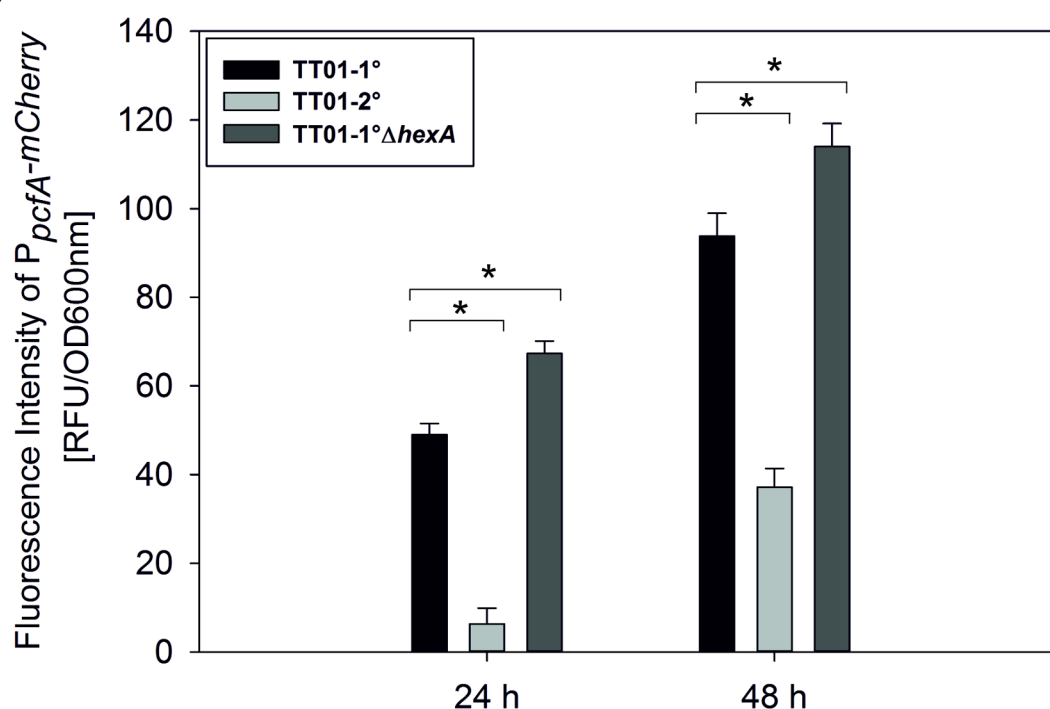
Fig 4. Cell clumping in P. luminescens TT01-1°, TT01-2° and TT01-1°ΔhexA. P_{pcfA} -mCherry activity and cell clumping in TT01-1°, TT01-2° and TT01-1°ΔhexA. The scale depicts 10 μm. Representative images from one of three independently performed experiments are shown (A). Promoter activity of pcfABCDEF at the population level in TT01-1°, TT01-2° and TT01-1°ΔhexA. The asterisk (*) indicates statistically significant differences with a p-value smaller than 0.05. Error bars represent standard deviation of three independently performed experiments (B).
