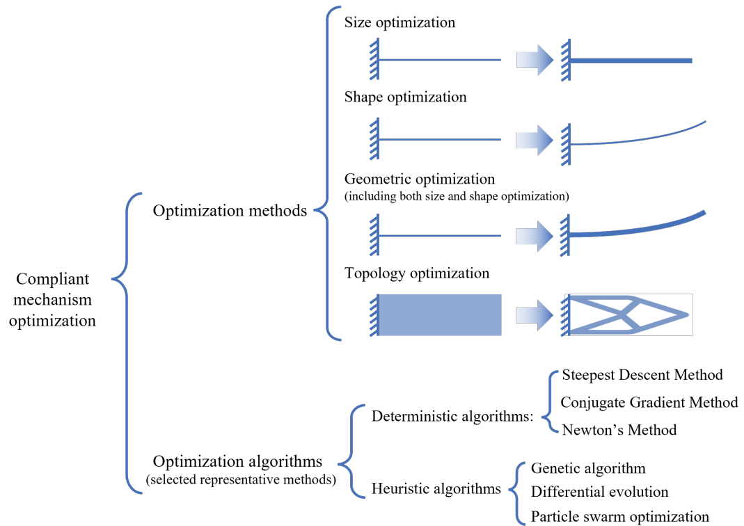
Fig. 1.7.: Classification of optimization approaches and algorithms for compliant mechanisms.
