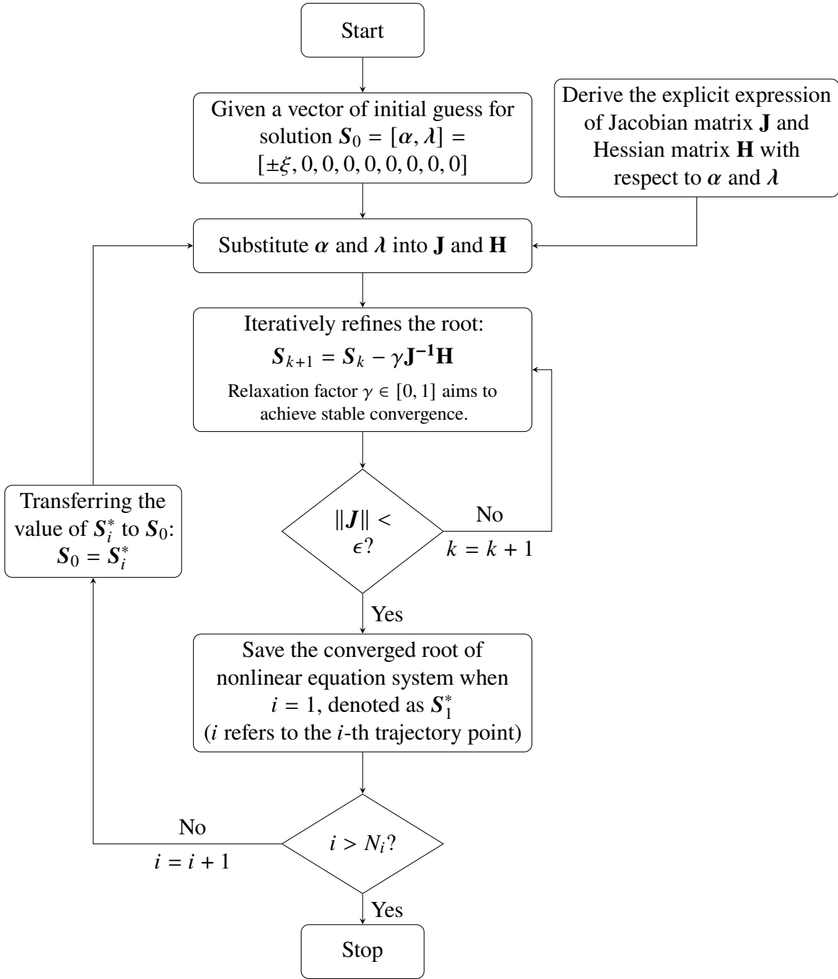
Fig. 3.2.: The flowchart of the root-finding algorithm. Before conducting the iteration, the explicit expressions of the Jacobian matrix \mathbf{J} and Hessian matrices \mathbf{H} need to be derived and used as part of the formulation during the iteration process. Then, the root-finding algorithm begins with a given initial guess S_0 . The Newton-Raphson method is then applied to determine the root of the Lagrange function as demonstrated in the flowchart. The iteration stops when the norms of the gradients have converged to the threshold \epsilon . Subsequently, the iteration process is applied to each trajectory point sequentially, until the last trajectory point.
