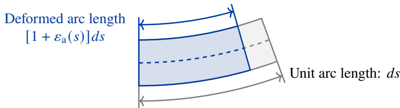
Fig. 2.2.: Illustration of stretching and compression of the neutral axis during axial deformation of a beam.
