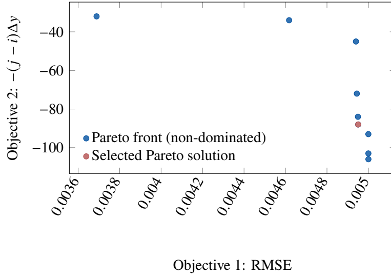
Fig. A.2.: Pareto front obtained from multi-objective optimization for a bistable mechanism with approximately constant negative stiffness. Scatter plot of the Pareto front showing non-dominated solutions in the objective space, where Objective 1 represents the RMSE and Objective 2 corresponds to the vertical displacement difference -(j-i)\Delta y . The red dot indicates the selected Pareto-optimal solution.
