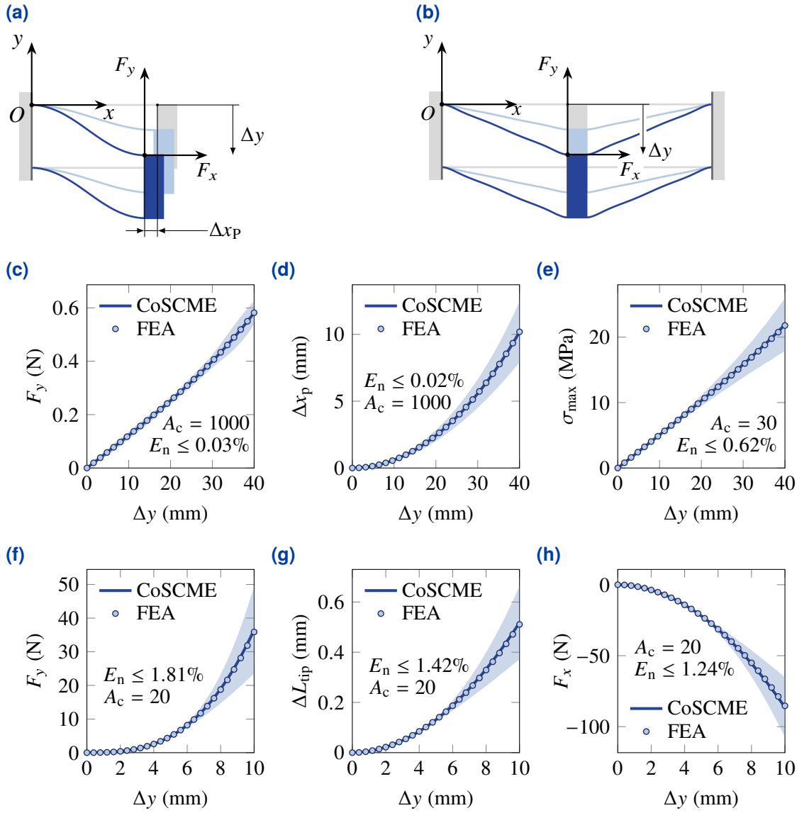
Fig. 4.6.: Modeling results for BPMs and CBPMs. (a) BPMs. (b) CBPMs. (c) F_y - \Delta y curve for BPMs. (d) \Delta x_p - \Delta y curve (parasitic movement of the moving shuttle) for BPMs. (e) \sigma_{\max} - \Delta y curve for BPMs. (f) F_y - \Delta y curve for CBPMs. (g) \Delta L_{\text{tip}} - \Delta y curve for CBPMs. (h) F_x - \Delta y curve for CBPMs.
