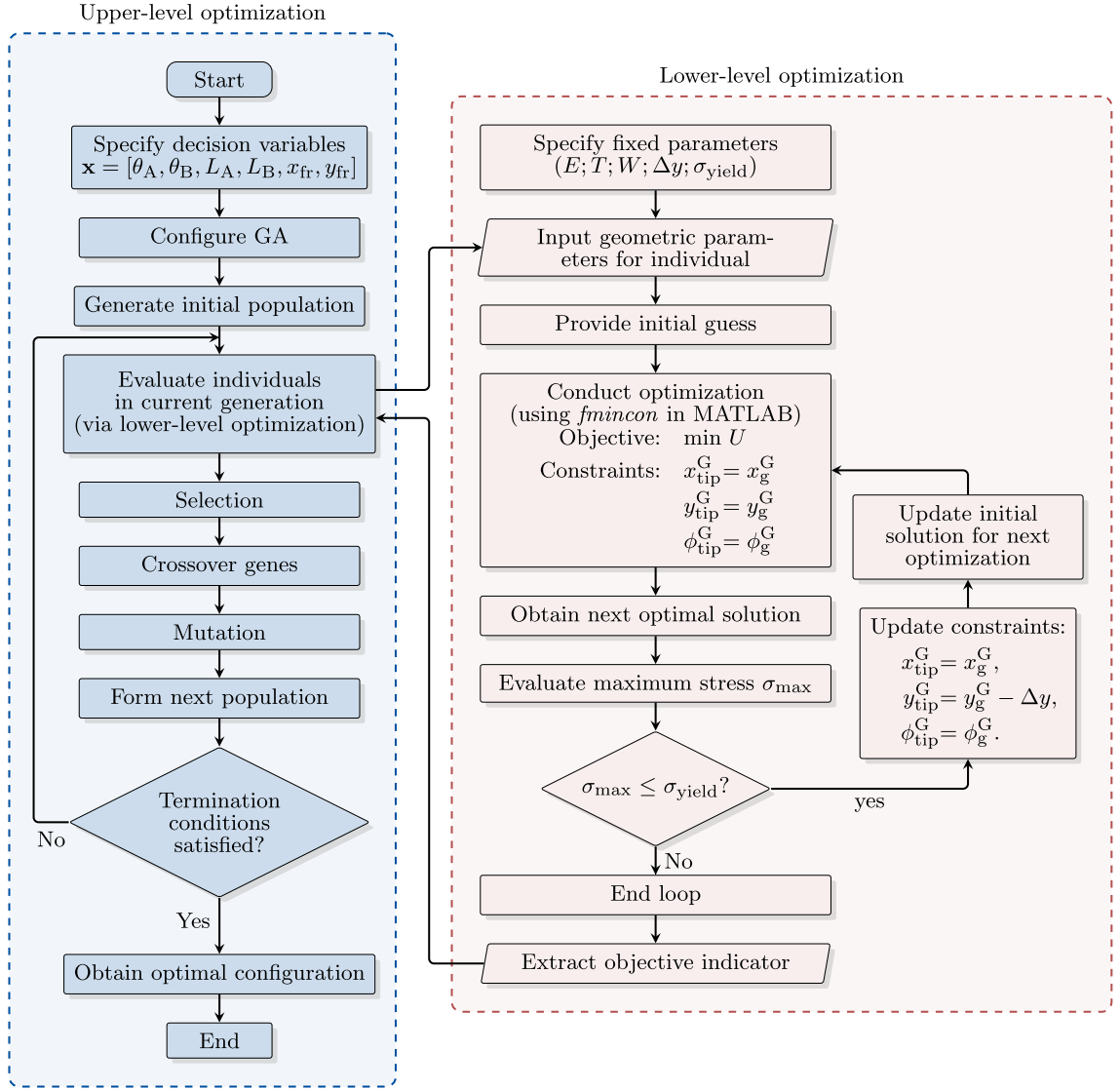
Fig. 5.1.: The flowchart of bi-level optimization.
