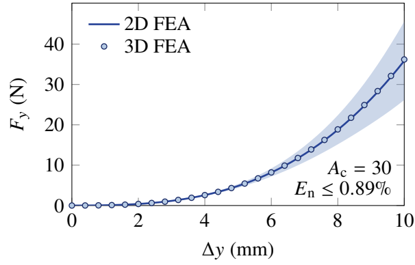
Fig. 4.4.: Comparison of 2D and 3D FEA simulation results for CBPMs under nonlinear static loading. The 2D model uses beam elements with 100 segments per beam, while the 3D model employs Quad4 elements with a maximum edge length of 2% of the beam length. Both models share consistent material properties and boundary conditions.
