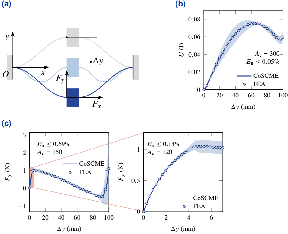
Fig. 4.11.: Case study of modeling a compliant bistable mechanism with initially curved beams. (a) Deformation results of the compliant bistable mechanism. The coordinate system, displacement direction, and reaction force are shown in the plot. (b) The strain energy curve during deformation. All results are validated by FEA simulations. The geometric parameters used describing this cosine-shaped beam is: T = 180\text{mm} , A = 25\text{mm} . (c) The modeling result of reaction force F_y . The figure on the right shows a zoomed-in result for more detail.
