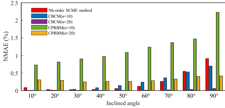
Fig. 3.14.: Modeling error comparison among the 5th-order SCME method, CBCM, and CPRBM. Ten and twenty beam elements are used in CBCM and CPRBM. The inclined angles gradually increase from 10 to 90 degrees.
