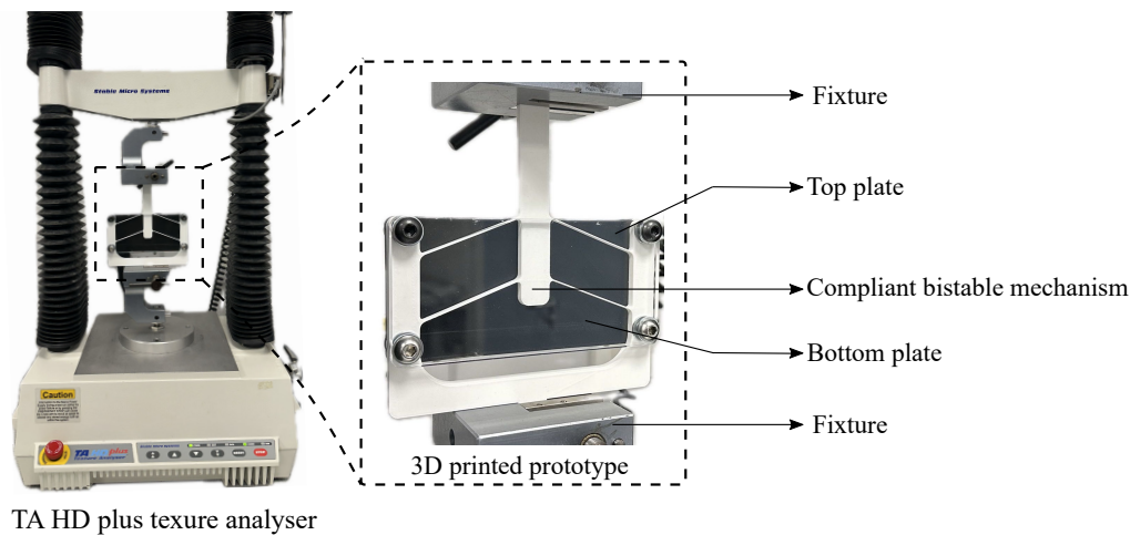
Fig. 3.9.: The experiment setup and 3D printed prototype. The experiment is conducted on the TA HD plus texture analyzer. The 3D printed prototype consists of three layers, including top and bottom plates, which are used to enhance the lateral stiffness. The middle layer is the 3D printed compliant bistable mechanism.
