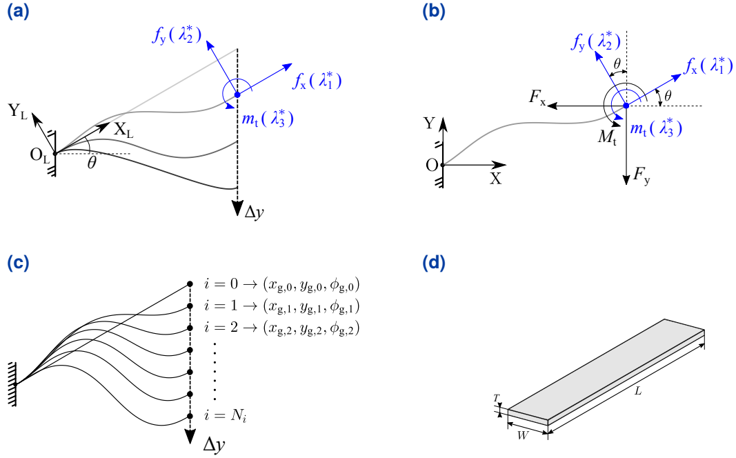
Fig. 3.1.: Explanation of local and global coordinate systems, trajectory points, and geometric parameters of compliant beams. (a) Definition of local coordinate system. (b) Definition of global coordinate system. (c) Definition of discrete trajectory points. (d) Definition of geometric parameters.
