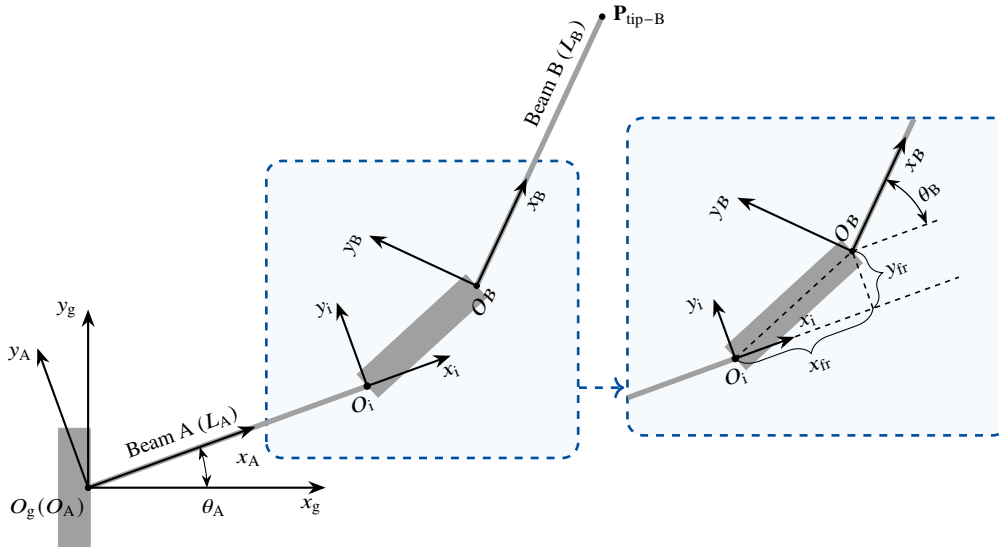
Fig. 5.2.: Definition of geometric layout and coordinate systems of lumped-compliance beam. The beams are rigidly connected to each other without hinges.
