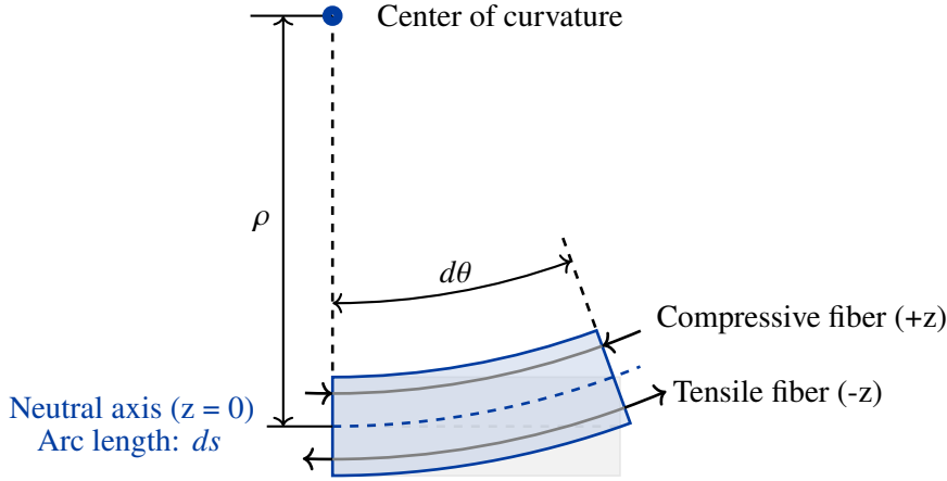
Fig. 2.1.: Illustration of compressive and tensile fibers in beam bending deformation.
