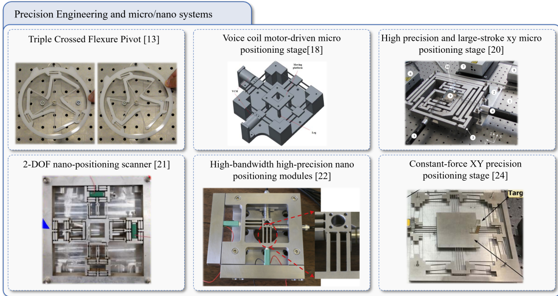
Fig. 1.2.: Applications of compliant mechanisms in precision engineering and micro/nano systems.
