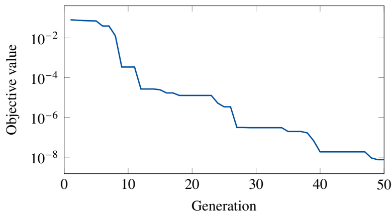
Fig. A.1.: Convergence history of the optimization for bistable mechanism with symmetric switching force.
