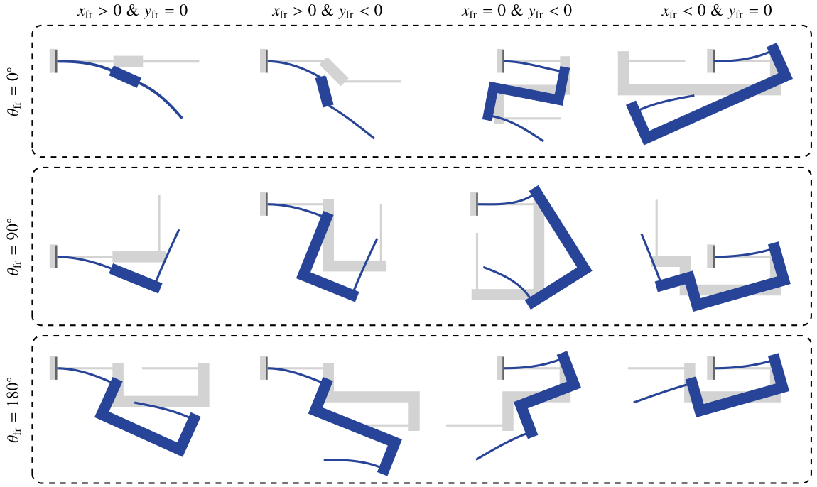
Fig. 4.10.: Twelve distinct configurations of general lumped-compliance beams. These beams are developed by adjusting frame parameters ( x_{fr} , y_{fr} , and \theta_{fr} ), which is inspired by the position-space-based compliant mechanism reconfiguration approach. The undeformed configurations are represented in grey, while the deformed configurations are shown in blue. The deformations are obtained from modeling results of the CoSCME. A vertical displacement load is applied to all of these general lumped-compliance beams, with the tips of each beam B free to rotate.
