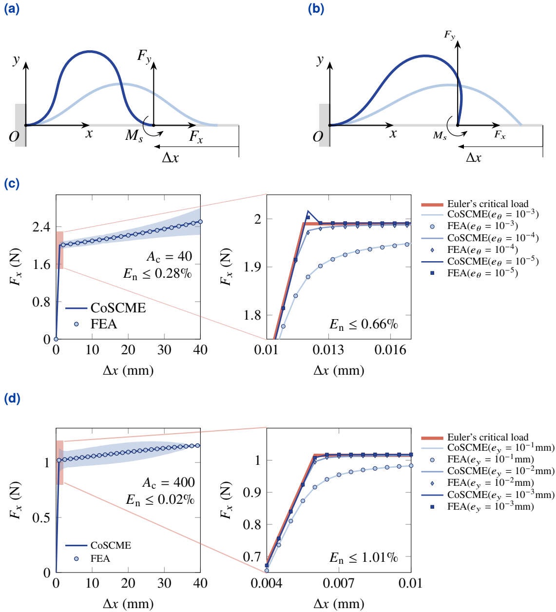
Fig. 4.5.: Modeling result of fixed-fixed beam and fixed-pinned beam. (a) Fixed-fixed beam. (b) Fixed-pinned beam. (c) F_x - \Delta x curve for fixed-fixed beam. (d) F_x - \Delta x curve for fixed-pinned beam.
