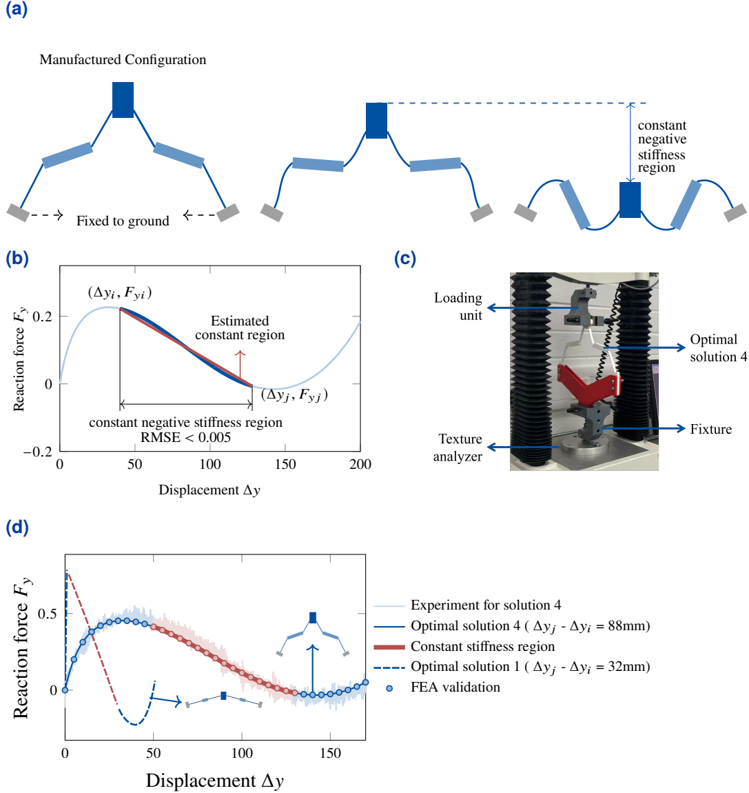
Fig. 5.5.: Illustration and validation of the optimized mechanism with constant negative stiffness. (a) Optimized configuration with labels indicating the original design and the constant negative stiffness region. (b) Visualization of optimization objectives. (c) Experimental setup for static testing. (d) Force–displacement curves of optimal solutions 1 and 4. Kinetostatic behavior of optimal solution 4 is validated through FEA simulations and experiment.
