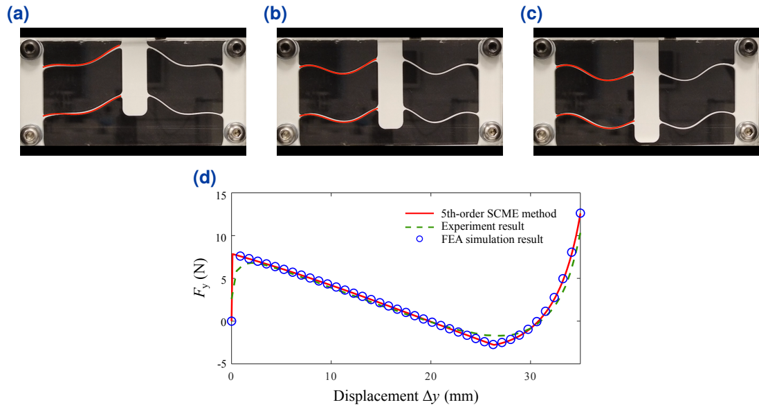
Fig. 3.10.: Experiment result comparison. The red continuous line represents the predicted deformation shape obtained from the SCME method. (a) Deformation shape comparison when \Delta y = 5\text{ mm} . (b) Deformation shape comparison when \Delta y = 15\text{ mm} . (c) Deformation shape comparison when \Delta y = 25\text{ mm} . (d) Force-displacement relationship comparison among the SCME method, experiment, and FEA simulation. Note that the total force obtained through the 5th-order SCME method is four times the force calculated for a single compliant beam. This is because the designed prototype incorporates four beams.
