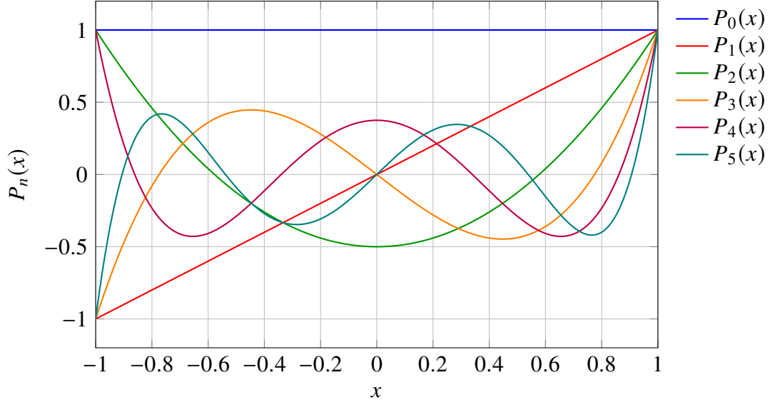
Fig. 2.3.: The first six Legendre polynomials P_0(x) – P_5(x) defined on the interval x \in [-1, 1] . Different colors are used to distinguish polynomial orders.
