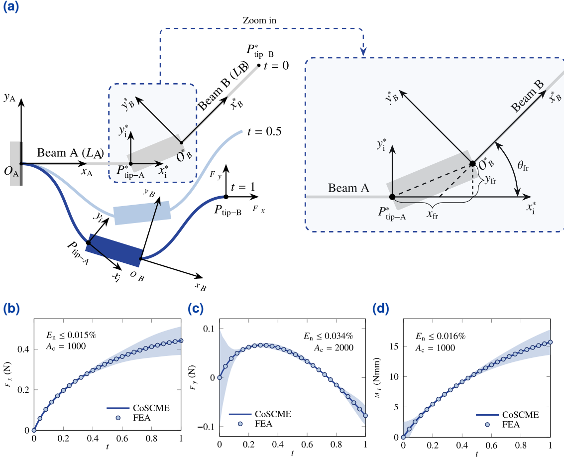
Fig. 4.9.: Case study of modeling a general lumped-compliance beam, which is composed of two compliant beams. A displacement load and a rotational load are applied to the tip of beam B. The deformation result is derived from the modeling using the CoSCME. (a) Terminology used for modeling the general lumped-compliance beam. The deformation process is described using the parameter t \in [0, 1] . Coordinate systems are defined in the figure, and all the coordinate systems for the initially undeformed configuration are marked with *. (b) Modeling results obtained from the CoSCME and FEA simulations, including reaction forces along the x - and y -directions, and the tip reaction moment M_t .
