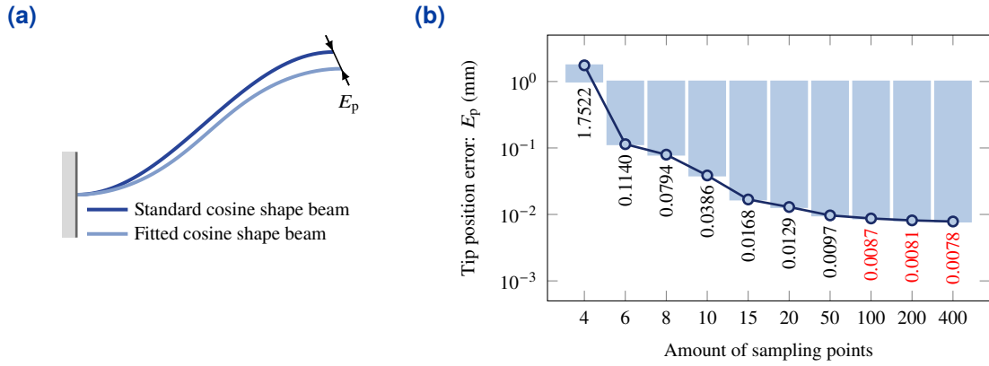
Fig. 4.12.: Convergence analysis of beam shape fitting. (a) Error comparison between the standard and fitted cosine-shaped beams. (b) Convergence analysis results.
