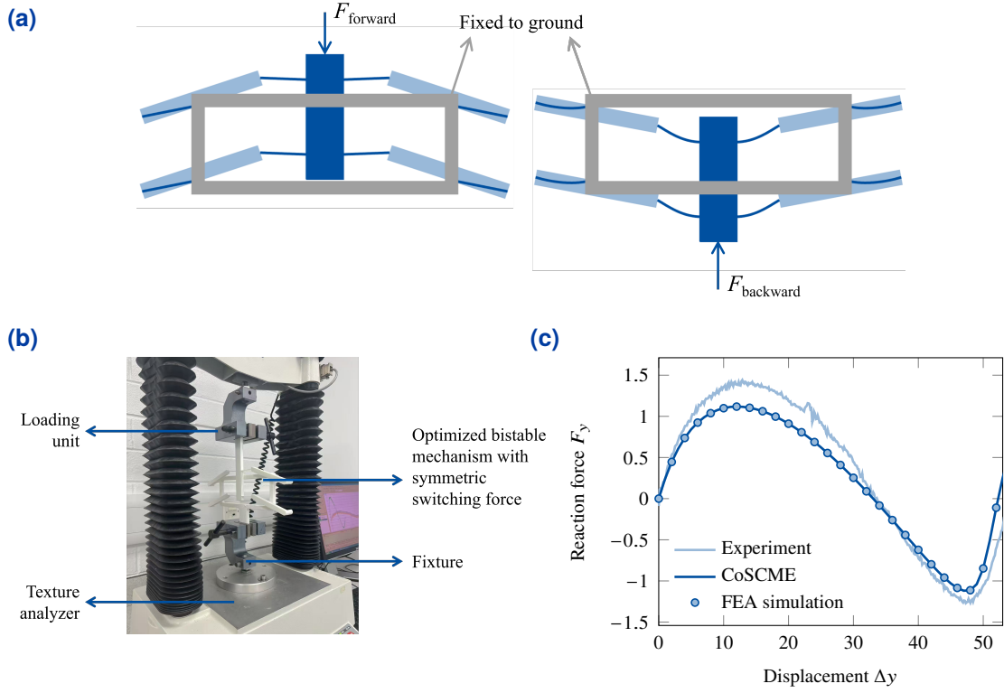
Fig. 5.4.: Optimal design of the bistable mechanism with symmetric switching force. A double-layer design is adopted to more effectively reduce the geometric size of the prototype. (a) The first and second stable configurations of the optimized mechanism. The grey block indicates the fixed part attached to the ground. The directions of the forward and backward forces are marked. (b) Force–displacement curve of a single lumped-compliance beam, validated by FEA simulation and experiment. (c) Experimental setup for testing the static behavior of the optimized mechanism.
