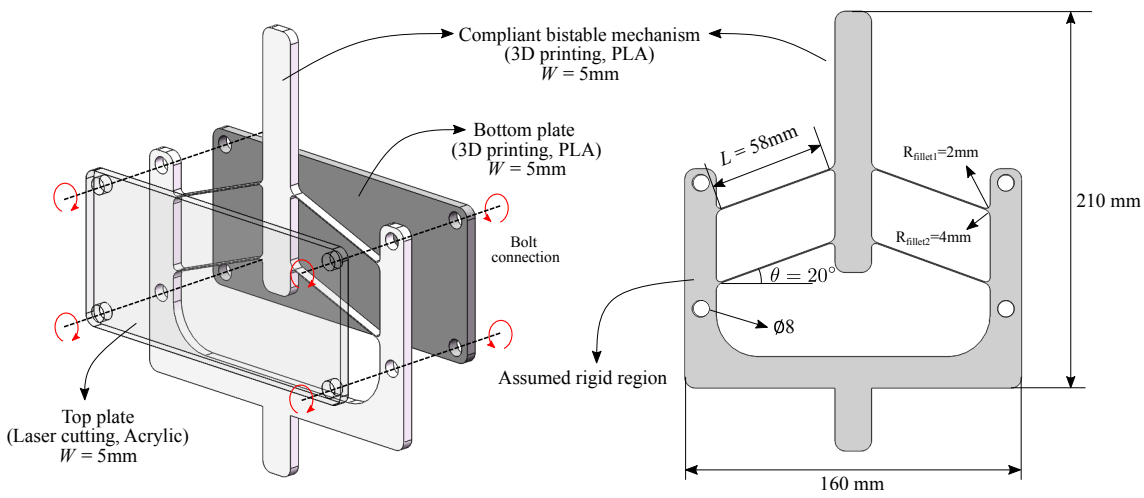
Fig. 3.8.: A prototype with three layers used for experimental validation. The bottom plate and top plate are designed to ensure sufficient stiffness of the rigid components while maintaining the entire mechanism in a relatively compact size. The middle layer is compliant bistable mechanism. Laser cutting is applied to manufacture the top plate, and transparent acrylic material is used to guarantee the visibility of deformation. The geometric parameters of the compliant bistable mechanism can be observed on the right side. Fillets are applied to the roots of beams to avoid stress concentration problems. The beam in-plane thickness T is designed to be 0.8mm.
