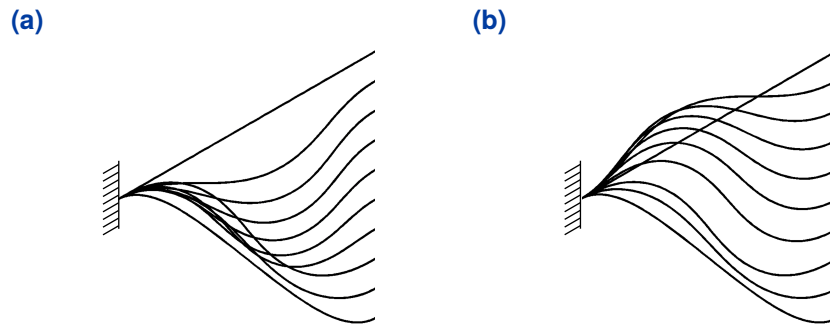
Fig. 3.3.: Two possible deformation shapes exist in modeling results. The distinct deformation shapes are induced by setting the initial guess of the root in the root-finding procedure. The sign of \xi affects the deformation shape (buckling direction). (a) Possible deformation shape A: when a positive \xi is given in initial guess S_0 . (b) Possible deformation shape B: when a negative \xi is given in initial guess S_0 .
