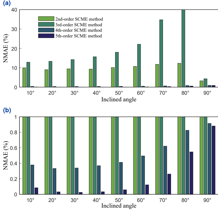
Fig. 3.12.: Modeling error comparison among 2nd-, 3rd-, 4th-, and 5th-order SCME methods. The error is measured using normalized mean absolute error. The comparison result indicates that the 5th-order SCME method is the most accurate. (a) The range of NMAE varies from 0% to 40%. (b) The range of NMAE varies from 0% to 1%.
