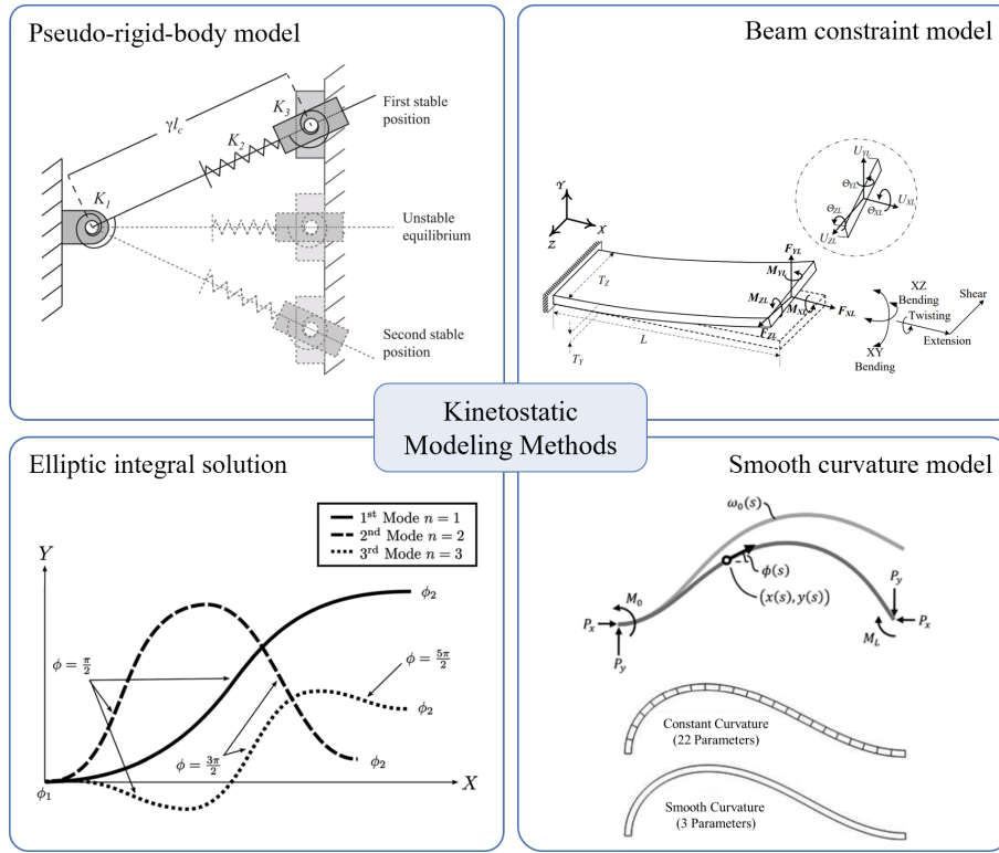
Fig. 1.6.: Representative kinetostatic modeling methods for compliant mechanisms. The pseudo-rigid-body model approximates flexible deformations using rigid links and torsional springs. The beam constraint model captures large deflections through force-moment relations at beam ends. Elliptic integral solutions provide exact analytical descriptions for certain beam configurations, but require discussion on number of inflection points. The smooth curvature model describes the continuous deformation of compliant members with a small number of parameters, offering a balance between accuracy and computational efficiency.
