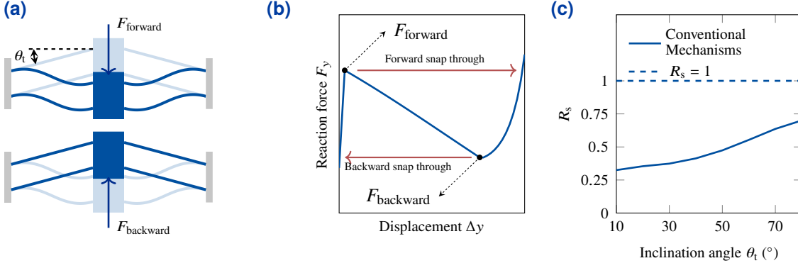
Fig. 5.3.: Forward and backward switching force analysis for conventional distributed-compliance bistable mechanisms. (a) Schematic of forward and backward switching forces, with beam inclination angle denoted by \theta_t . (b) Illustration of forward and backward switching force from the force-displacement relationship. (c) Relationship between inclination angle \theta_t and switching force ratio R_s .
