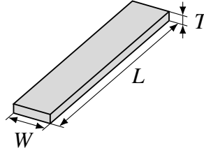
Fig. 4.3.: Definition of geometric parameters: L is the beam length, W is the beam width, and T is the beam thickness. In the following case studies involving initially straight beams, all beams are defined with L = 100\text{mm} , W = 10\text{mm} , T = 0.8\text{mm} .
