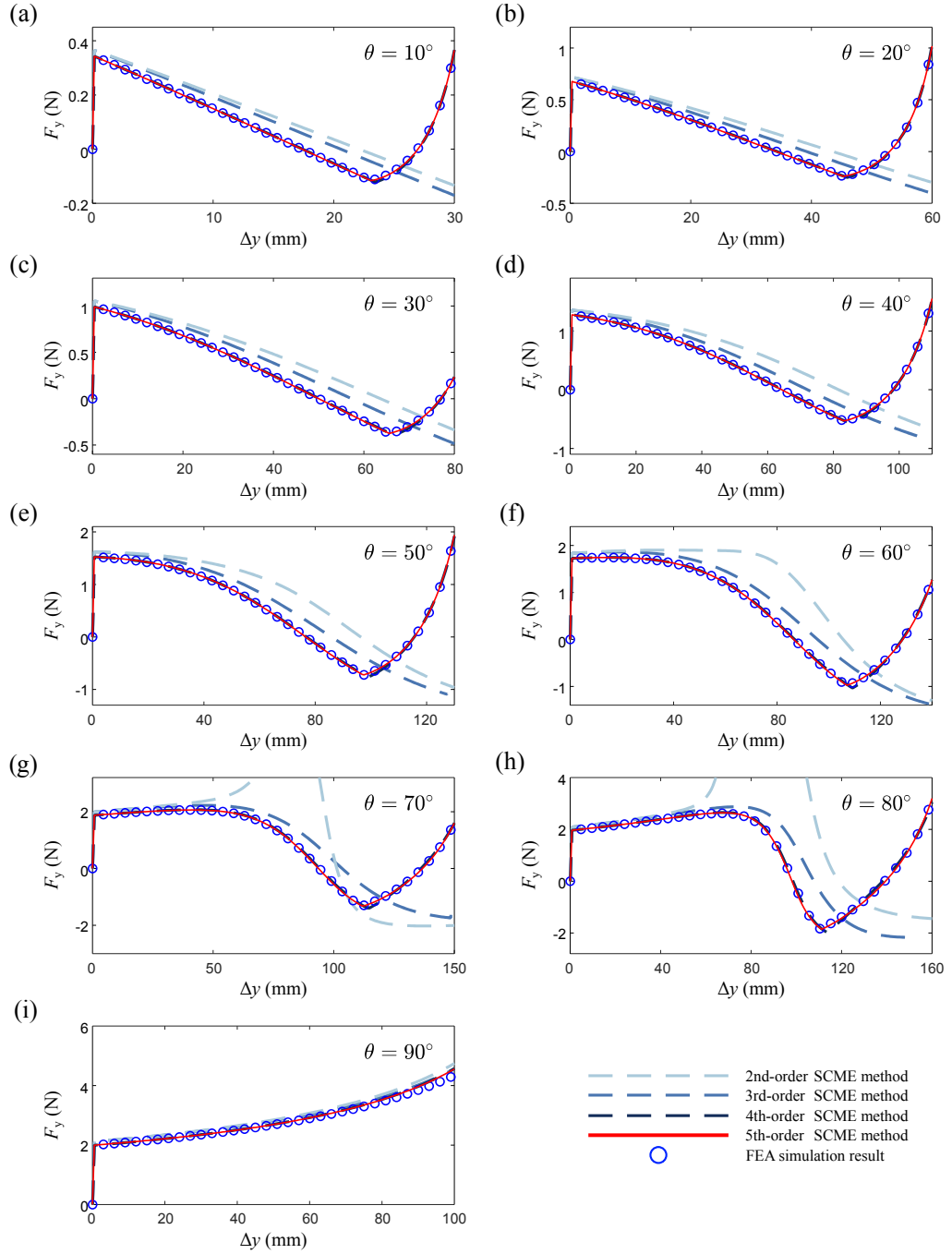
Fig. 3.11.: Force-displacement relationship comparison between 2nd-order, 3rd-order, 4th-order and 5th-order SCME method. The parameters used in modeling and simulation are: L=100\text{mm} , E=2800\text{ MPa} , W=10\text{mm} , T=0.6\text{mm} . (a) \theta = 10^\circ . (b) \theta = 20^\circ . (c) \theta = 30^\circ . (d) \theta = 40^\circ . (e) \theta = 50^\circ . (f) \theta = 60^\circ . (g) \theta = 70^\circ . (h) \theta = 80^\circ . (i) \theta = 90^\circ .
