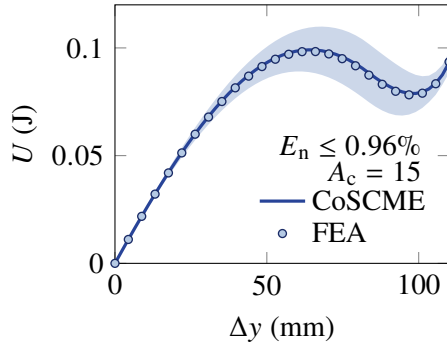
Fig. 4.7.: Modeling results for the classical translational bistable mechanism. Results are verified by FEA simulations. (a) Coordinate systems and terminology used for modeling the classical translational bistable mechanism: Parameters defined in the global coordinate system ( O - xy ) include the displacement exerted on the center shuttle, denoted as \Delta y , and the reaction forces in the global coordinate system, denoted as F_x and F_y . Parameters defined in the local coordinate system ( O_L - x_L y_L ) include the reaction forces, denoted as f_x and f_y . (b) The force-displacement relationship of the translational bistable mechanism. The figure on the right zooms in on the results, providing more details around the critical buckling point. (c) Energy-displacement curve for translational bistable mechanism. (d) Maximum stress during deformation obtained from both CoSCME and FEA simulation.
