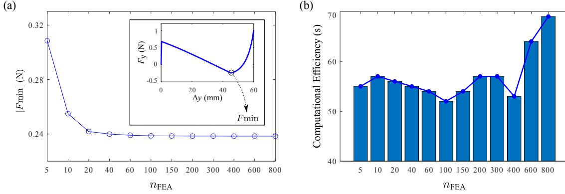
Fig. 3.4.: Convergence analysis of FEA simulation via modeling compliant beams with varying numbers of beam elements. The amount of beam elements varies from 5 to 800. (a) The local minima of the force-displacement curve ( F_{\min} ) obtained from FEA simulations against distinct beam elements. The convergence of the simulation is evaluated by examining whether the magnitude of F_{\min} converges. (b) Computational efficiency comparison, which is measured in seconds.
