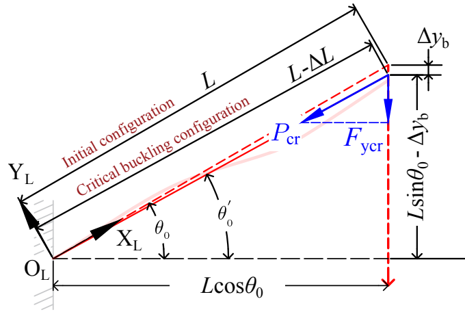
Fig. 3.6.: The variables and geometrical parameters defined to derive the critical buckling position and force. The initial configuration of the beam is represented using the red dashed line. The critical buckling configuration is represented using the red continuous line. The buckled configuration of the beam line is represented using a half-transparent red continuous line.
