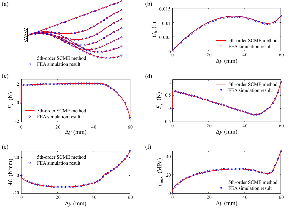
Fig. 3.5.: The modeling result comparisons between 5th-order SCME method and FEA simulation result. The parameters used in modeling and simulation are: L=100\text{mm} , \theta=20^\circ , E=2800\text{ MPa} , W=10\text{mm} , T=0.6\text{mm} . (a) Comparison of deformation shape. (b) Comparison of bending strain energy U_b . (c) Comparison of F_x . (d) Comparison of F_y . (e) Comparison of M_t . (f) Comparison of maximum stress \sigma_{\max} .
