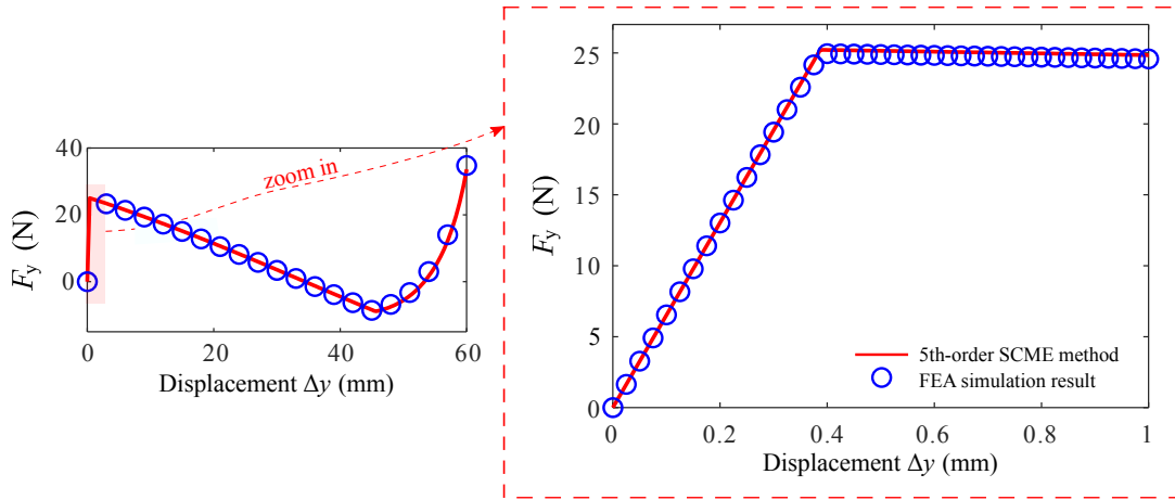
Fig. 3.7.: Comparison between the modeling result considering linear compensation and FEA simulation. The overall force-displacement curve is displayed on the left, while the displacement range [0,1] is zoomed in to provide a clearer visualization of the linear deformation compensation result, as demonstrated on the right.
