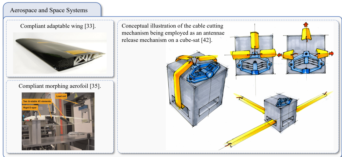
Fig. 1.4.: Representative applications of compliant mechanisms in aerospace and space systems.
