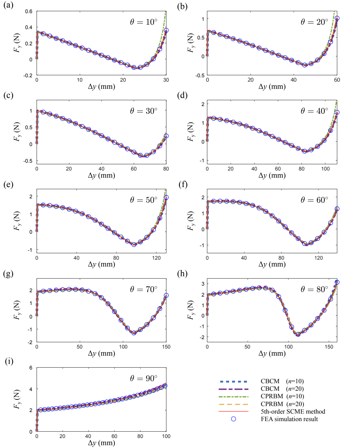
Fig. 3.13.: Force-displacement relationship comparison between 5th-order SCME method, CBCM, CPRBM, and FEA simulation. Ten and twenty beam elements are used in CBCM and CPRBM. The parameters used in modeling and simulation are: L=100\text{mm} , E=2800\text{ MPa} , W=10\text{mm} , T=0.6\text{mm} . (a) \theta = 10^\circ . (b) \theta = 20^\circ . (c) \theta = 30^\circ . (d) \theta = 40^\circ . (e) \theta = 50^\circ . (f) \theta = 60^\circ . (g) \theta = 70^\circ . (h) \theta = 80^\circ . (i) \theta = 90^\circ .
