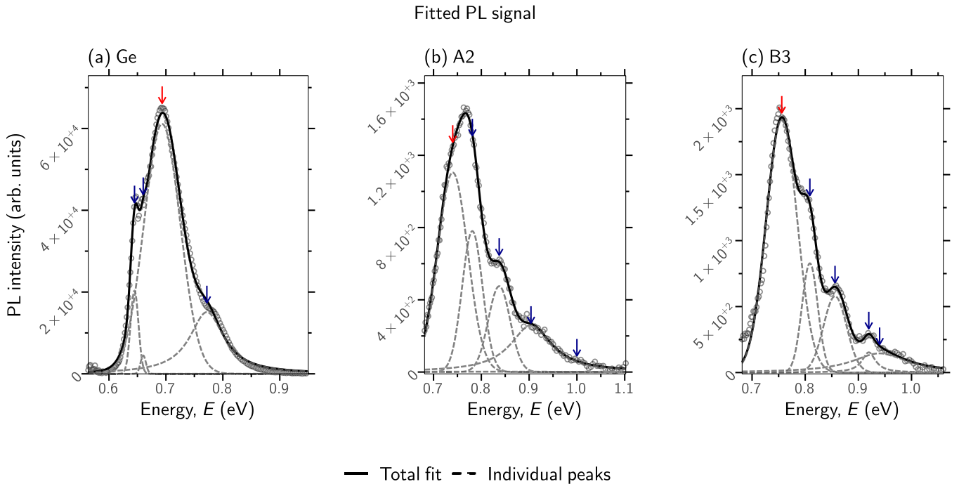
FIG. 7. Illustration of the fits to the PL data at low power using Gaussian and Lorentzian line shapes. The total fit to the data and individual peaks are shown for (a) the Ge reference sample, (b) sample A2, and (c) the thicker B3 sample. The arrows indicate the individual peak locations; the red arrow in each case indicates the peak with the highest intensity, which was taken to correspond to LA phonon absorption by analogy with the PL spectrum of Ge.
