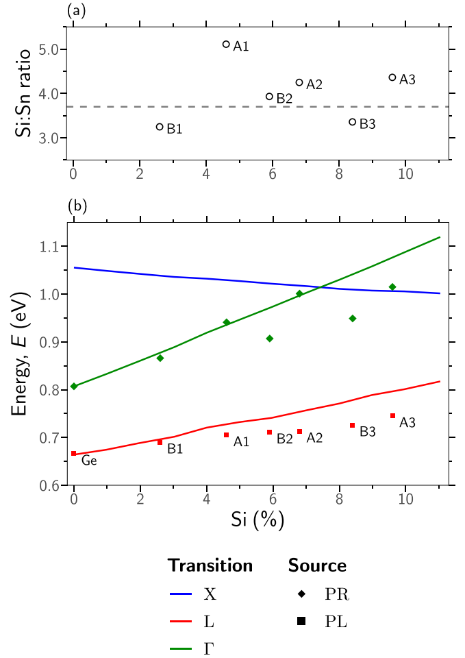
FIG. 8. (a) SEM-EDX measured Si to Sn composition ratios x:y for the samples investigated (cf. Table I). (b) Comparison of the transition energies extracted from experimental measurements (points) and calculated using TB method (lines), showing data for the indirect band gap from PL measurements (red squares), and for the direct transition from PR measurements (green diamonds). The theoretical results are the calculated weighted average direct \Gamma_{7c}-\Gamma_{8v} (green), and indirect L_{6c}-\Gamma_{8v} (red) and X_{5c}-\Gamma_{8v} (blue) transition energies.
