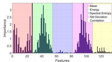
Fig. 7: Features Importance
