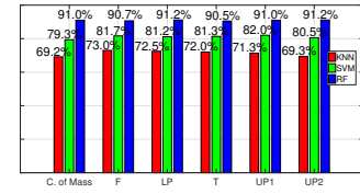
Fig. 3: Accuracies Comparison - Full Dataset
