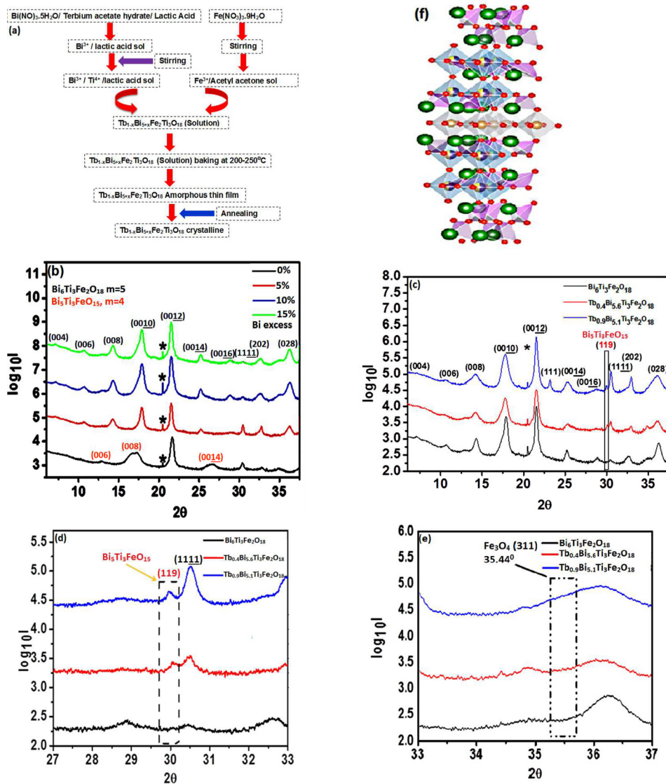
FIG. 1. (a) Chemical solution deposition (CSD) flow sheet demonstrating the synthesis of \text{Tb}_{1-x}\text{Bi}_{5+x}\text{Fe}_2\text{Ti}_3\text{O}_{18} thin films; X-Ray diffraction (XRD) patterns (b) illustrating the possible % (0%, 5%, 10%, and 15%) of Bi excess required to synthesize single phase \text{Bi}_6\text{Fe}_2\text{Ti}_3\text{O}_{18} (it should be noted that these samples were annealed for 30 min at 850 °C); (c) the diffraction patterns from \text{Bi}_6\text{Fe}_2\text{Ti}_3\text{O}_{18} , \text{Tb}_{0.40}\text{Bi}_{5.6}\text{Fe}_2\text{Ti}_3\text{O}_{18} , and \text{Tb}_{0.9}\text{Bi}_{5.1}\text{Fe}_2\text{Ti}_6\text{O}_{18} thin films on sapphire substrates (10% excess bismuth was used during the synthetic process); (d) restricted range slow speed scans through the 2-theta region which would be expected to reveal the appearance of secondary \text{Bi}_5\text{FeTi}_3\text{O}_{15} phase (119) reflection on increase in Tb substitution; (e) the presence of the ferromagnetic spinel impurity phases \text{Fe}_3\text{O}_4 or \text{TbFe}_2\text{O}_4 , if present in \text{Bi}_6\text{Fe}_2\text{Ti}_3\text{O}_{18} , \text{Tb}_{0.40}\text{Bi}_{5.6}\text{Fe}_2\text{Ti}_3\text{O}_{18} , and \text{Tb}_{0.9}\text{Bi}_{5.1}\text{Fe}_2\text{Ti}_6\text{O}_{18} thin films; (f) the crystal structure of the m = 5 Aurivillius phase \text{Tb}_{1-x}\text{Bi}_{5+x}\text{Fe}_2\text{Ti}_3\text{O}_{18} along the <110> direction with five perovskite units sandwiched between two bismuth oxide blocks.
