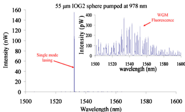
FIG. 4. (Color online) Single mode lasing at 1532 nm from a 55 \mu\text{m} IOG-2 microsphere pumped at 978 nm. Typical observed lasing thresholds are \sim 100 \mu\text{W} . Inset: WGM fluorescence from the same microsphere.
