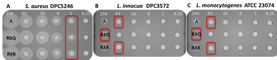
Figure 6. Activity ( \mu\text{M} ) of bacteriocin A (A) bacteriocin R8Q (plantaricin ST 1) and bacteriocin R8K against S. aureus DPC5246 (A) L. innocua DPC3572 (B) and L. monocytogenes ATCC 23074 (C).
