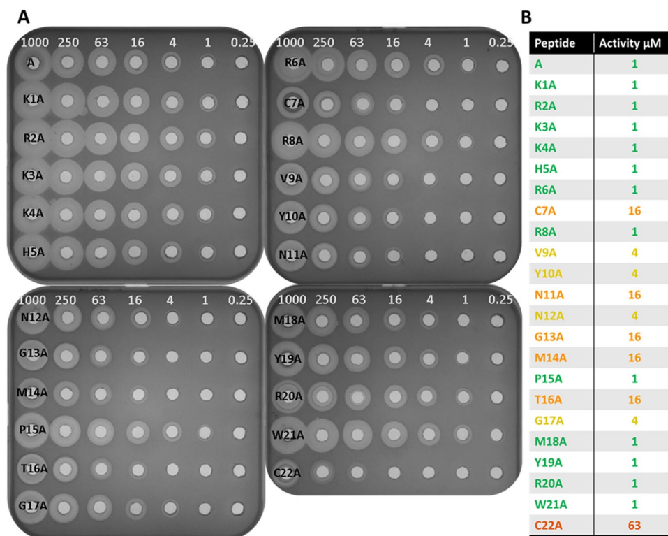
Figure 4. (A) Serial dilutions of each alanine variant plated on S. aureus DPC5246 indicator plates and (B) shows activity ( \mu\text{M} ) of bactofencin alanine variants against S. aureus DPC5246. Activity is colour coded with green being most active and red least active.
