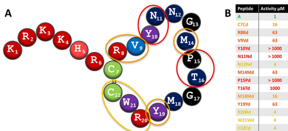
Figure 5. Activity ( \mu\text{M} ) of bactofencin D-variants C7Cd-C22Cd against S. aureus DPC5246. Activity is colour coded with green being most active and red inactive. Amino acids most affected by D-substitution are circled in (A) and activities presented in (B).
