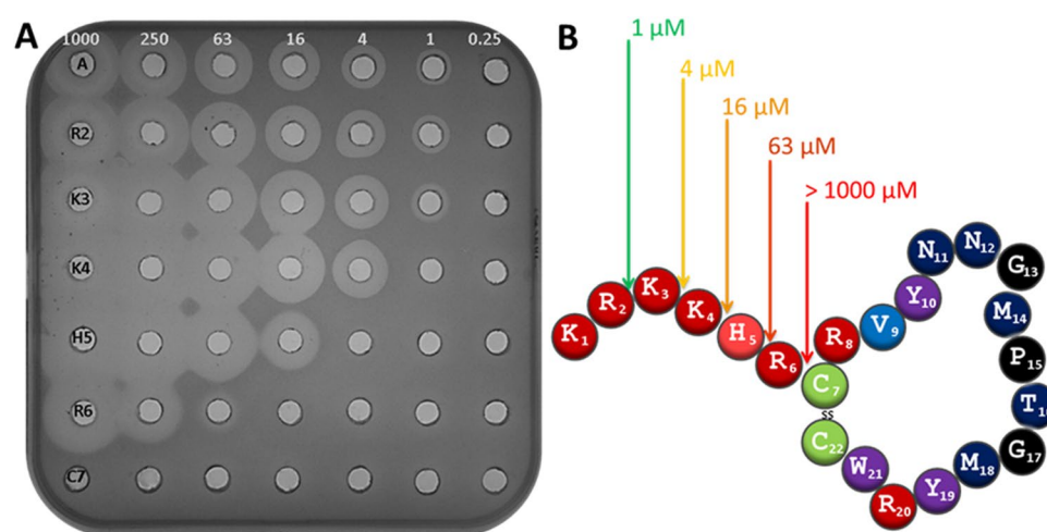
Figure 3. (A) Activity ( \mu\text{M} ) of bactofencin A and deletion variants, R2-C22, K3-C22, K4-C22, H5-C22, R6-C22 and C7-C22 against S. aureus DPC5246. (B) Activity ( \mu\text{M} ) of bactofencin A and deletion variants against S. aureus DPC5246. Activity is colour coded with green being most active and red inactive.
