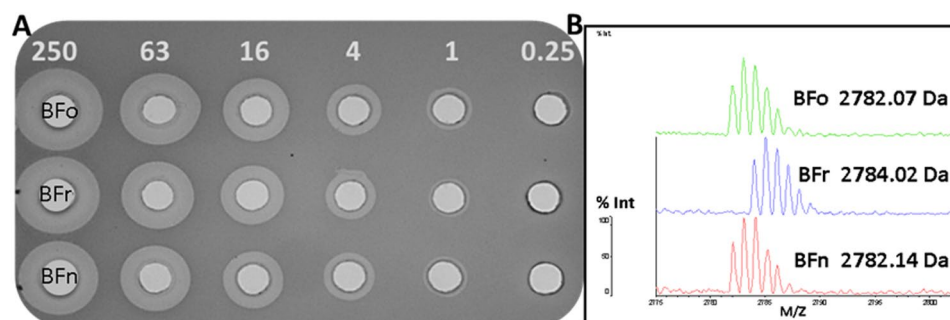
Figure 1. Activity ( \mu\text{M} ) of oxidized synthetic bactofencin A (BFo), reduced bactofencin A (BFr) and natural bactofencin A (BFN) against S. aureus DPC5246 (A) and molecular mass of oxidized synthetic bactofencin A (Top), reduced bactofencin A (Middle) and natural bactofencin A (Bottom) (B).
