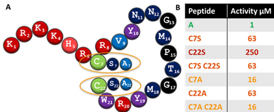
Figure 2. (A) Cys7 and Cys22 were substituted individually and in tandem with serine and alanine to give bactofencin variants C7S, C22S, C7S-C22S, C7A, C22A, C7A-C22A. Activity ( \mu\text{M} ) of bactofencin A compared to bactofencin cysteine variants C7S, C22S, C7S-C22S, C7A, C22A and C7A-C22A is presented in (B).
