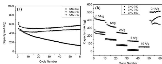
Figure 14 (a) Cycling performance of CNCs. Increasing temperature results in higher graphitisation and improved cycling and (b) rate performance of the CNCs at current densities ranging from 0.1–10 A g -1 [160]. Adapted with permission of The Royal Society of Chemistry.
