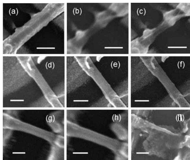
Figure 21 SEM images of single nanorod devices of (a-c) \text{LiMn}_2\text{O}_4 after 3, 6 and 9 h respectively, (d-f) \text{LiAl}_{0.1}\text{Mn}_{1.9}\text{O}_4 and (g-i) \lambda\text{-MnO}_2 after the same exposure times. Reprinted with permission from [270]. Copyright 2009 American Chemical Society.
