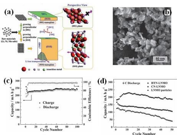
Figure 25 (a) Illustrative representation of the synthesis of (001) and (010) dominant \text{Li}[\text{Li}_{0.17}\text{Ni}_{0.25}\text{Mn}_{0.58}]\text{O}_2 nanoplates, (b) SEM image of the (010) nanoplates, (c) cycling and Coulombic efficiency studies of (010) nanoplates at a current density of 60 \text{ mA g}^{-1} between 2.0 – 4.8 V and (d) cycling of (010)-nanoplates (HTN-LNMO), (001)-nanoplates (CN-LMNO) and LNMO particles at 6 C rate. Adapted from [314]. Copyright Wiley-VCH Verlag GmbH & Co. KGaA. Reproduced with permission.
