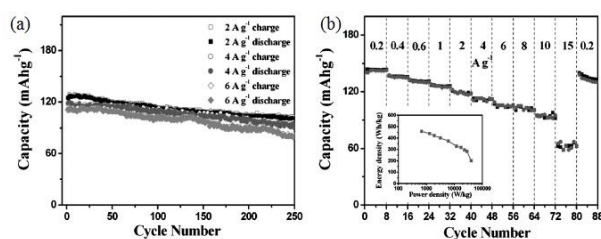
Figure 28 Electrochemical performance of the porous V_2O_5 nanotubes showing (a) discharge capacity as a function of cycle number and (b) rate performance over current densities 0.2 – 15 – 0.2 A\ g^{-1} . Adapted from [331]. Copyright Wiley-VCH Verlag GmbH & Co. KGaA. Reproduced with permission
