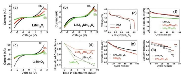
Figure 22. I-V curves of (a) LiMn 2 O 4 , (b) LiAl 0.1 Mn 1.9 O 4 , (c) \lambda -MnO 2 and (d) normalised conductance as a function of exposure time in LiPF 6 electrolyte. (e) First discharge plot of LiMn 2 O 4 and LiAl 0.1 Mn 1.9 O 4 cells at a rate of C/5, (f) cycling of LiMn 2 O 4 , LiAl 0.1 Mn 1.9 O 4 and \lambda -MnO 2 at a rate of C/5 at room temperature and (g) 60 °C. (h) Rate-performance of the LiMn 2 O 4 and LiAl 0.1 Mn 1.9 O 4 cells at room temperature. Reprinted with permission from [270]. Copyright 2009 American Chemical Society.
