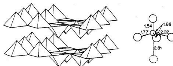
Figure 26 Structure of layered \text{V}_2\text{O}_5 (left) depicting square pyramidal \text{VO}_5 units which share both corner and edges and the
