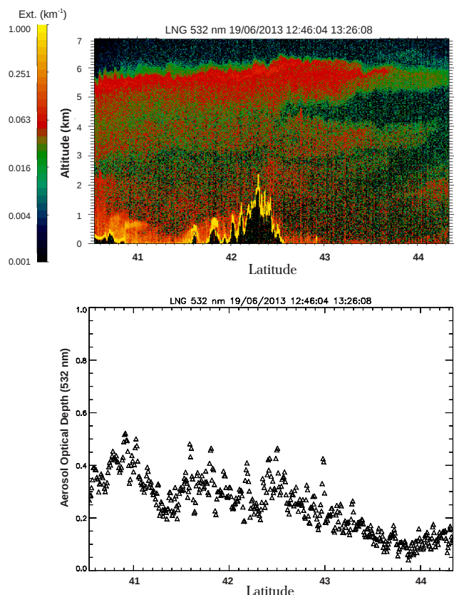
Figure 24. Observations of aerosol extinction coefficient (top, in \text{km}^{-1} at 532 nm) and aerosol optical depth (bottom) obtained from the lidar LNG system onboard the F-20 aircraft during 19 June that corresponds to the flight (12:46 to 13:26) from Cagliari to the Gulf of Genoa.
