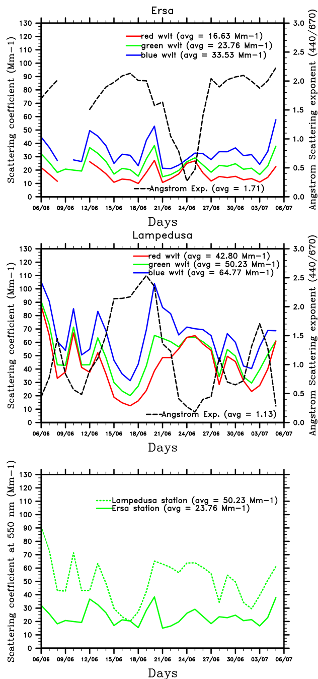
Figure 18. Time series of the daily scattering coefficient (in Mm -1 ) estimated at the Ersa and Lampedusa stations. The daily Angström exponent (AE), calculated between 440 and 670 nm, is also reported.
