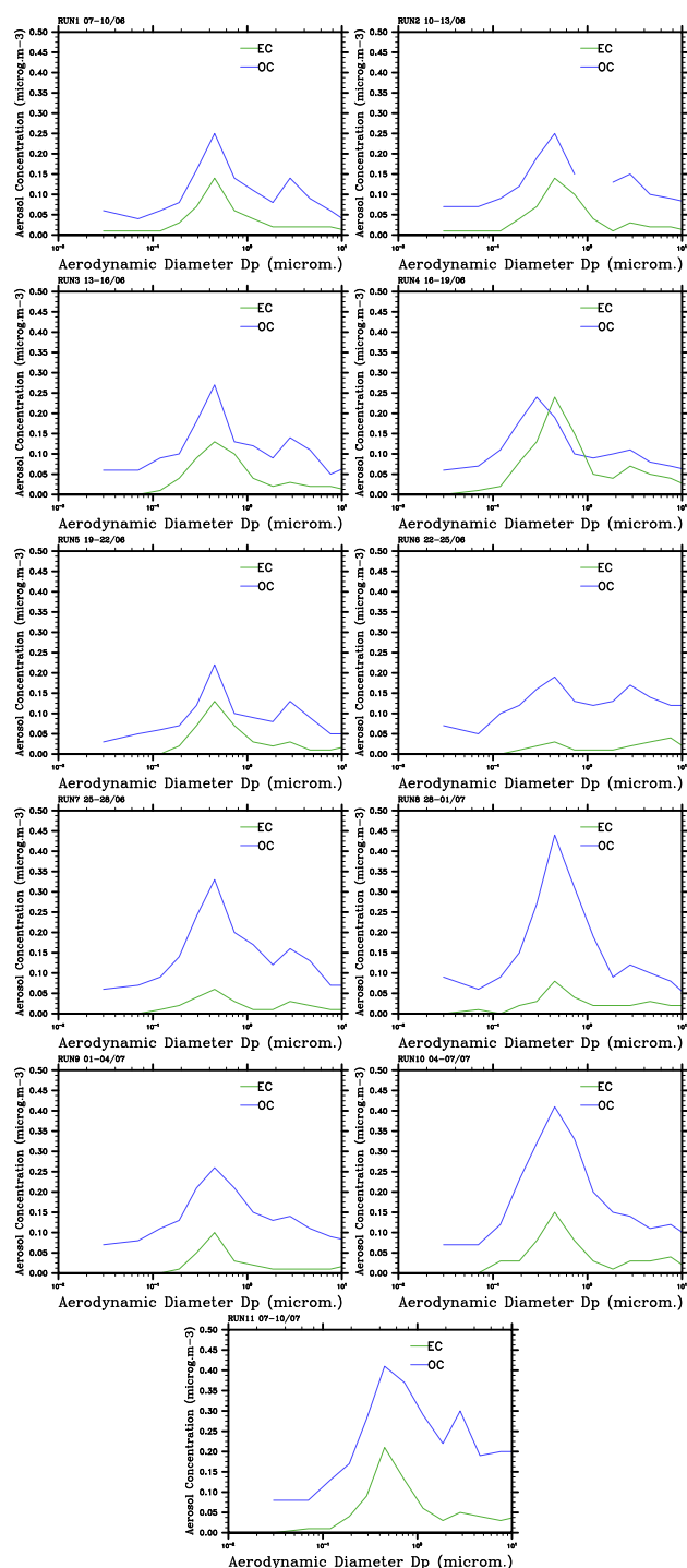
Figure 16. EC and OC (48 h mean) aerosol mass size distributions obtained at Ersá from the DEKATI impactor instrument for the entire SOP-1a period.
