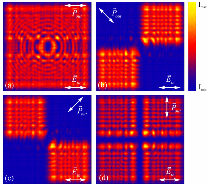
Fig. 3. Intensity distribution (negative) for a beam \vec{E}_{in} having passed through a micropolarizer, measured 5.1- \mu\text{m} away from the micropolarizer surface. The analyzer \vec{P}_{out} is rotated by 0° (a), -45° (b), 45° (c), and 90° (d) with respect to the polarization vector \vec{E}_{in} .
