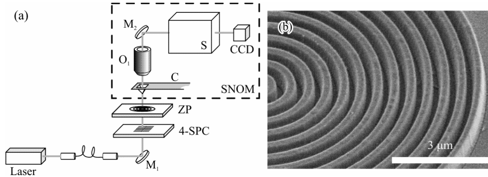
Fig. 9. Experimental optical arrangement (a): M_1 , M_2 are mirrors, O_1 is a 100\times objective, C is a probe, S is a spectrometer, and CCD is a video-camera. SEM image of ZP [13] (b).
