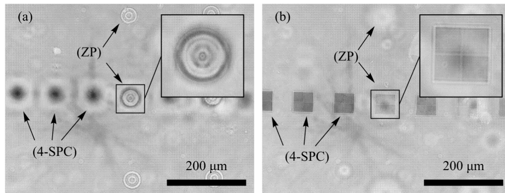
Fig. 10. An optical microscope 20x image of (a) a ZP on the 4-SPC background and (b) a 4-SPC on the ZP background. The inset shows magnified and aligned ZP and 4-SPC with their centers lying on the optical axis.
