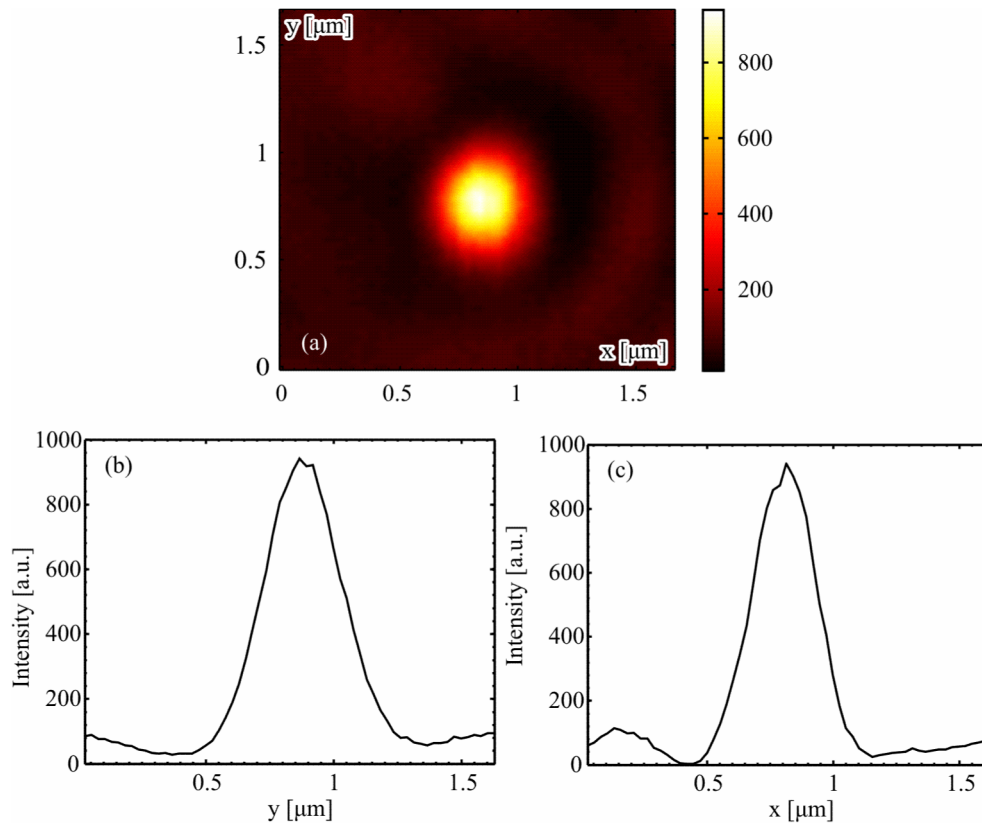
Fig. 12. Intensity profile of the focal spot measured using a NSOM Ntegra Spectra: 2D intensity distribution (a) and intensity profiles along the y- (b) and x-axis (c).
