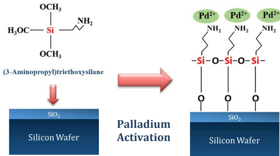
Fig. 3. Schematics of self-assembled monolayer deposition process and \text{Pd}^{2+} deposition as catalyst layer.
