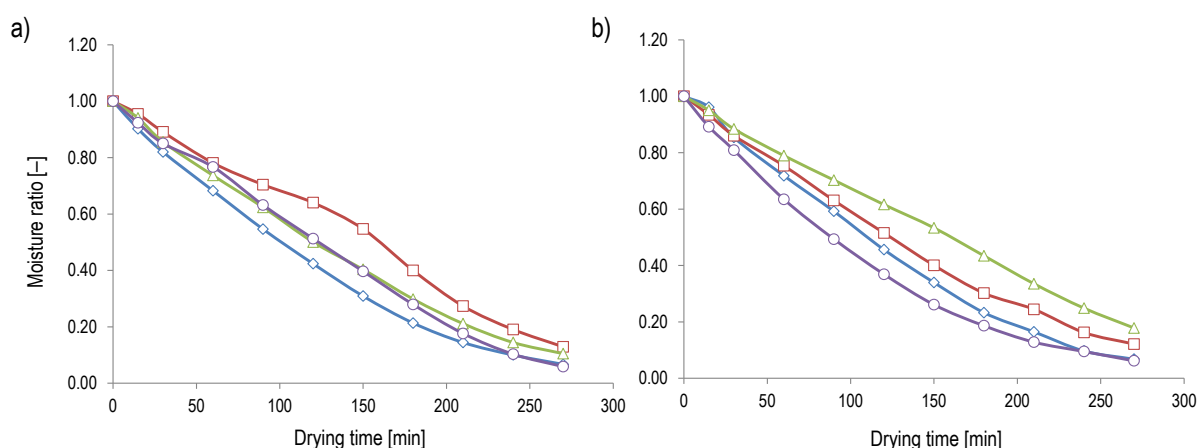
Figure 6.1. Moisture ratio [MR] vs. drying time [min] for a) uncultured and (b) cultured beef jerky slices pre-treated at various ultrasonic frequencies [Control ( \diamond ), 25 kHz ( \square ), 33 kHz ( \triangle ) and 45 kHz ( \circ ) respectively].
