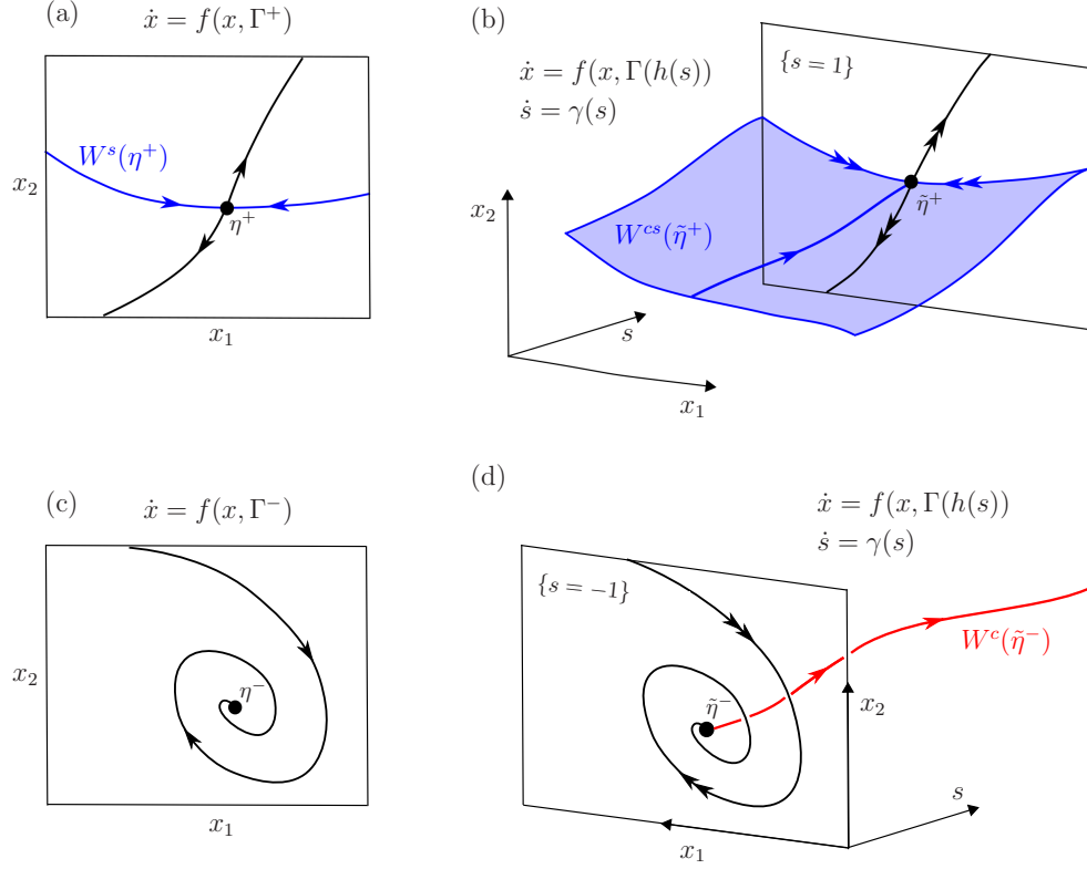
Figure 2.4: (a) A hyperbolic saddle \eta^+ for the future limit system (2.3) gains a neutrally stable center direction and becomes (b) a non-hyperbolic saddle \tilde{\eta}^+ = (\eta^+, 1) in the extended phase space of the compactified system (2.7)–(2.12). (c) A hyperbolic stable focus \eta^- for the past limit system (2.4) gains a neutrally unstable center direction and becomes (d) a non-hyperbolic saddle-focus \tilde{\eta}^- = (\eta^-, -1) with one-dimensional center manifold in the extended phase space of (2.7)–(2.12).
