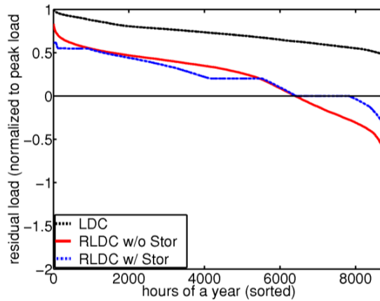
Figure 11: Effect of short-term storage deployment in DIMES on the RLDC for Europe with a gross contribution (gross meaning “before curtailments”) to a load of 30% from wind and 40% from PV. The LDC is displayed in black. Compared to the RLDC before use of short-term storage (red), the RLDC with storage (blue) shows much lower residual peak demand and less curtailment.
