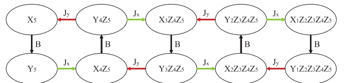
FIG. 1. (Color online) Oriented graph describing how the operators \hat{X}_5 and \hat{Y}_5 evolve in the Heisenberg picture. The operators within each circle (a node) give rise to their nearest neighbors on commutation with \hat{\mathcal{H}} in Eq. (1). The oriented edges connect such nodes. The corresponding coefficients are also shown and an outgoing (incoming) edge with respect to a node implies a + ( - ) sign. Black, light green, and dark red edges are associated respectively with B , J_x , and J_y interaction terms.
