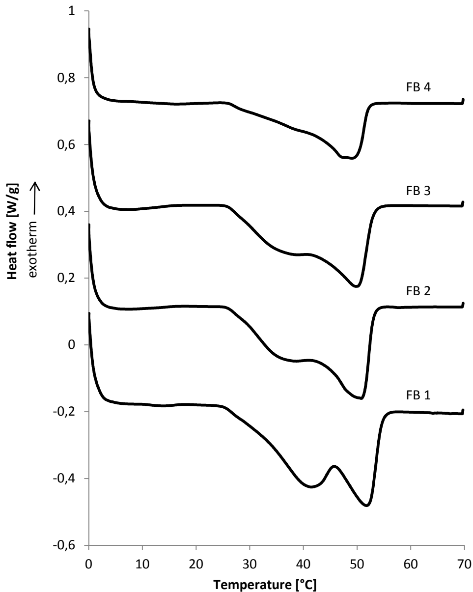
Figure 4-2 DSC melting curves of fat blends (FB) 1 to 4 at a heating rate of 5 °C/min
