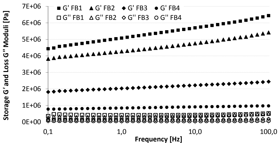
Figure 4-4 Storage ( G' ) and loss ( G'' ) moduli as a function of frequency of fat blends (FB) 1 to 4 at 25 °C and a constant strain of 5 \times 10^{-3} %. Values are means ( n = 3 )
