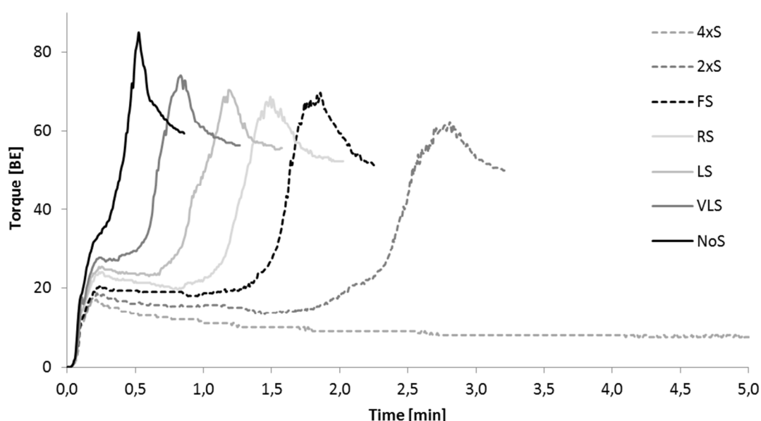
Figure 5-1 GlutoPeak curves of puff pastry basic dough with different salt levels: 4xS – fourfold salt, 2xS – twofold salt, FS – full salt, RS –reduced salt, LS – low salt, VLS – very low salt, NoS – no salt
