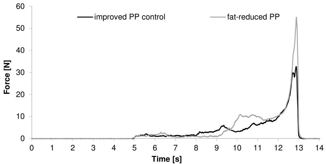
Figure 3-2 Force-time plot of 40 % fat-reduced puff pastry (48 layers, 2.25 mm) and improved puff pastry control (81 layers, 2.50 mm)
