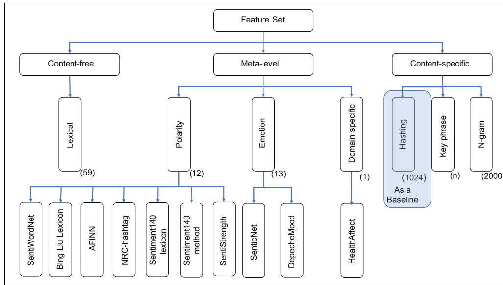
Figure 5.4: Feature set
