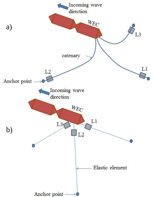
Figure 5. Schematically drawings of the mooring system for the test model, a) Catenary and b) taut arrangement; L1, L2 and L3: load cells
