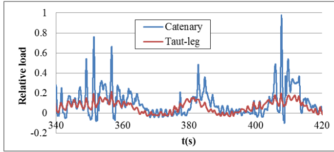
Figure 6. Loads on front anchor (normalised by the largest load on anchors)
