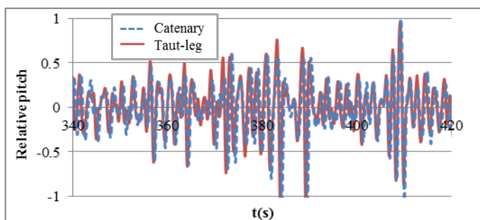
Figure 9. Pitch motion (normalised by the maximal significant height of pitch motion)
