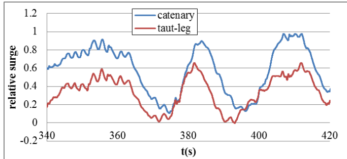
Figure 7. Surge motion (normalised by using the largest excursion)
