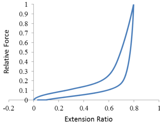
Figure 3. Seaflex elastic component Force – extension curve
