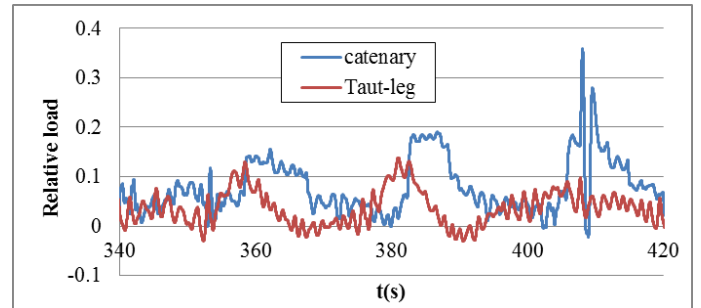
Figure 10. Loads on front anchor (normalised by the largest load on anchors)
