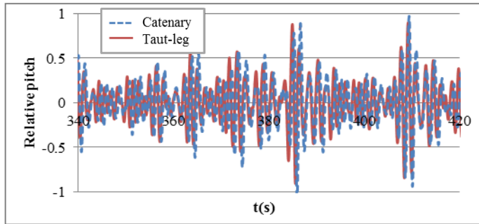
Figure 13. Pitch motion (normalised by the maximal significant height of pitch motion)
