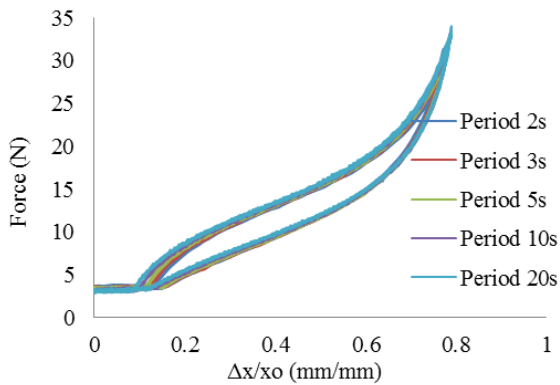
Figure 4. O-ring cord 3.5 mm test
