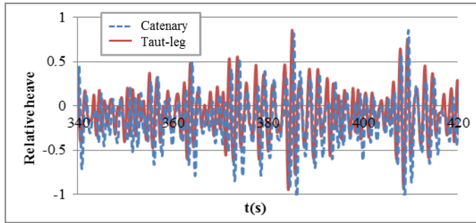
Figure 12. Heave motion (normalised by the maximal significant height of heave motion)
