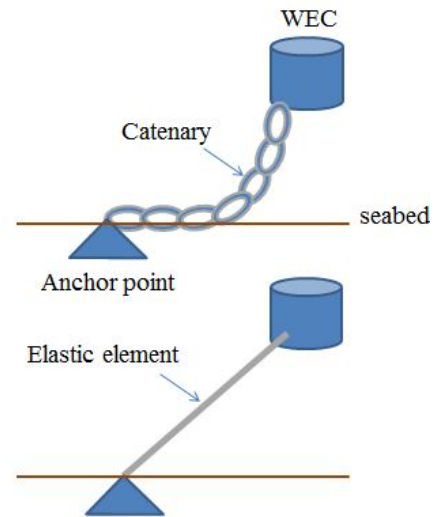
Figure 1. General principle of the catenary and elastic mooring line
