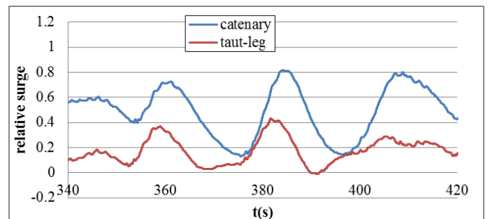
Figure 11. Surge motion (normalised by using the largest excursion)
