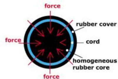
Figure 2. Cross-section of a Seaflex strand
