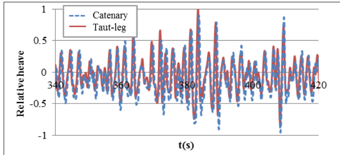
Figure 8. Heave motion (normalised by the maximal significant height of heave motion)
