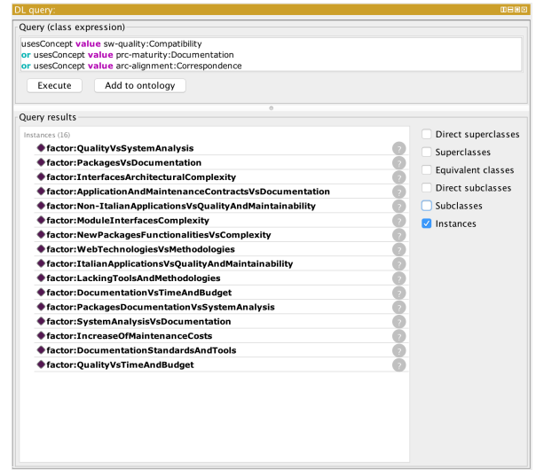
Fig. 4. Execution of a DL query on the RDF sample.
