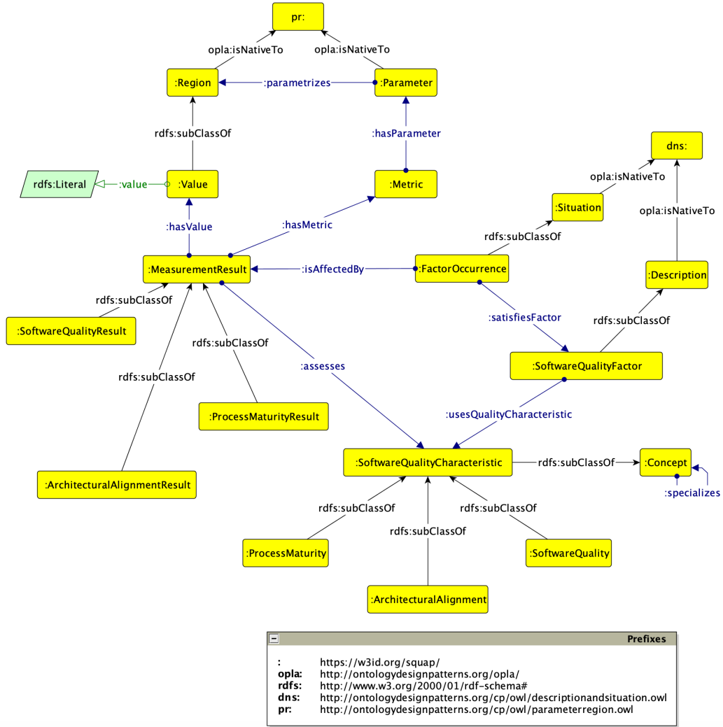
Fig. 3. Core classes of SQuAP-Ont.
