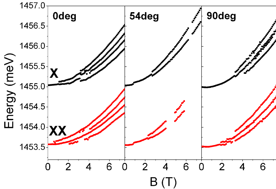
Figure 6.2-1. Evolution of LQD exciton and biexciton photoluminescence splitting in the magnetic field taken at different angles between magnetic field and growth direction ( 0^\circ , 54^\circ and 90^\circ ).
