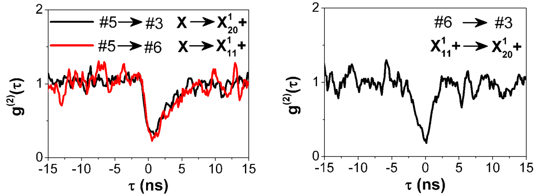
Figure 4.7-4. (a) The cross-correlations between transitions #5 and #3 (#6). (b) The cross-correlation between #6 and #3.
