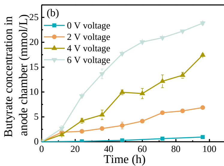
Fig. 2 Removal experiments of simulated fermentation broth. (a) Butyrate concentration in the fermentation chamber; (b) Butyrate concentration in the anode chamber.
